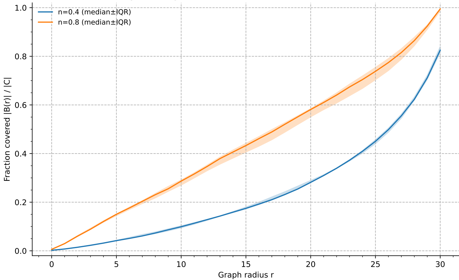
Fig. 5 Ball growth fraction (ensemble) ( W=100 , N=8 )
