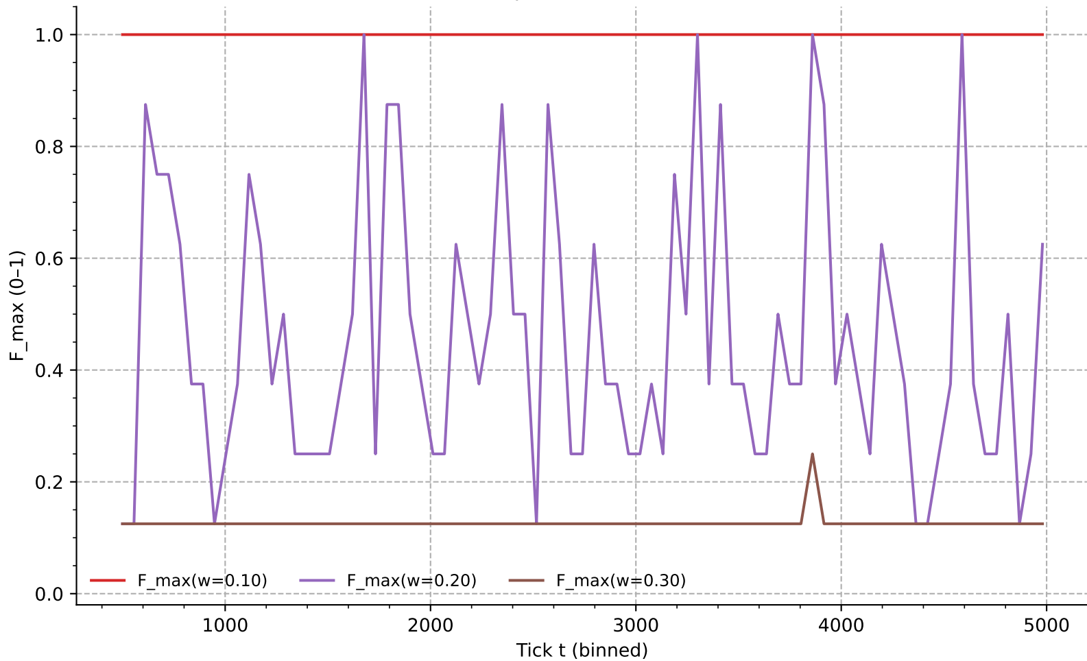
Island coherence over time (pilot: W=100 , N=8 , n=0.8 , seed=56796)
