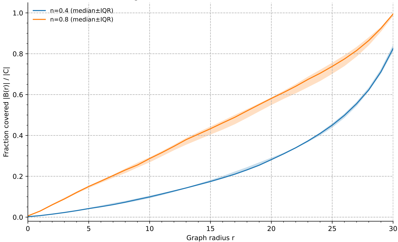
Ball growth fraction (ensemble) ( W=100 , N=8 )
