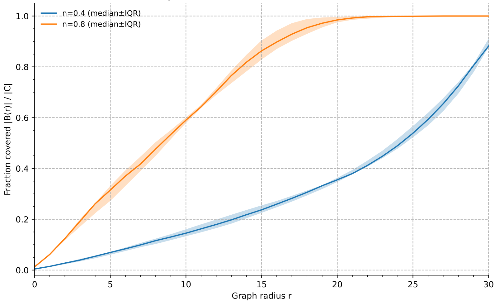
Ball growth fraction (ensemble) (W=100, N=4)
