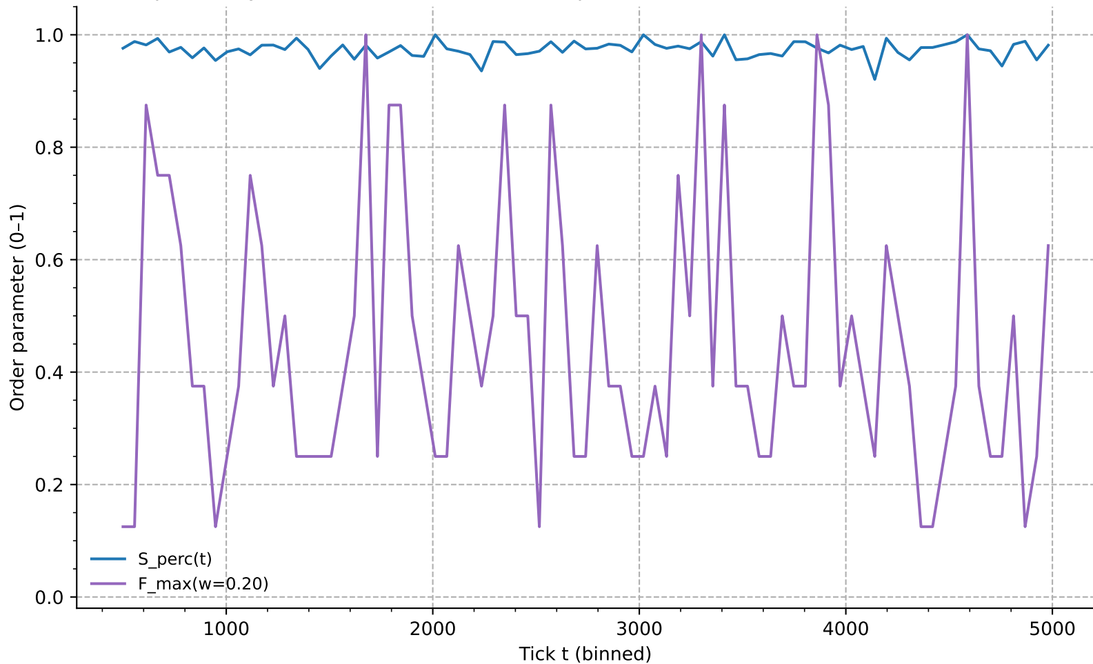
Space stays on while islands fluctuate (pilot: W=100 , N=8 , n=0.8 , seed=56796)
