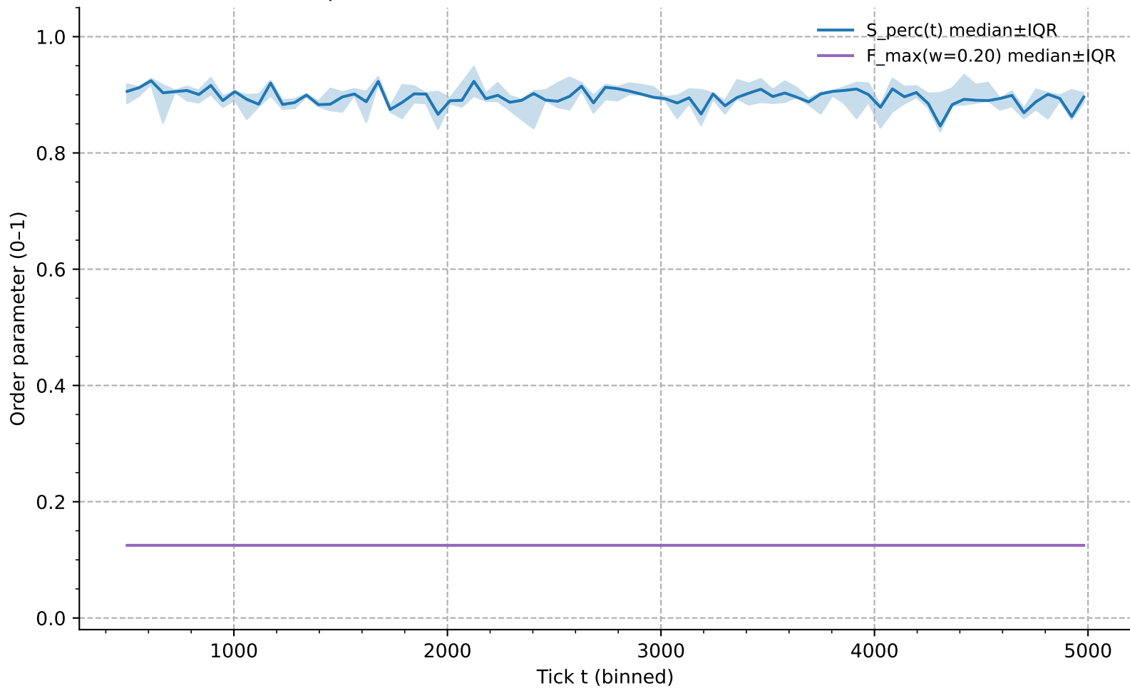
Space vs islands (ensemble) ( n=0.4 , W=100 , N=8 )
