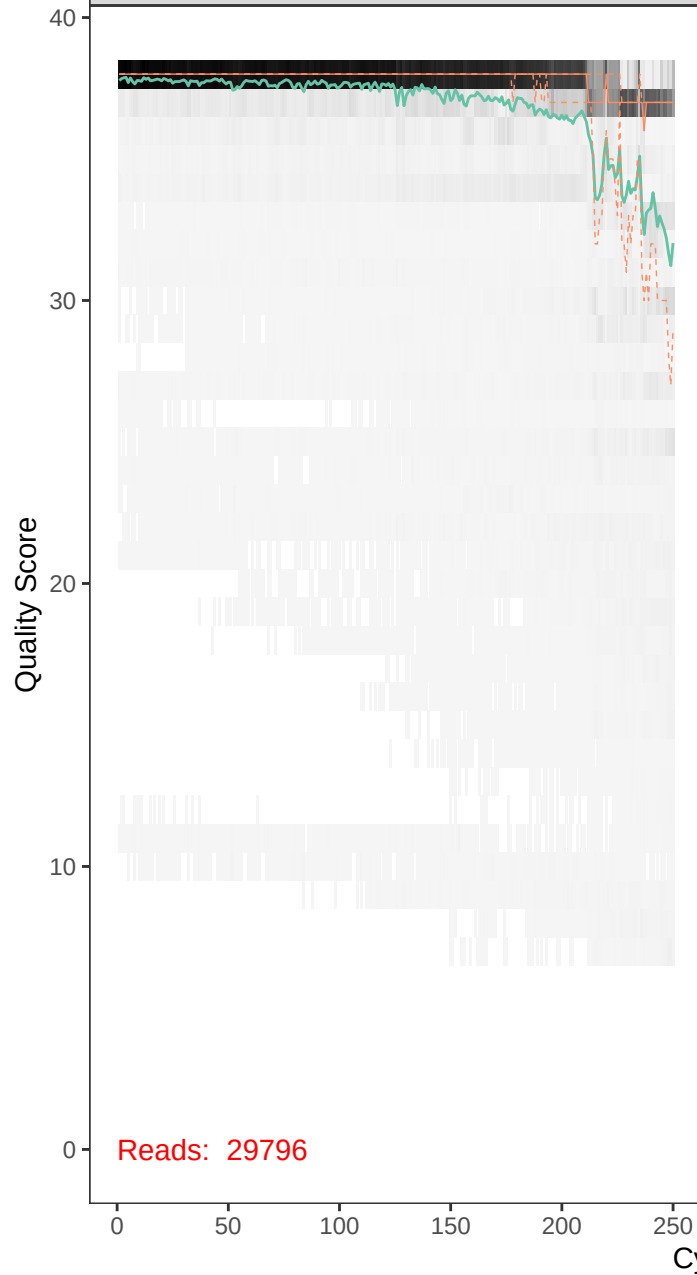
runBE08_F60R50-r1_F_filt.fastq
