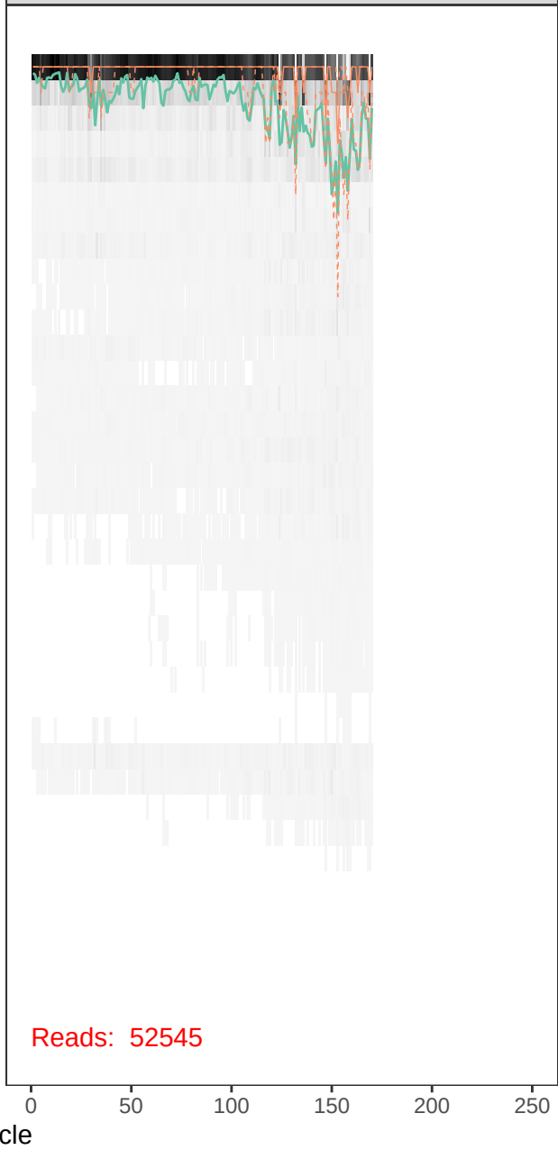
runBE05_FLD0364-r1_R_filt.fastq
