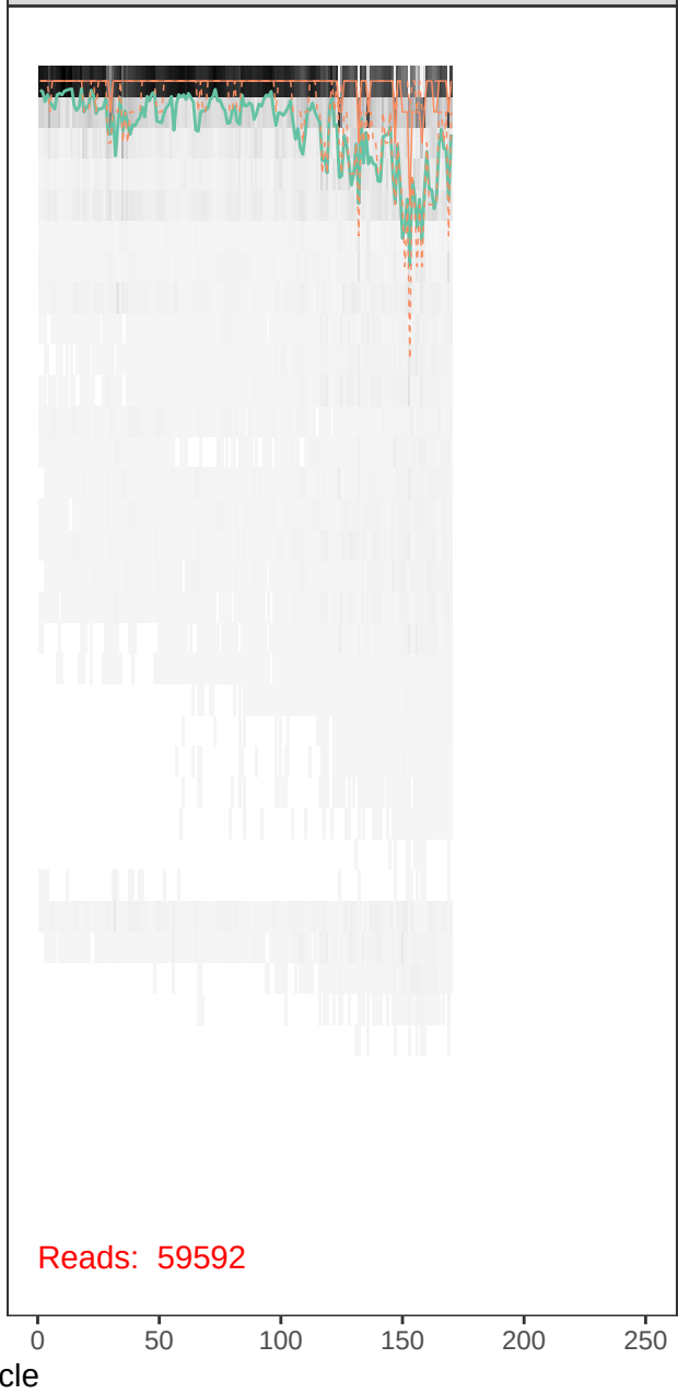
runBE05_FLD0055-r1_R_filt.fastq
