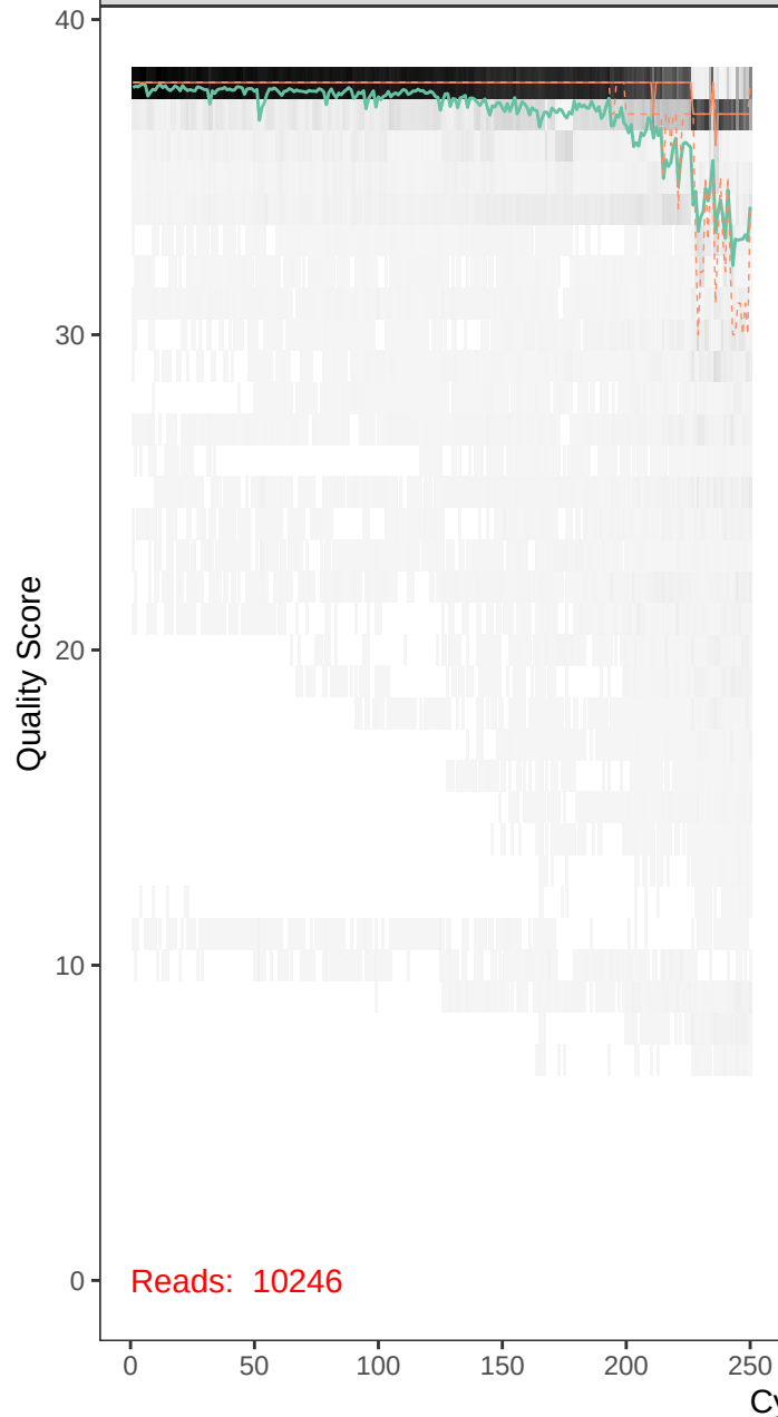
runBE08_F66R46-r1_F_filt.fastq
