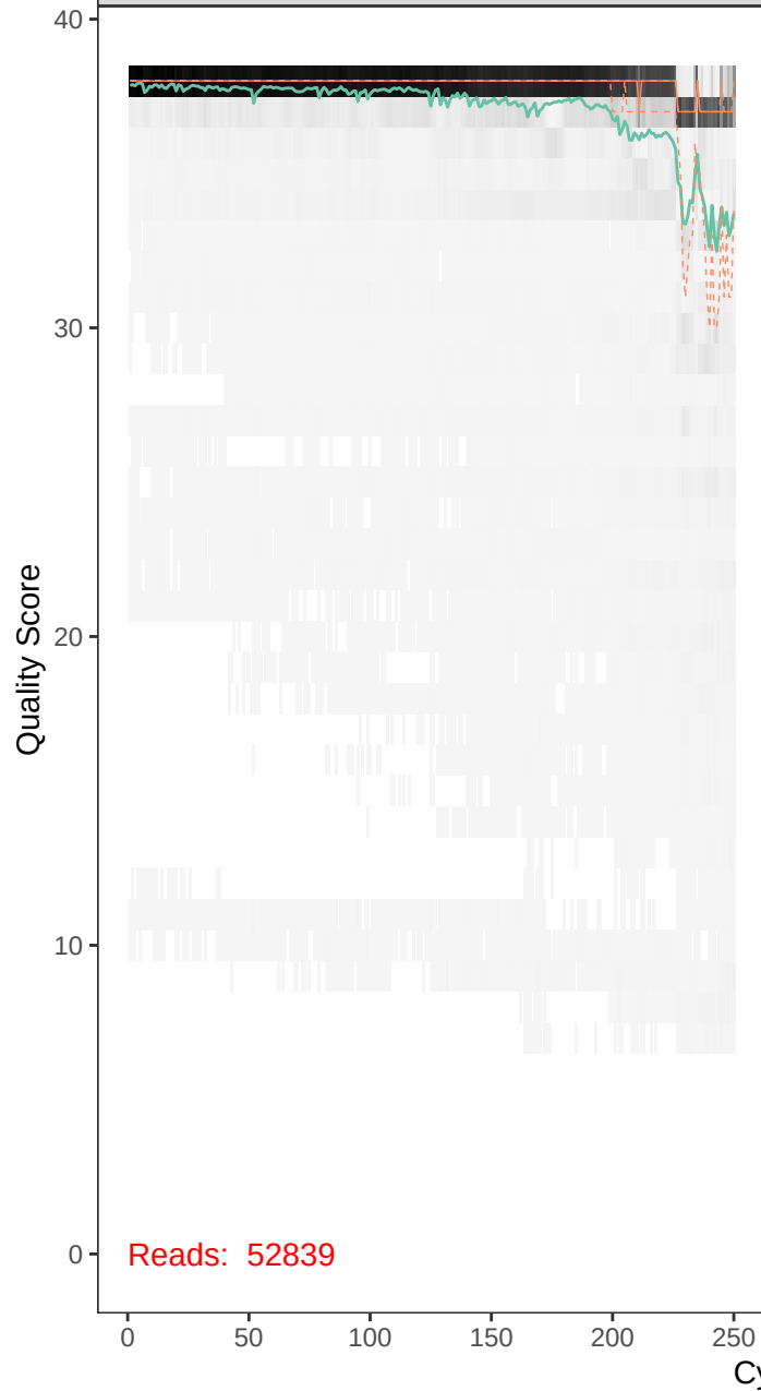
runBE08_F70R53-r1_F_filt.fastq
