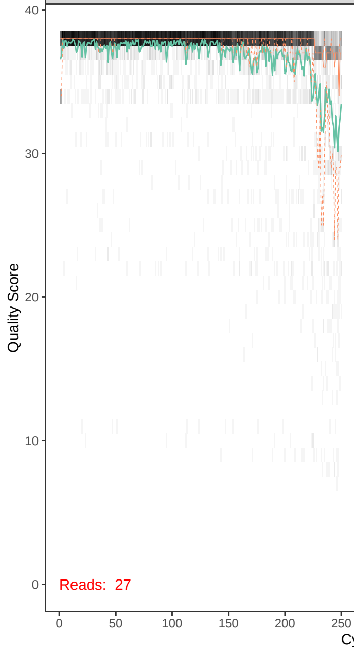
runBE08_F75R47-r1_F_filt.fastq
