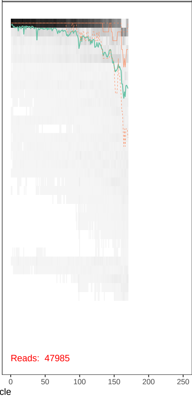
runBE08_F68R55-r1_R_filt.fastq
