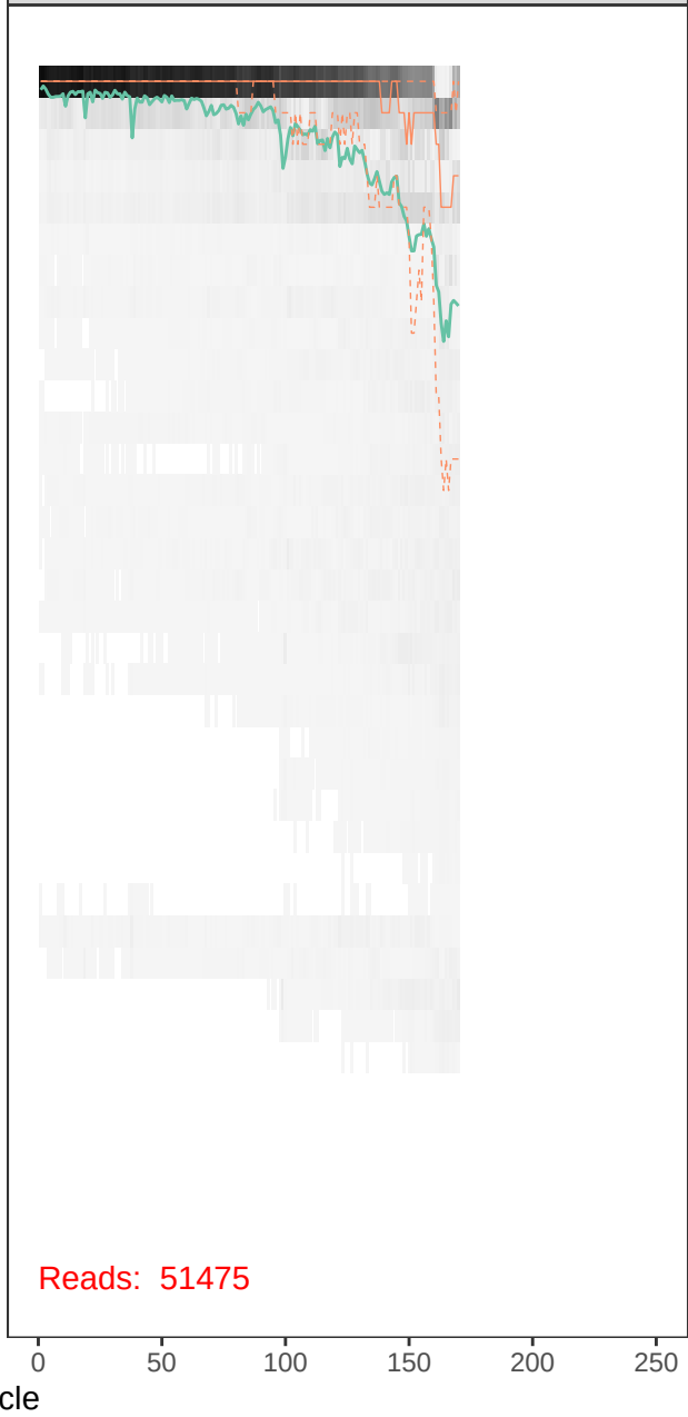
runBE08_F65R52-r1_R_filt.fastq
