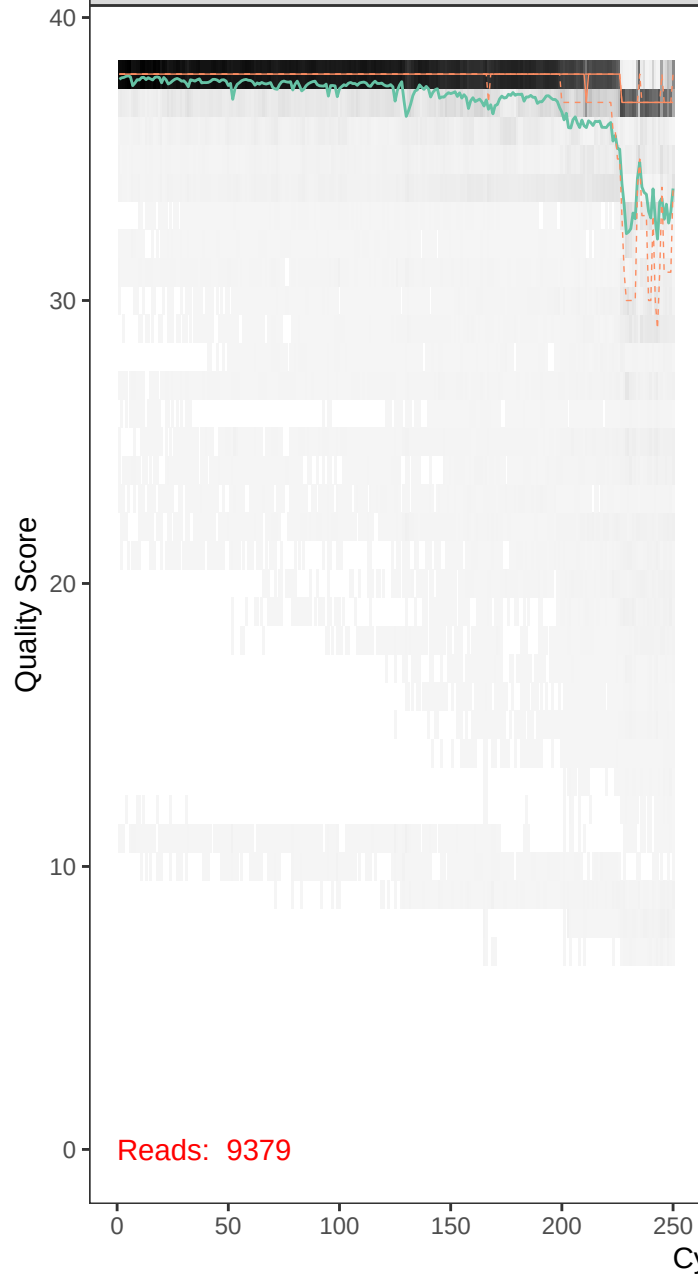
runBE08_F73R43-r1_F_filt.fastq
