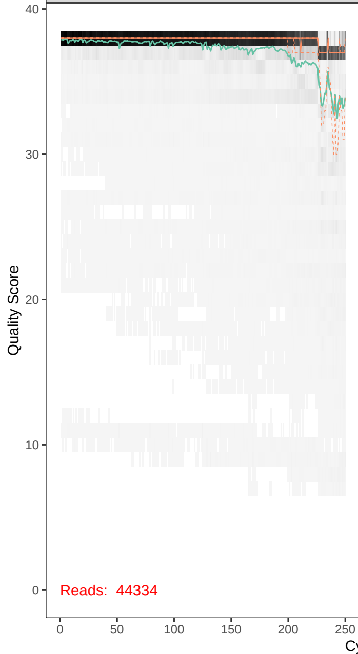
runBE08_F68R45-r1_F_filt.fastq
