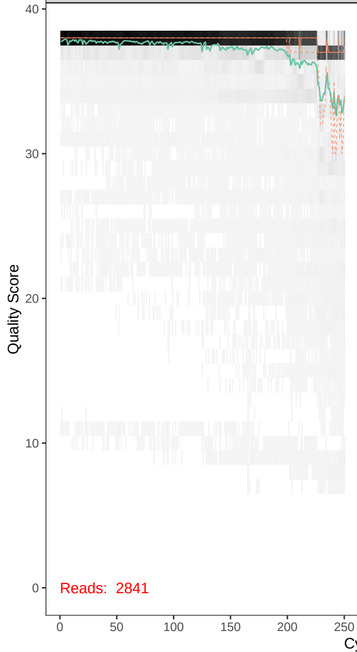
runBE08_F72R48-r1_F_filt.fastq
