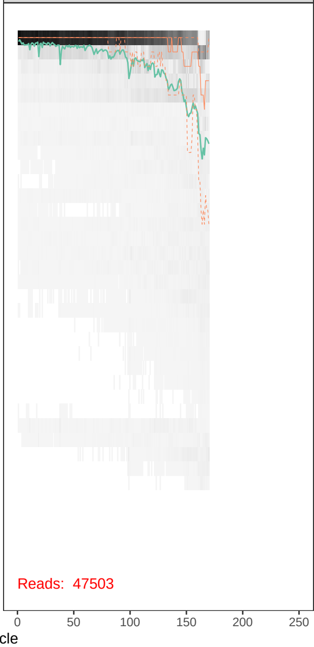
runBE08_F63R52-r1_R_filt.fastq
