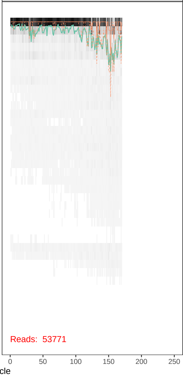
runBE05_FLD0003-r1_R_filt.fastq
