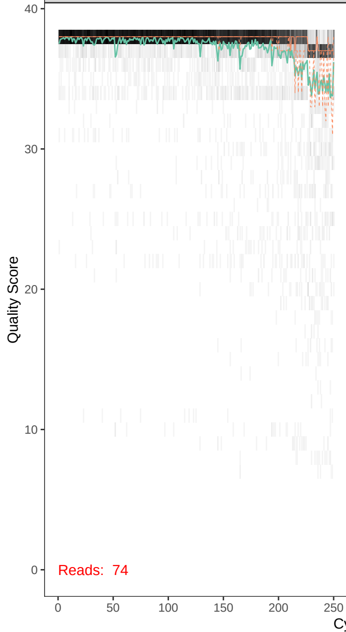
runBE08_F67R53-r1_F_filt.fastq
