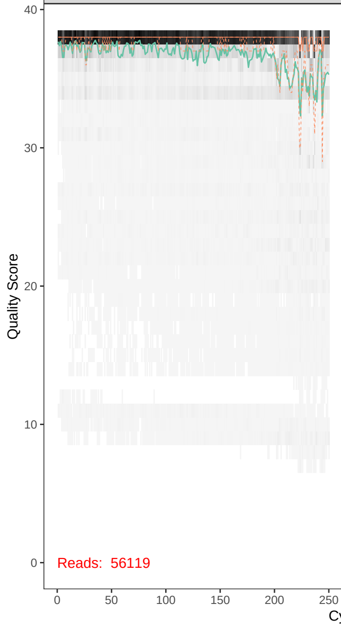
runBE05_FLD0064-r1_F_filt.fastq
