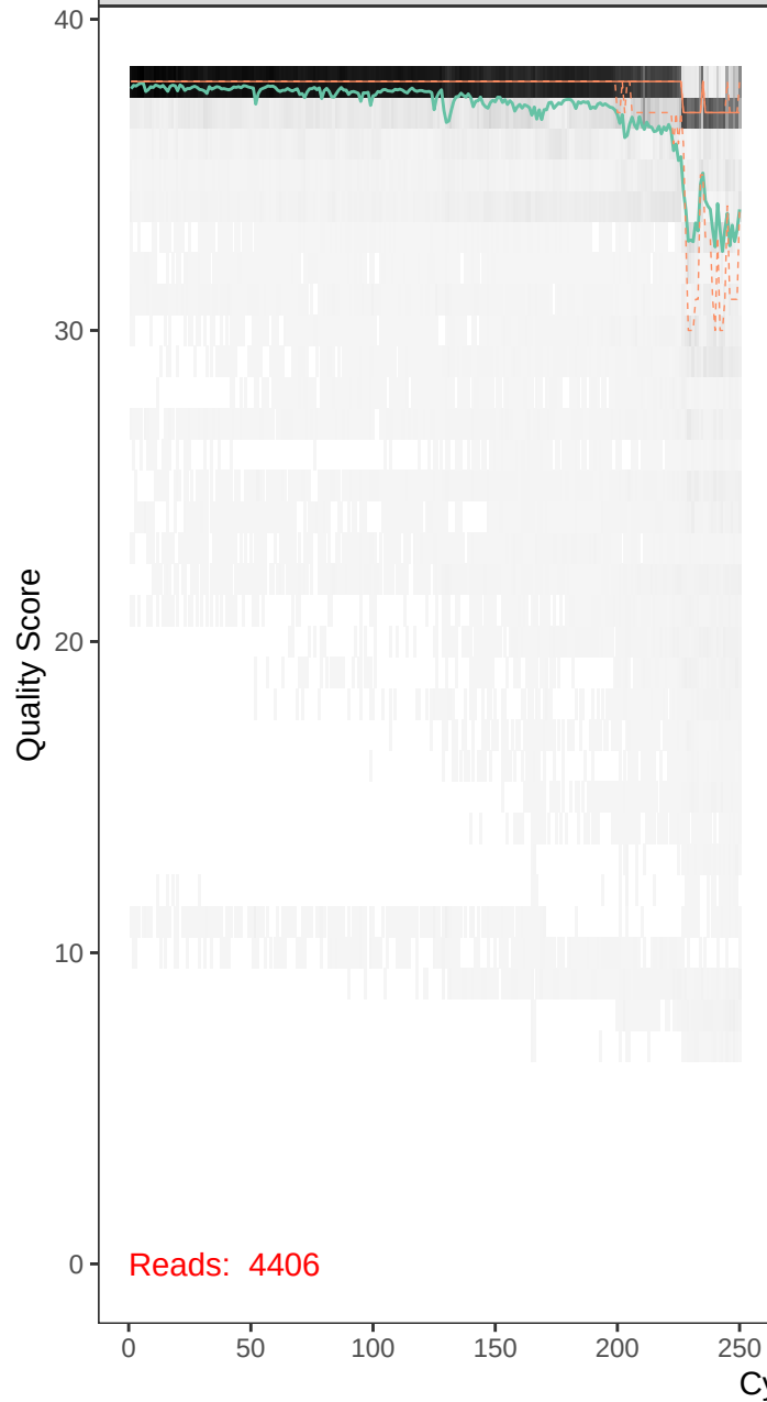
runBE08_F62R53-r1_F_filt.fastq
