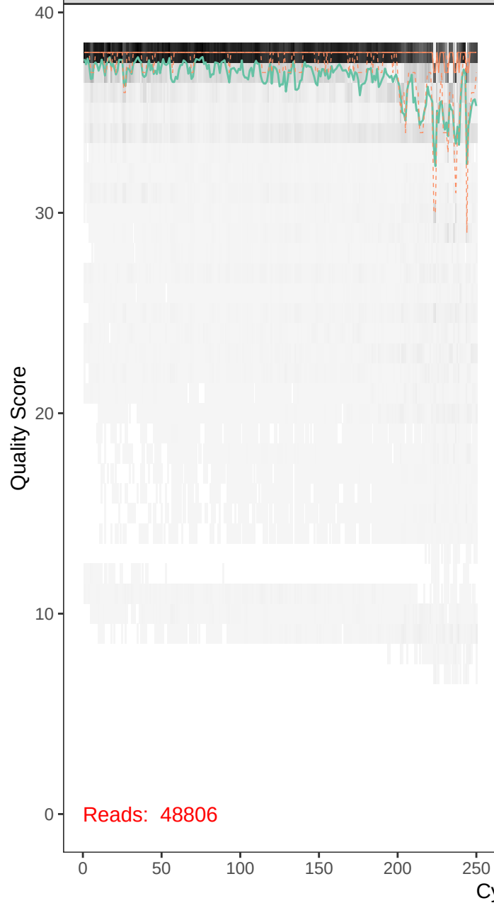
runBE05_FLD0079-r1_F_filt.fastq
