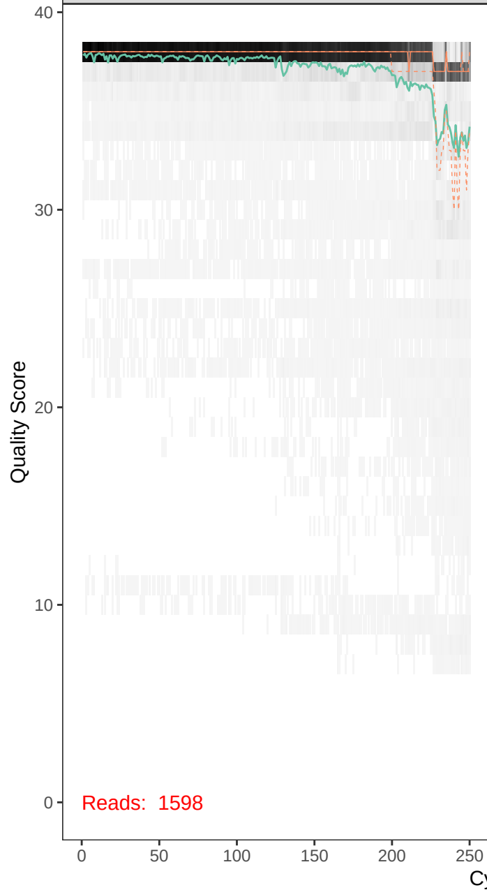
runBE08_F66R53-r1_F_filt.fastq
