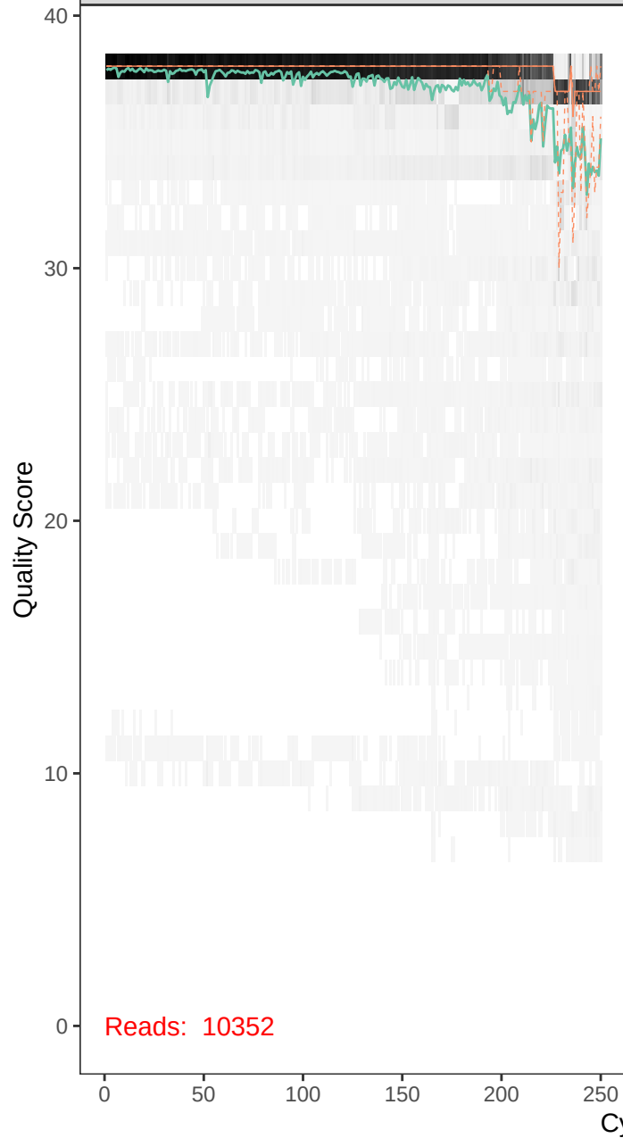
runBE08_F62R43-r1_F_filt.fastq
