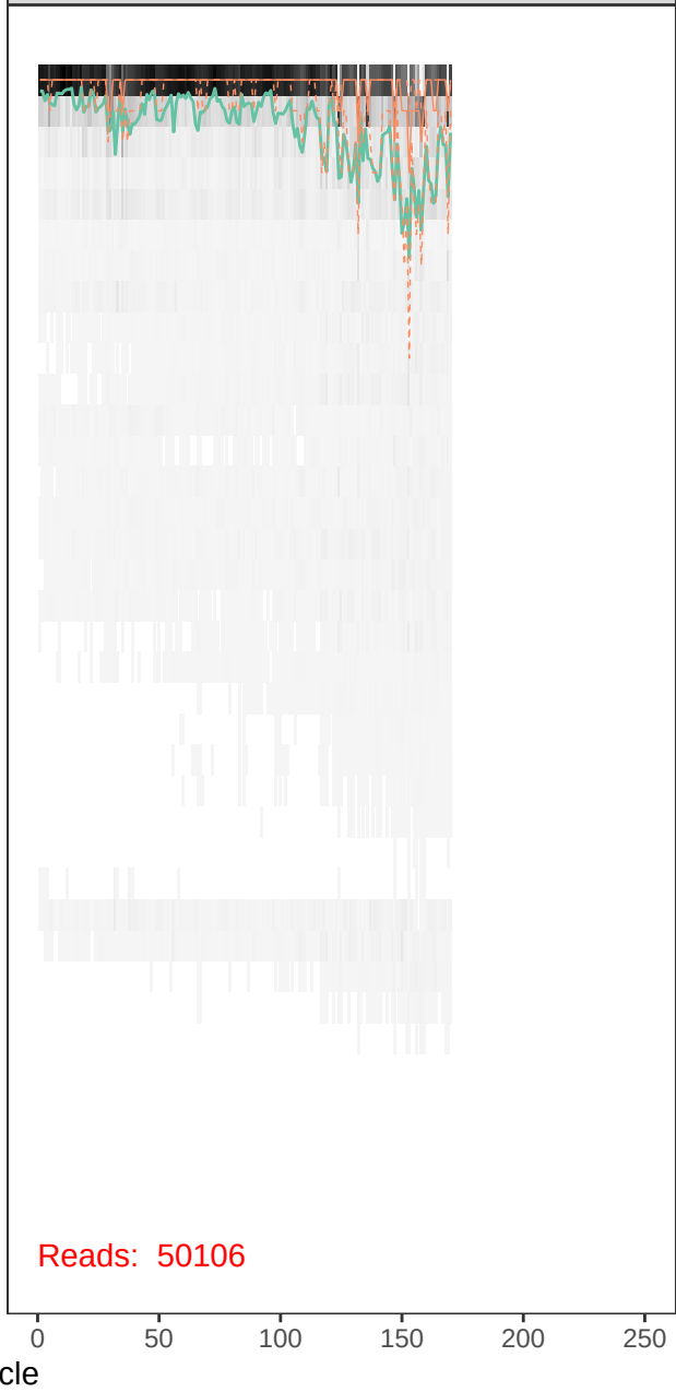
runBE05_FLD0101-r1_R_filt.fastq
