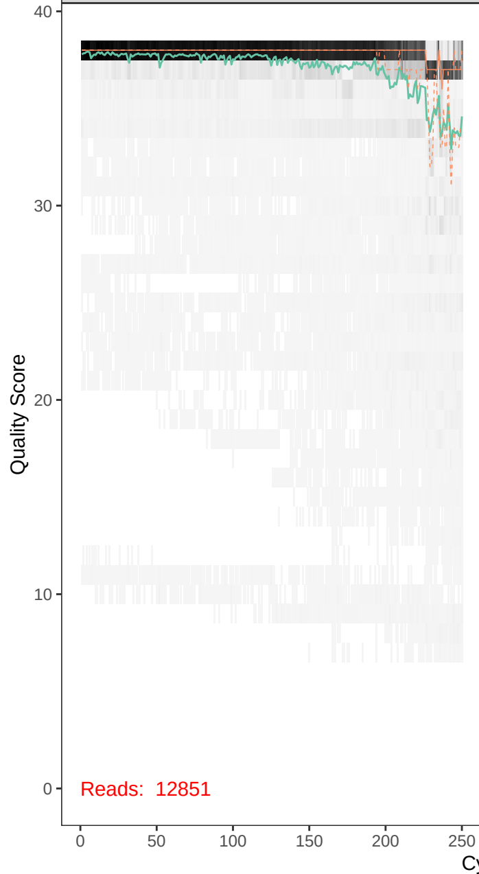
runBE08_F60R48-r1_F_filt.fastq
