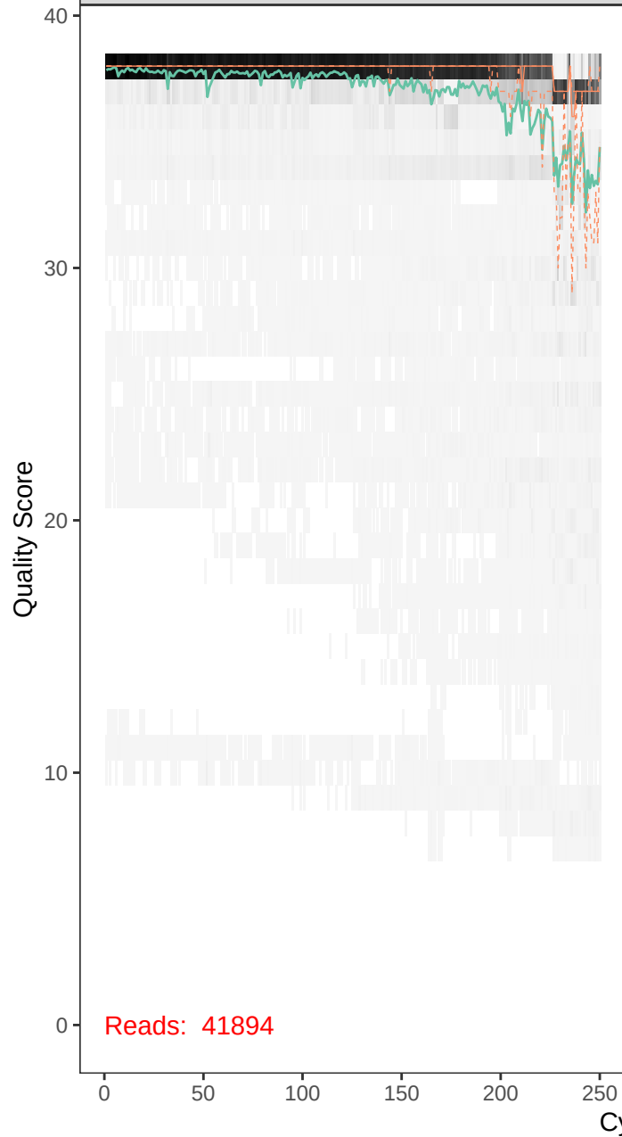
runBE08_F73R53-r1_F_filt.fastq
