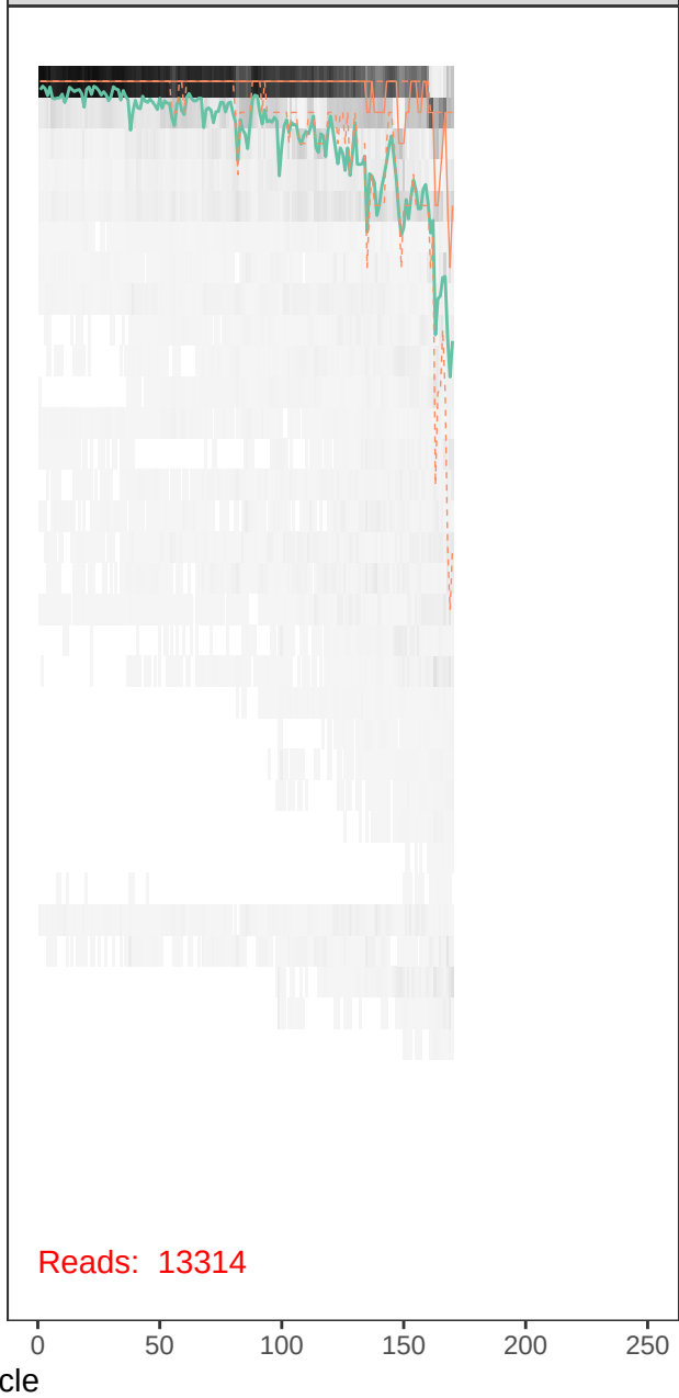
runBE08_F66R40-r1_R_filt.fastq
