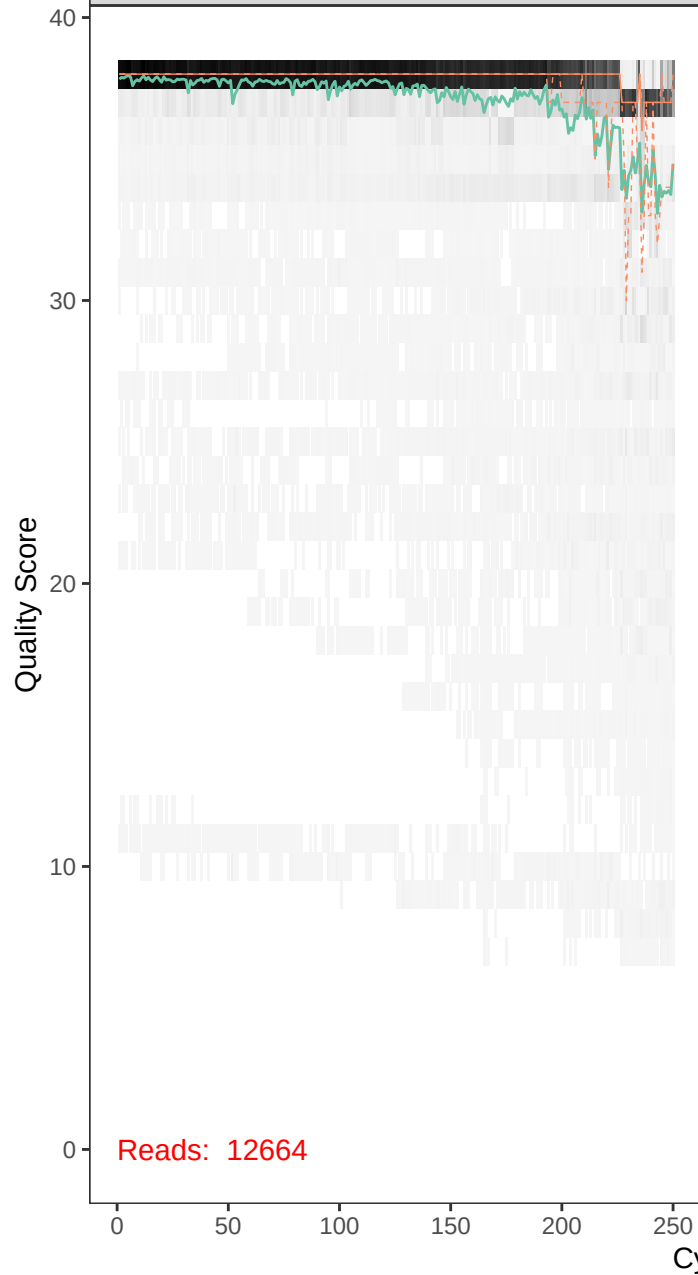
runBE08_F61R40-r1_F_filt.fastq
