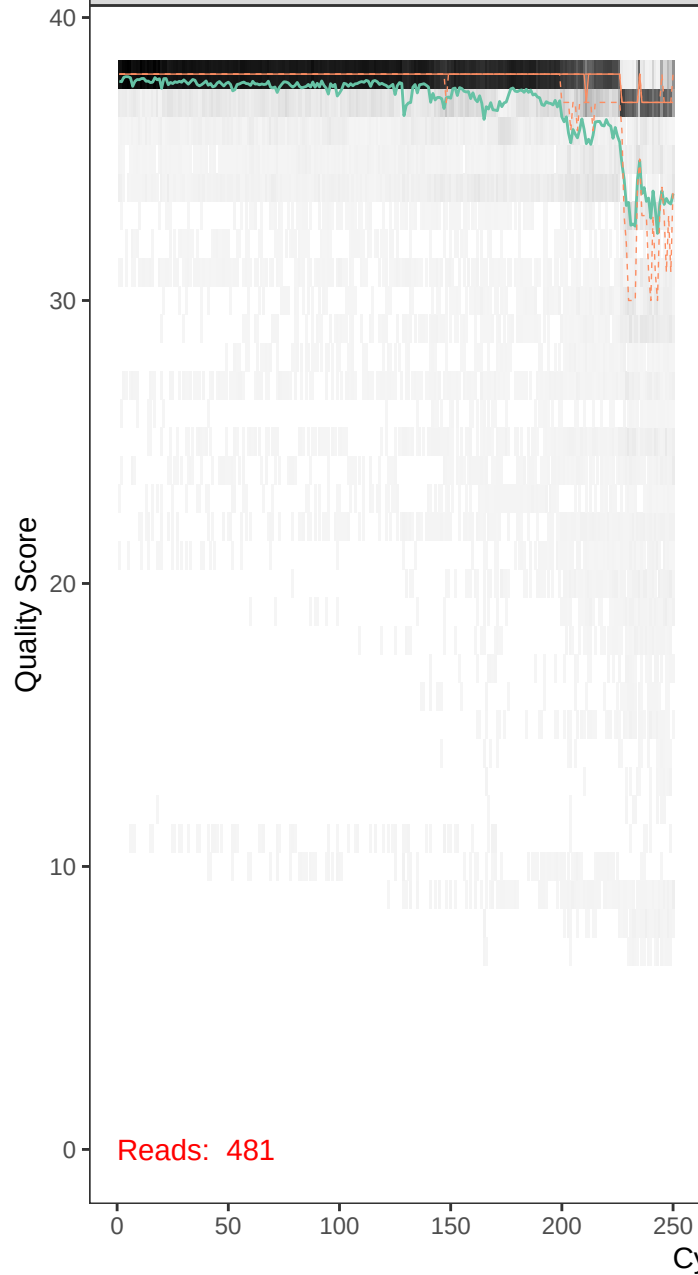
runBE08_F75R48-r1_F_filt.fastq
