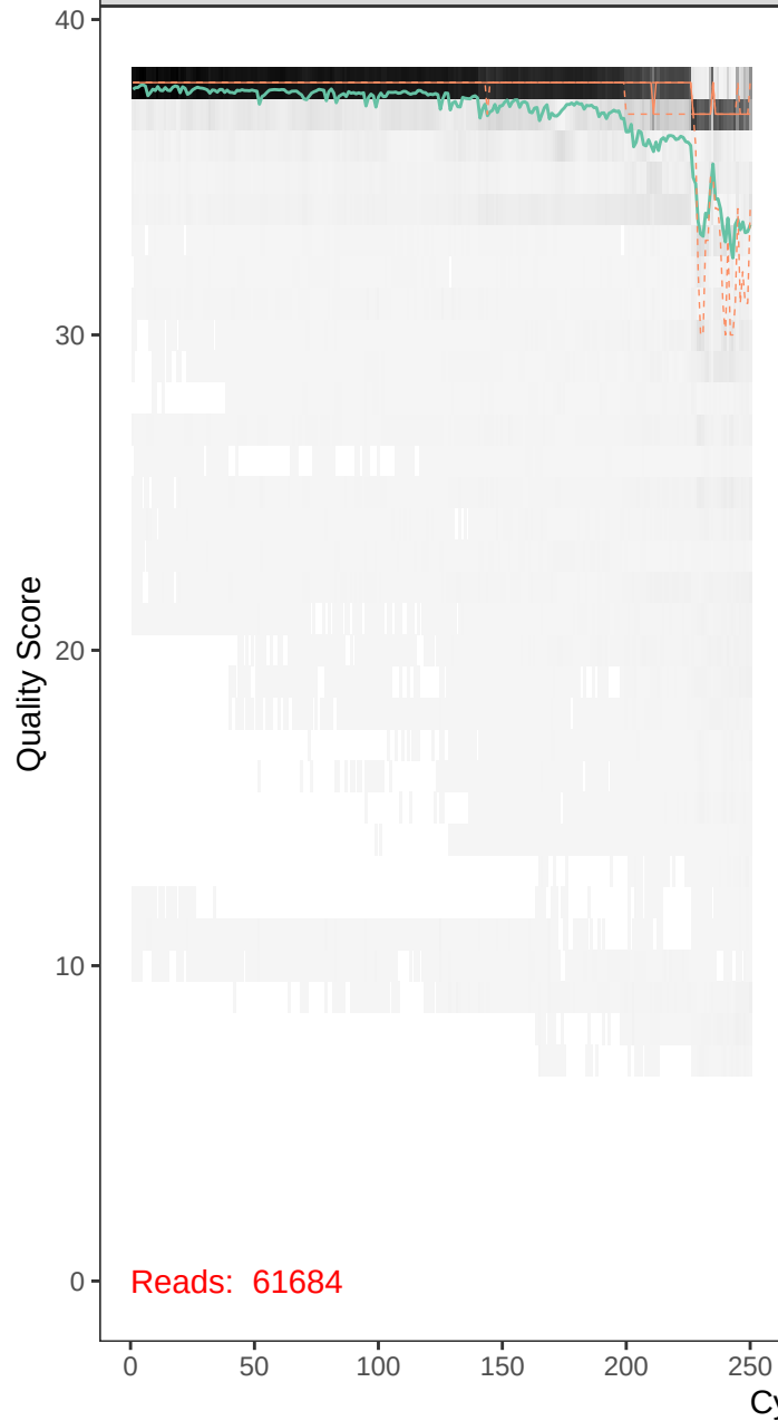
runBE08_F72R49-r1_F_filt.fastq
