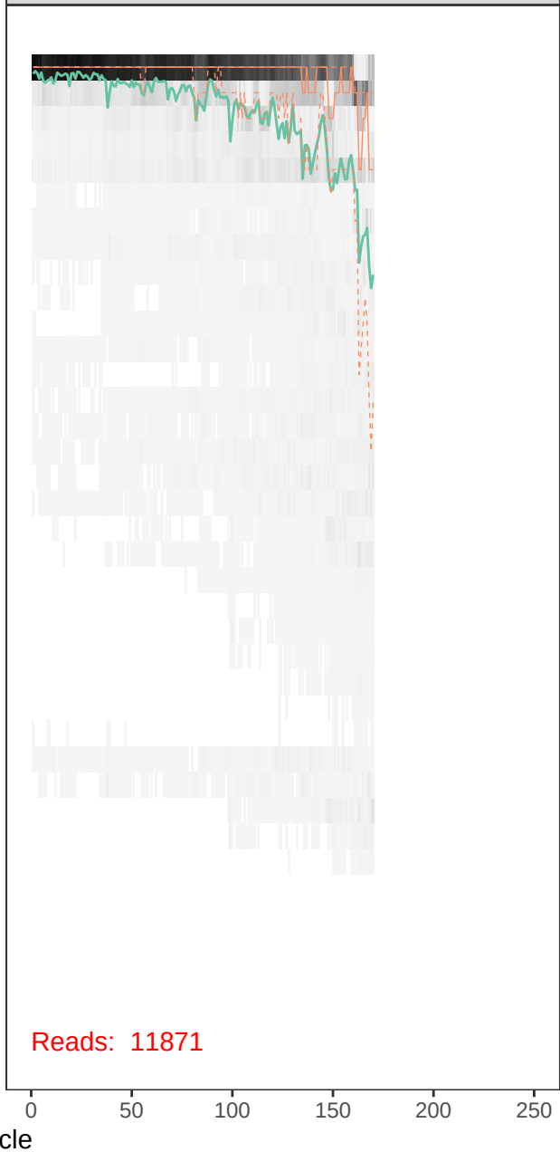
runBE08_F67R44-r1_R_filt.fastq
