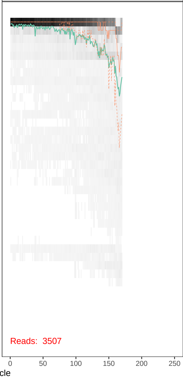
runBE08_F74R45-r1_R_filt.fastq
