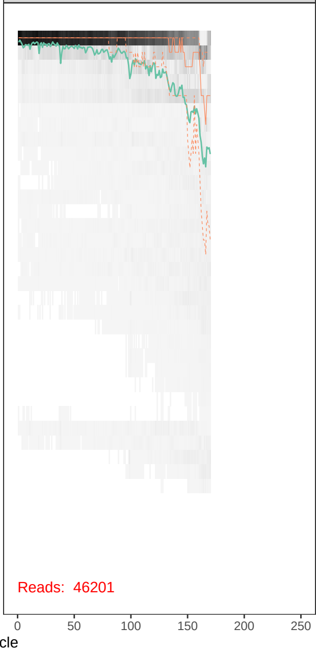
runBE08_F70R45-r1_R_filt.fastq
