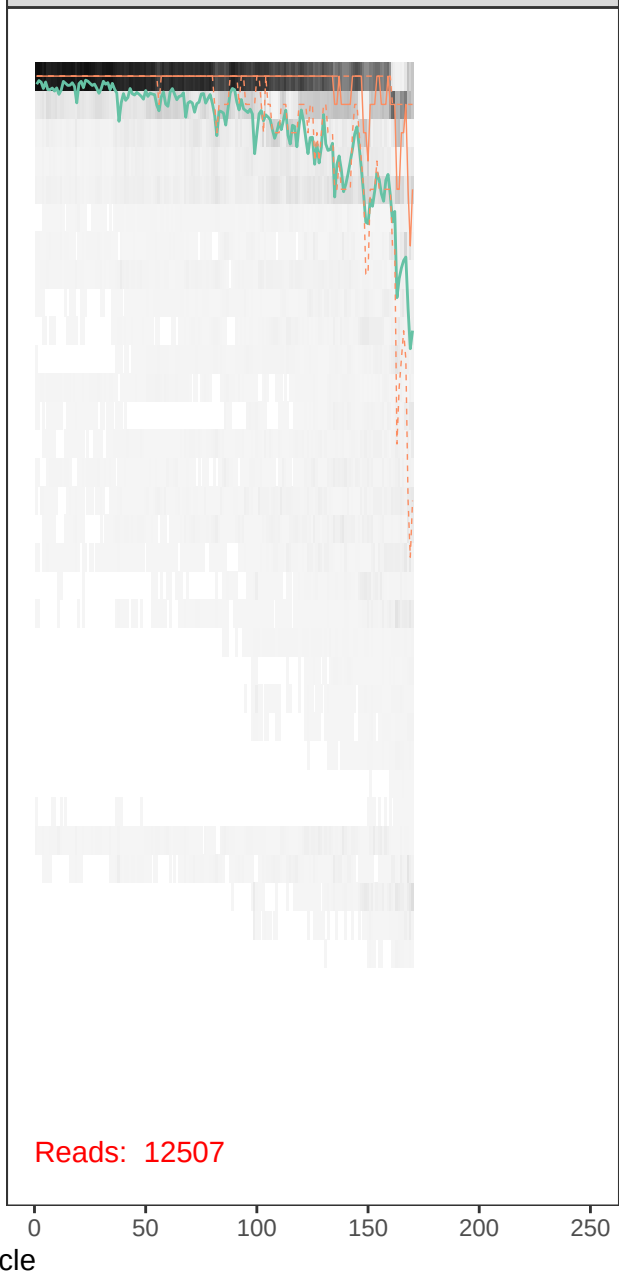
runBE08_F64R40-r1_R_filt.fastq
