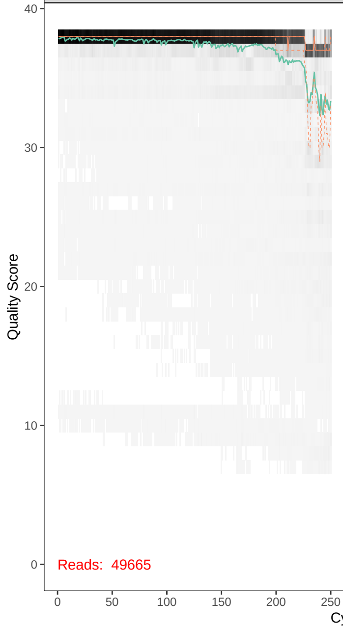
runBE08_F60R55-r1_F_filt.fastq
