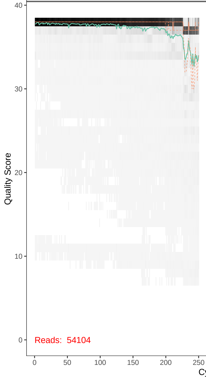
runBE08_F72R54-r1_F_filt.fastq
