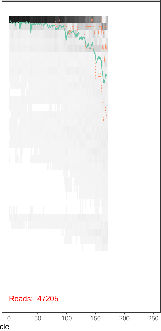
runBE08_F71R45-r1_R_filt.fastq
