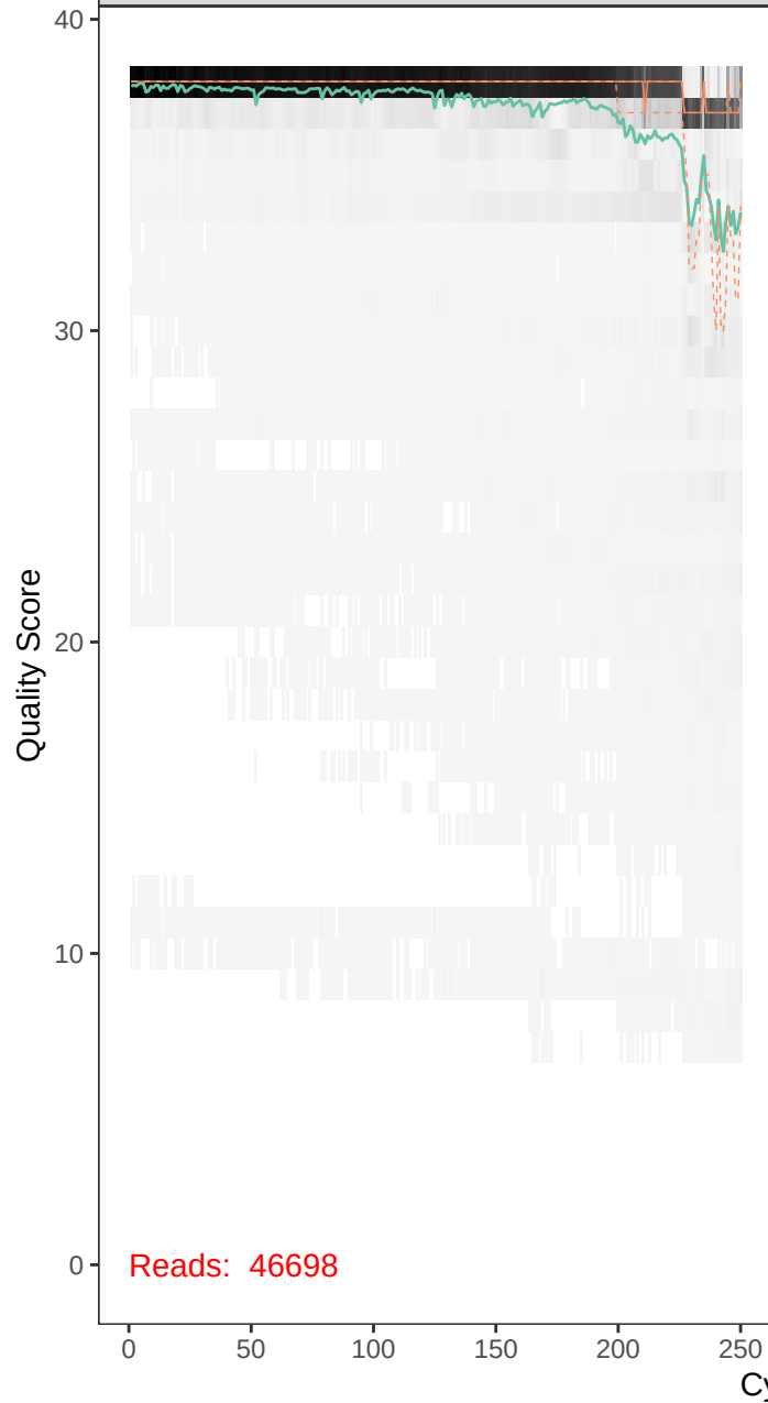
runBE08_F72R45-r1_F_filt.fastq
