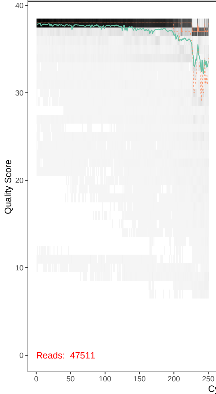
runBE08_F69R43-r1_F_filt.fastq
