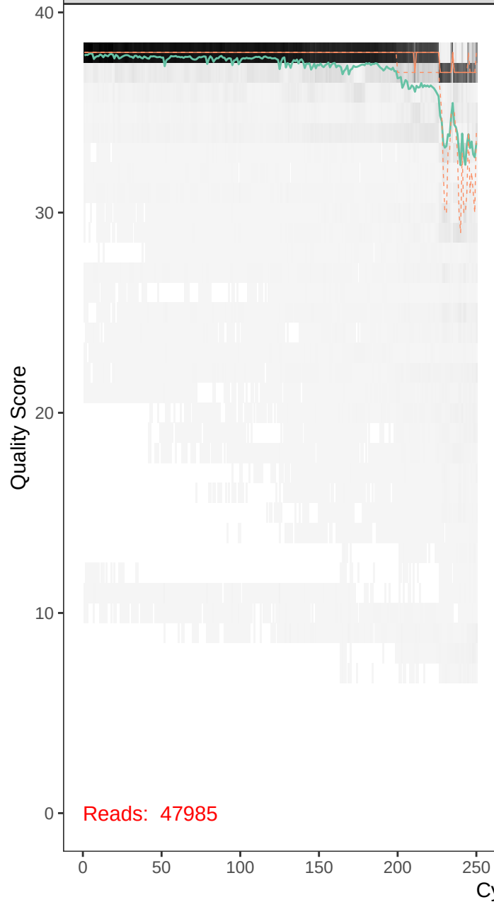
runBE08_F68R55-r1_F_filt.fastq
