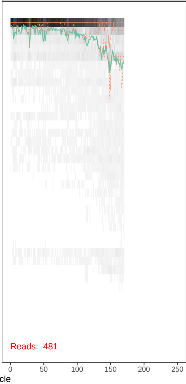
runBE08_F75R48-r1_R_filt.fastq
