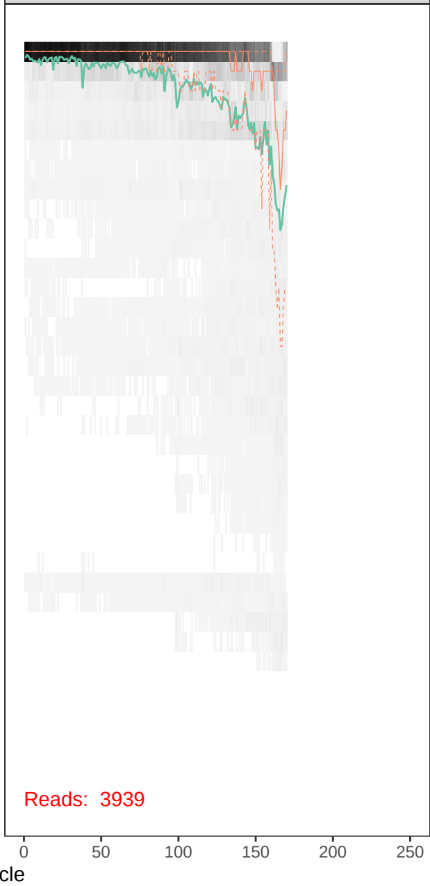
runBE08_F74R42-r1_R_filt.fastq
