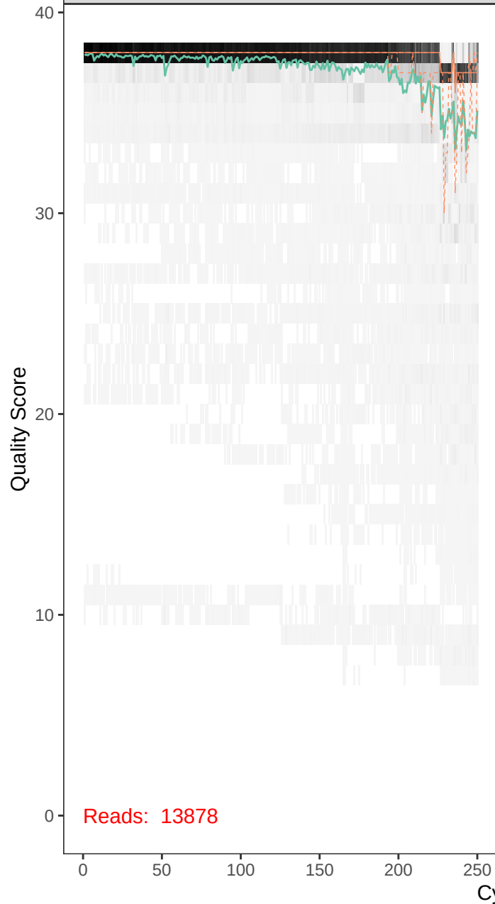
runBE08_F66R48-r1_F_filt.fastq
