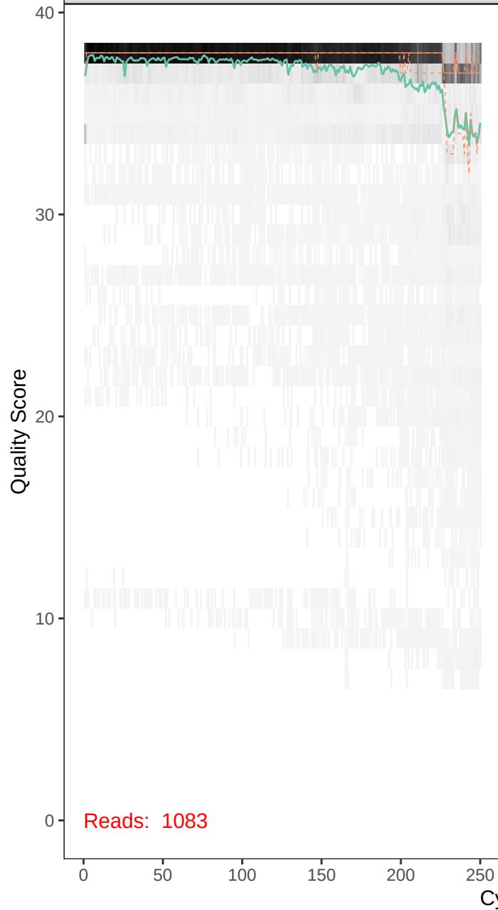
runBE08_F74R48-r1_F_filt.fastq
