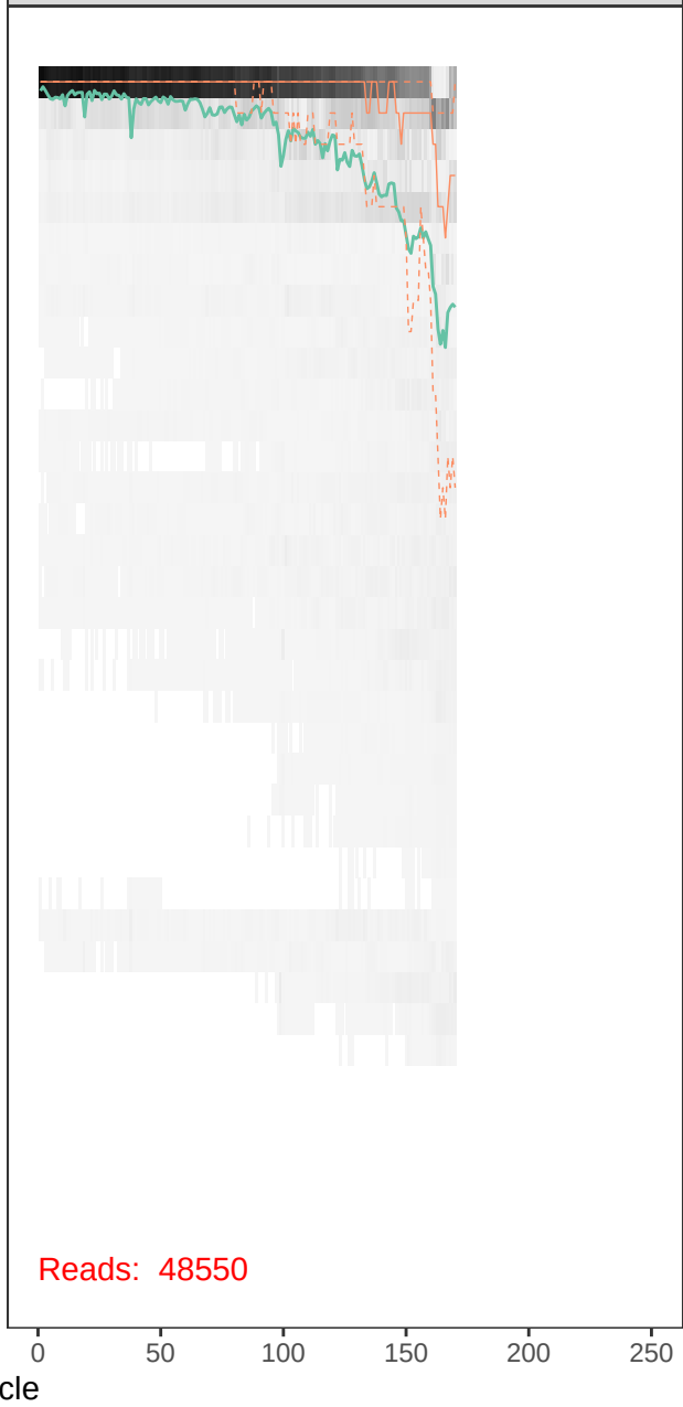
runBE08_F72R44-r1_R_filt.fastq
