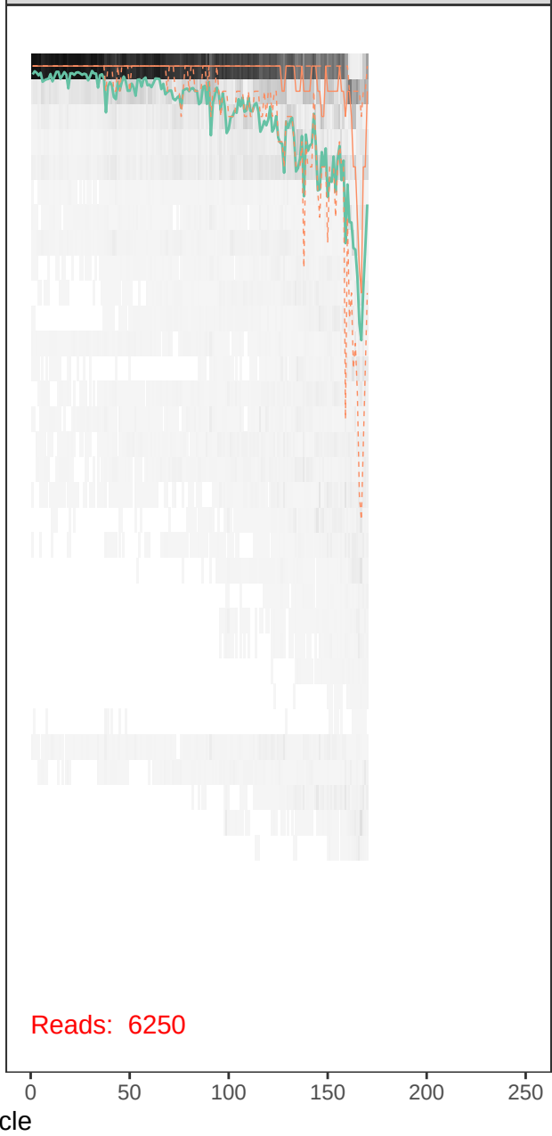
runBE08_F74R51-r1_R_filt.fastq
