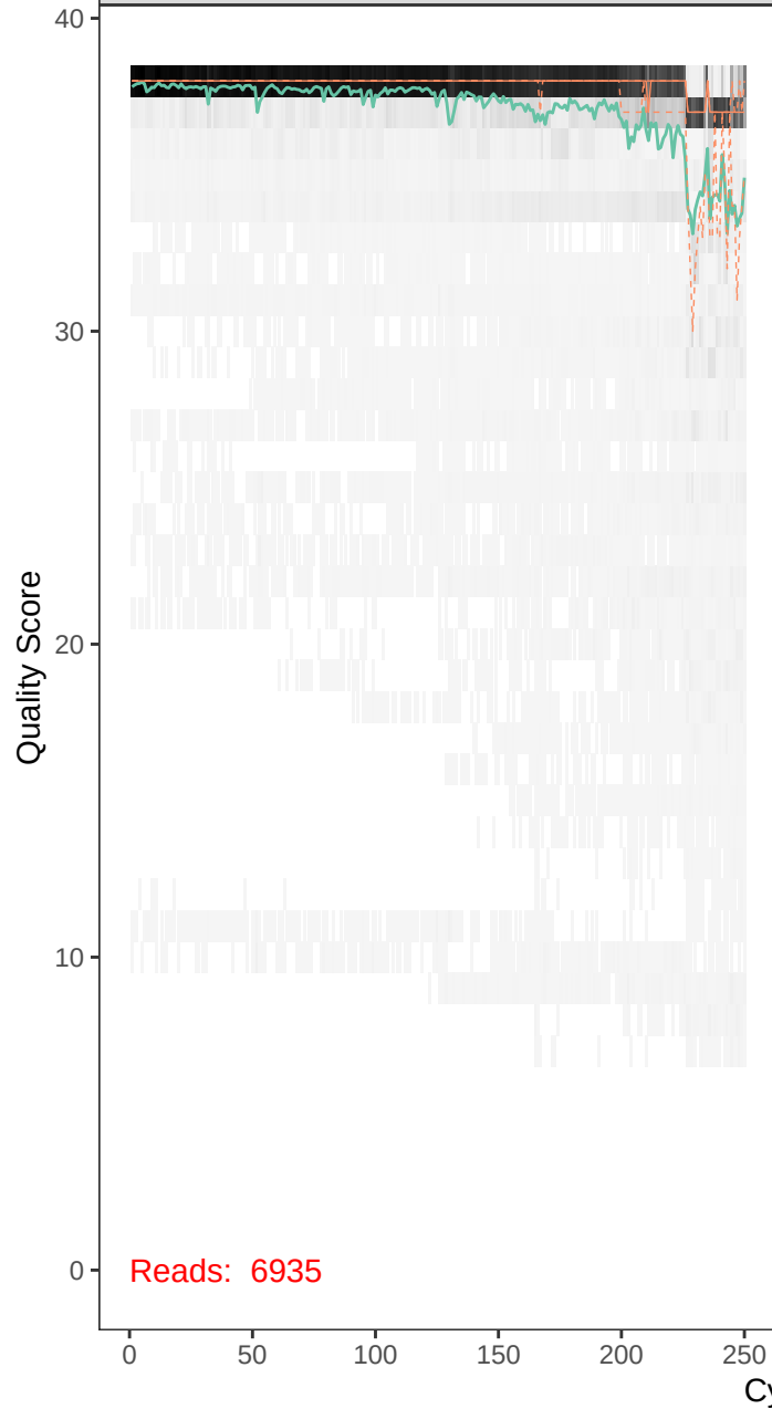
runBE08_F71R52-r1_F_filt.fastq
