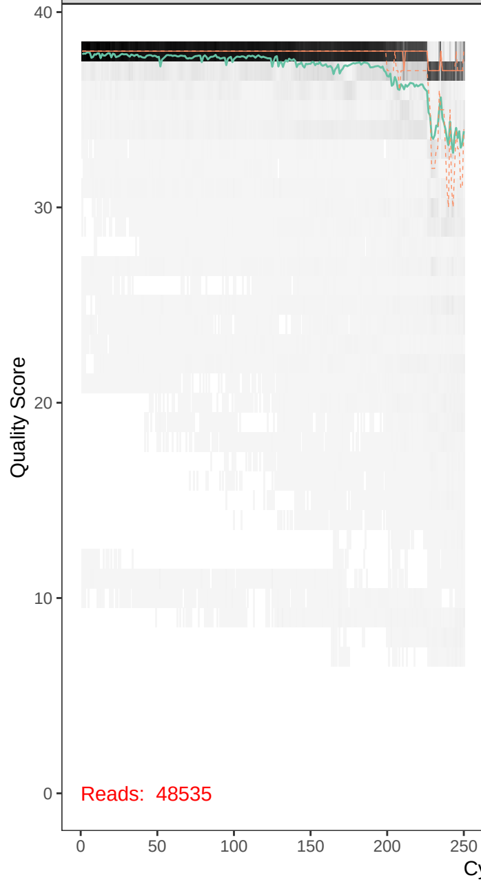
runBE08_F72R55-r1_F_filt.fastq
