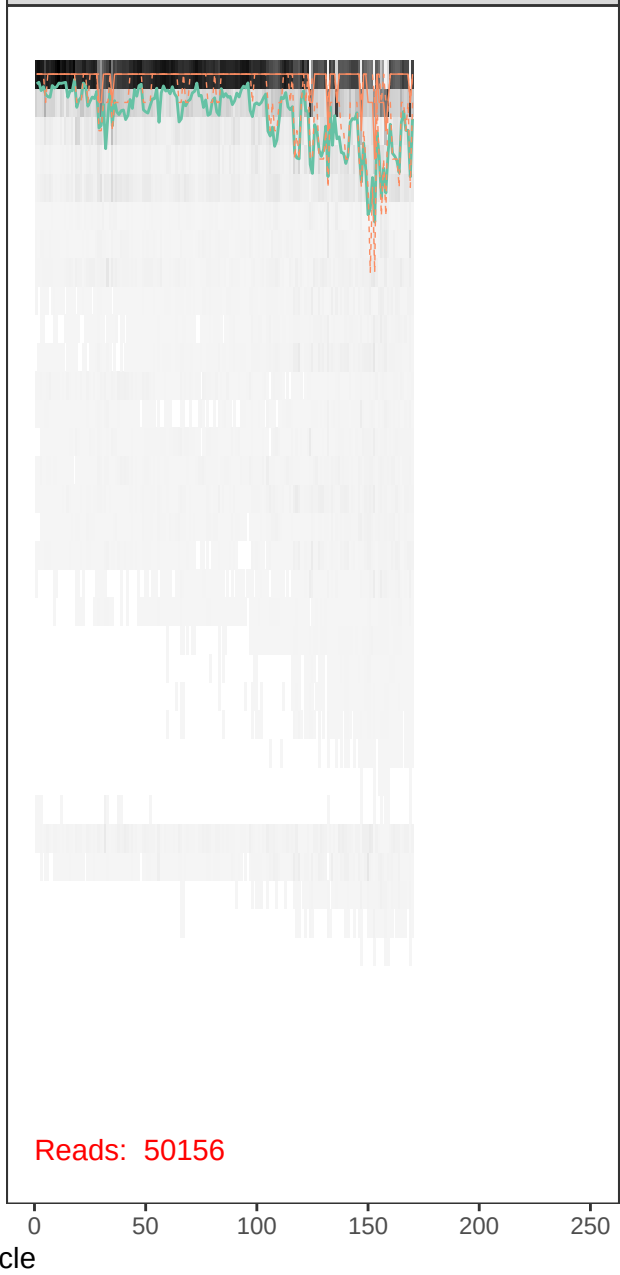
runBE05_FLD0100-r1_R_filt.fastq
