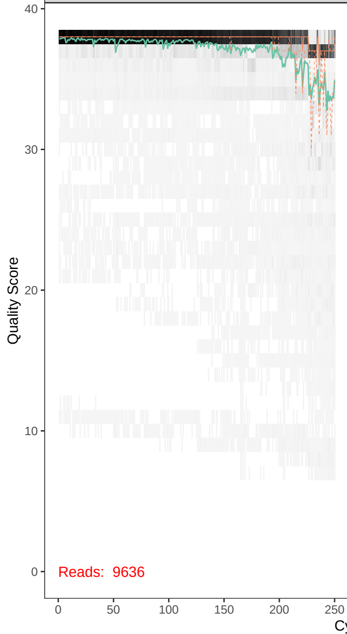
runBE08_F65R46-r1_F_filt.fastq
