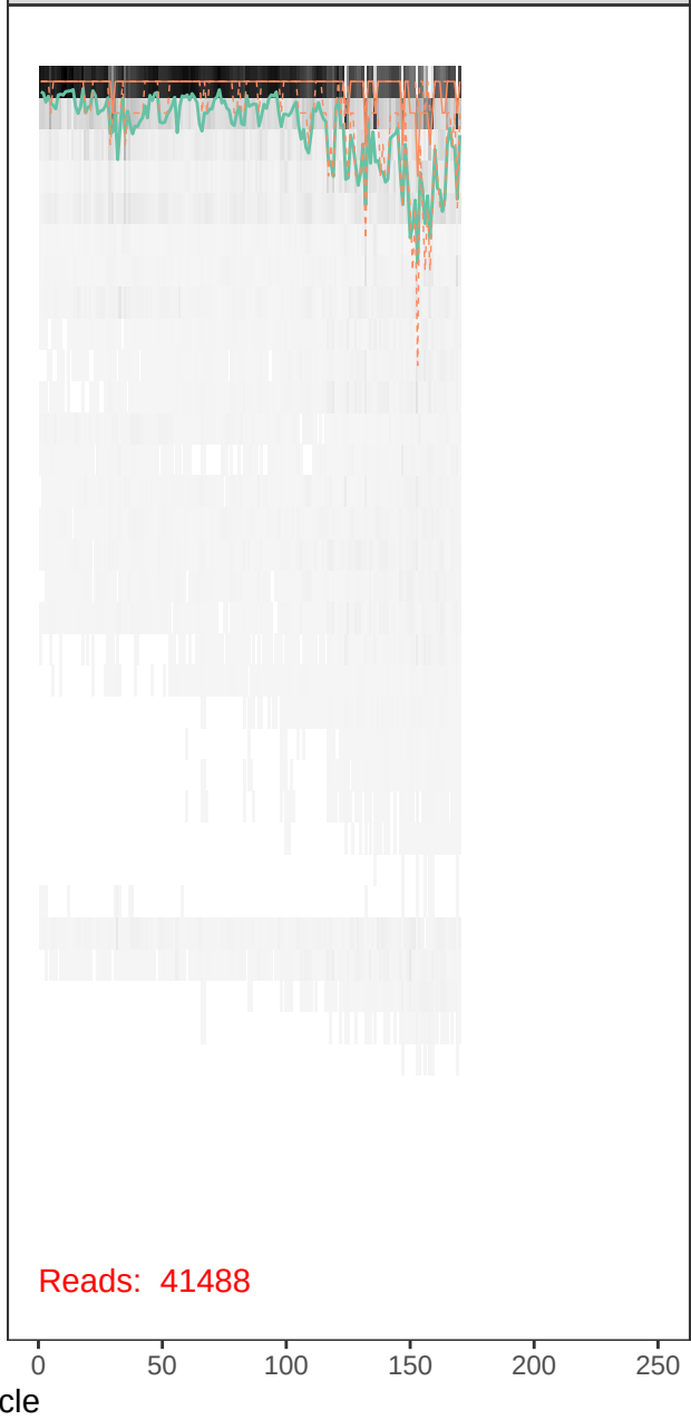
runBE05_FLD0117-r1_R_filt.fastq
