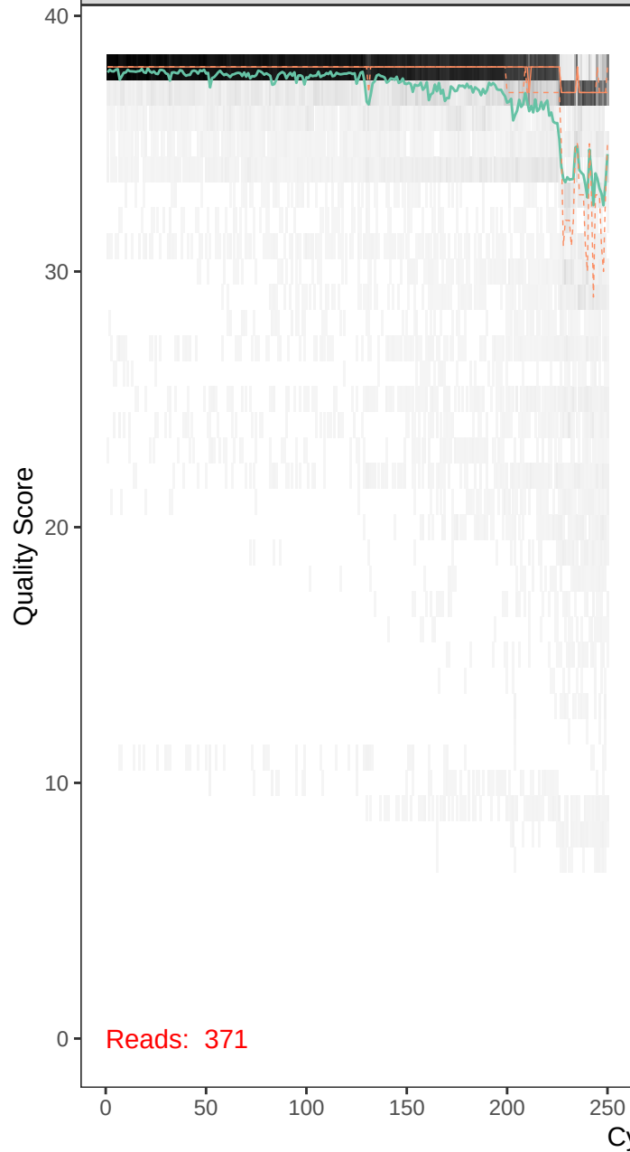
runBE08_F64R52-r1_F_filt.fastq
