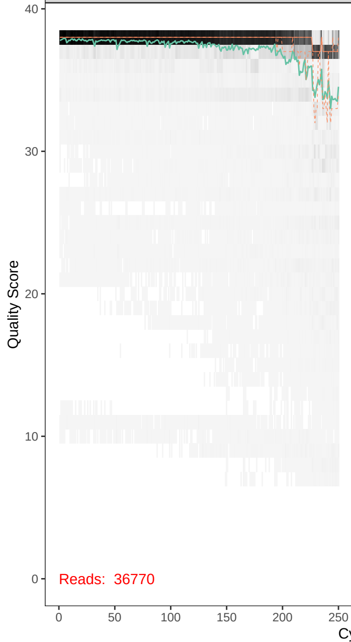
runBE08_F60R44-r1_F_filt.fastq
