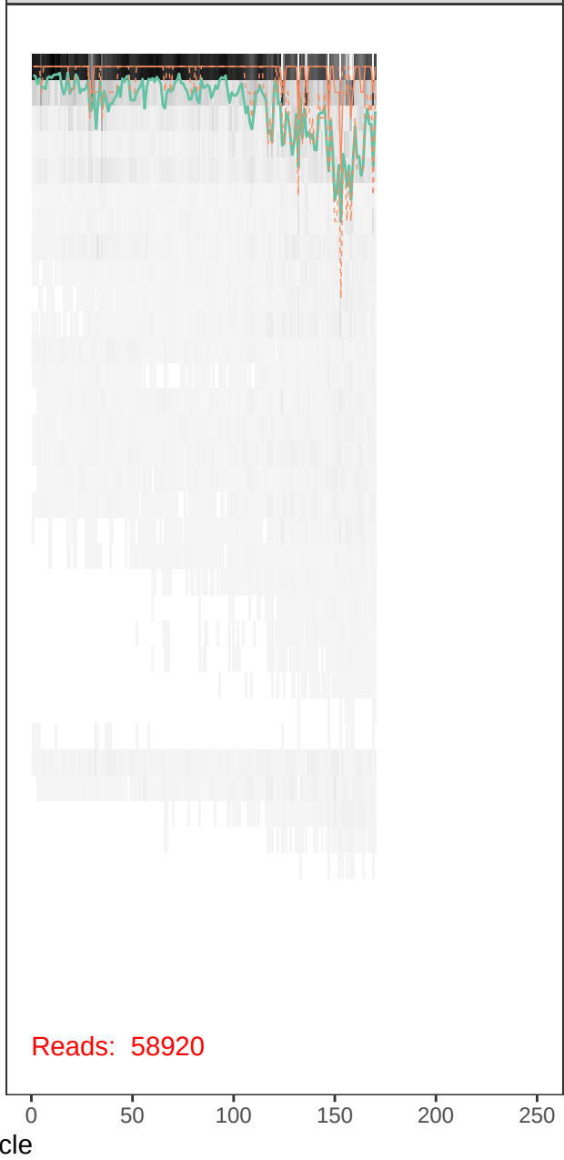
runBE05_FLD0061-r1_R_filt.fastq
