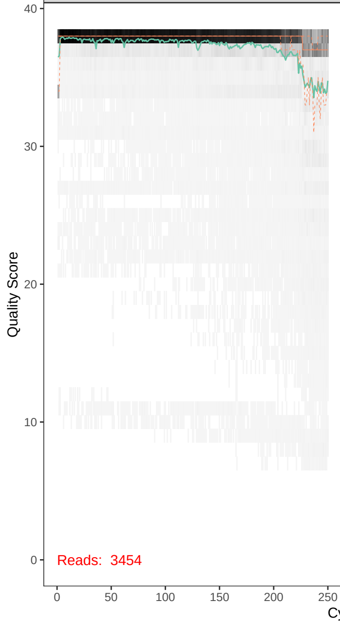
runBE08_F73R54-r1_F_filt.fastq
