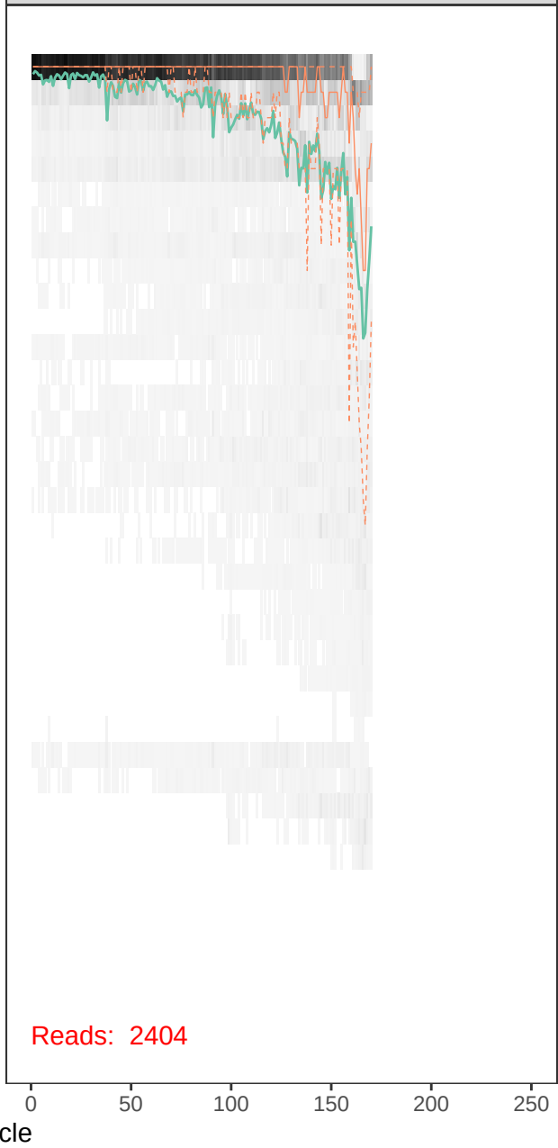
runBE08_F73R41-r1_R_filt.fastq
