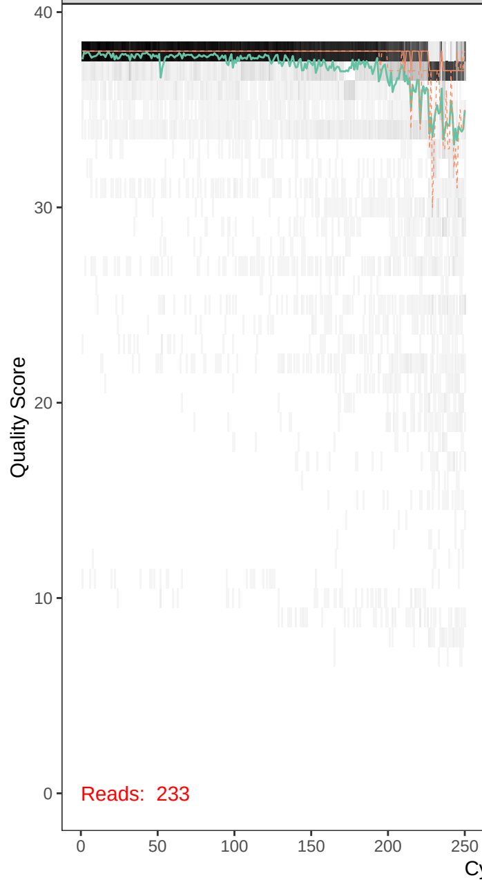
runBE08_F67R55-r1_F_filt.fastq
