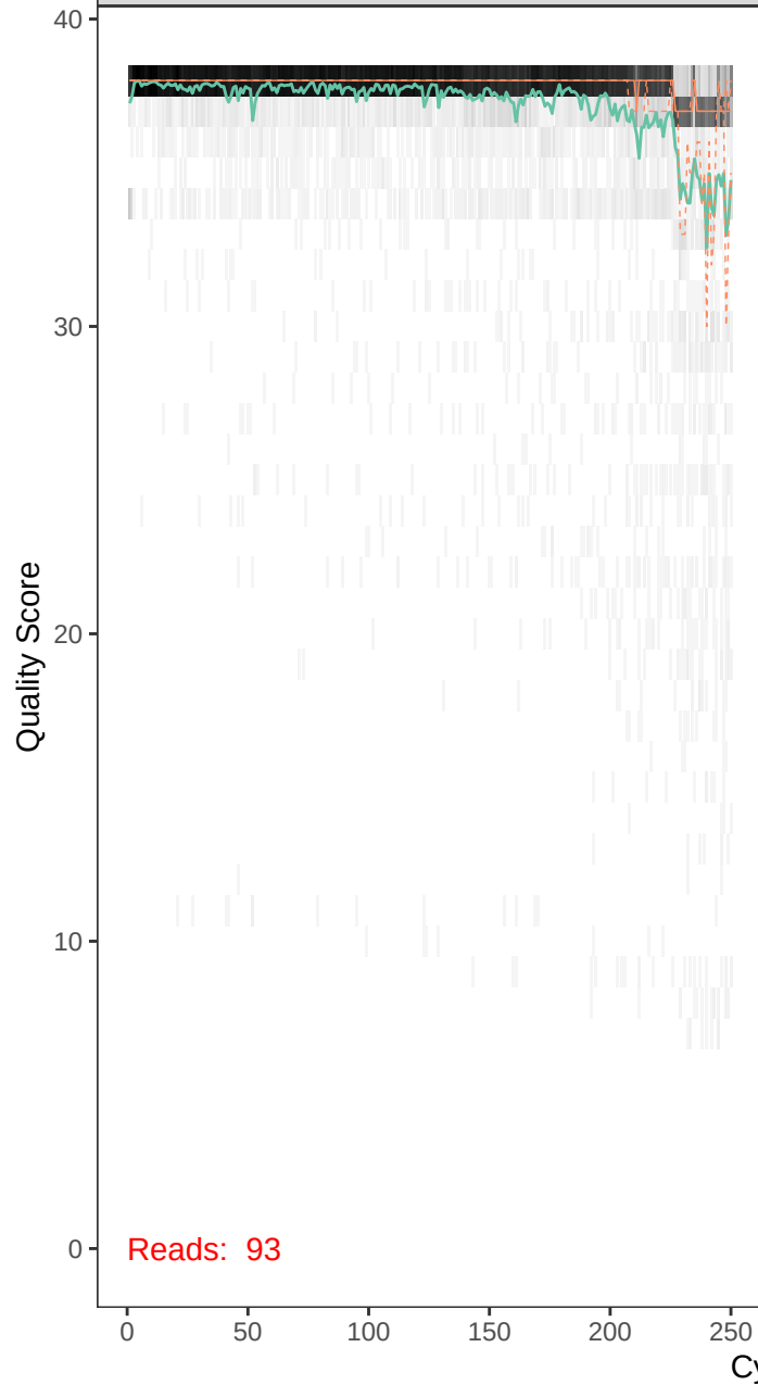
runBE08_F71R46-r1_F_filt.fastq
