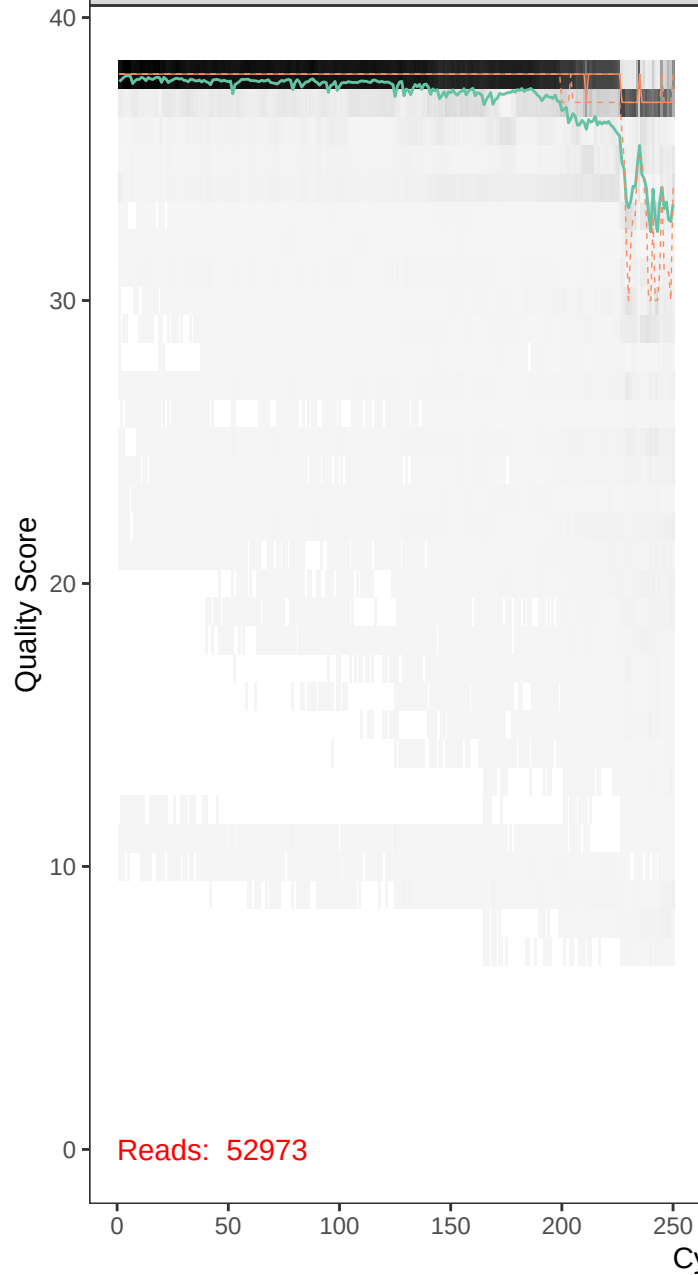
runBE08_F63R54-r1_F_filt.fastq
