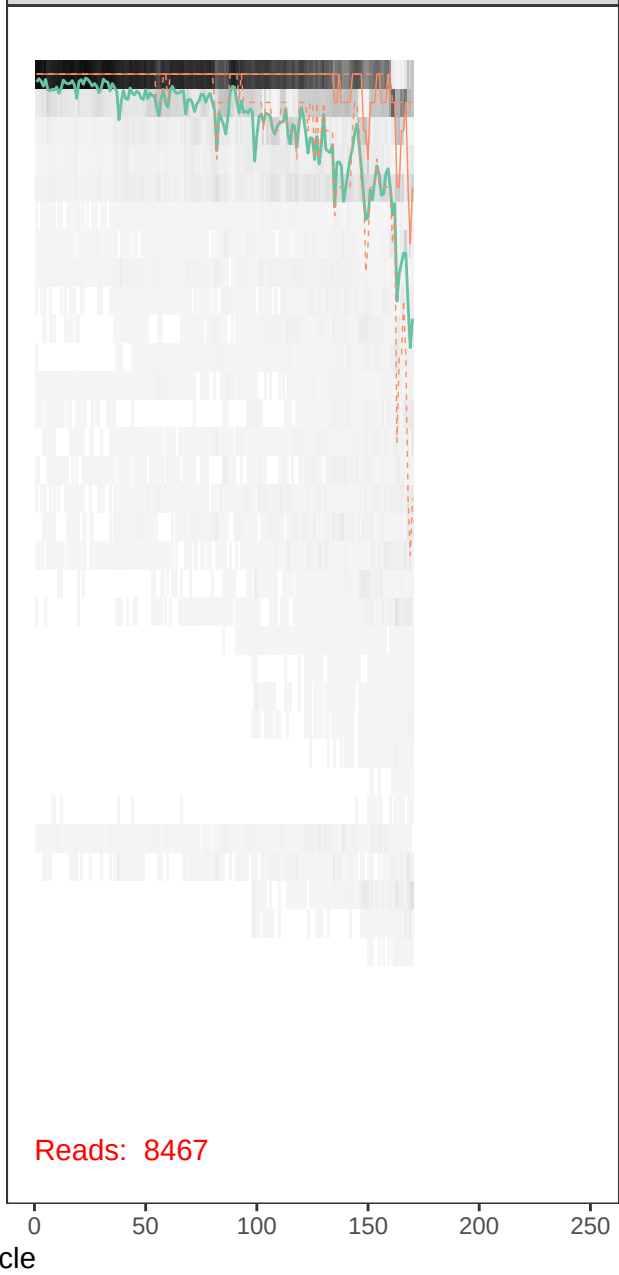
runBE08_F61R46-r1_R_filt.fastq
