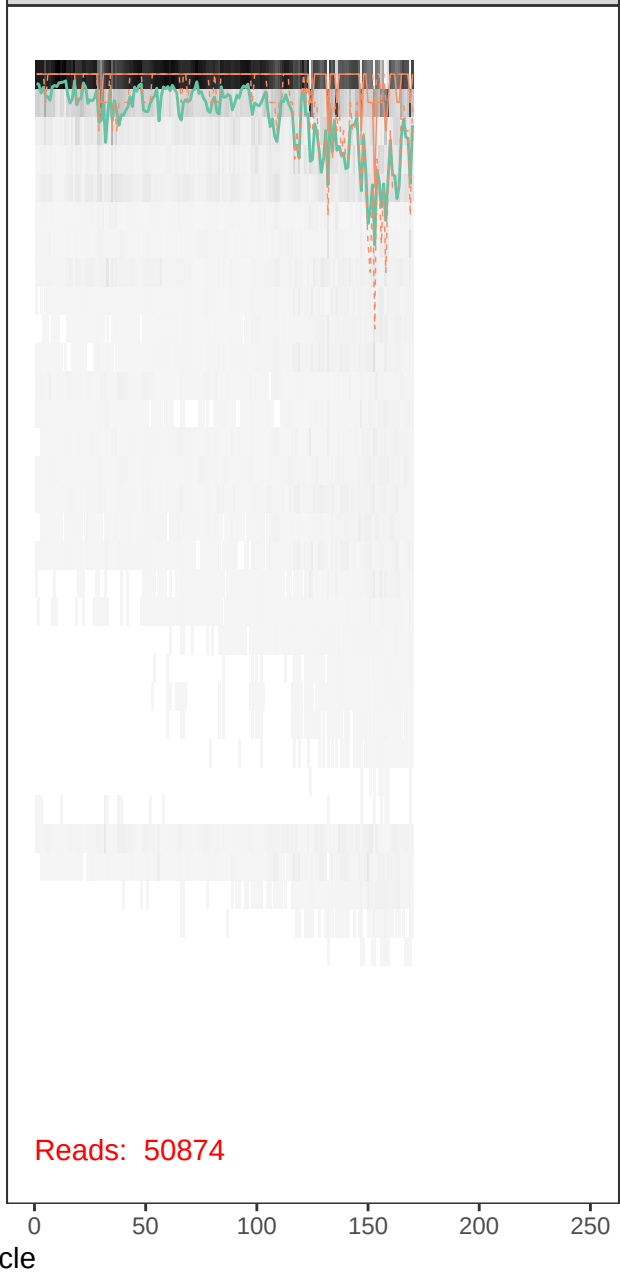
runBE05_FLD0069-r1_R_filt.fastq
