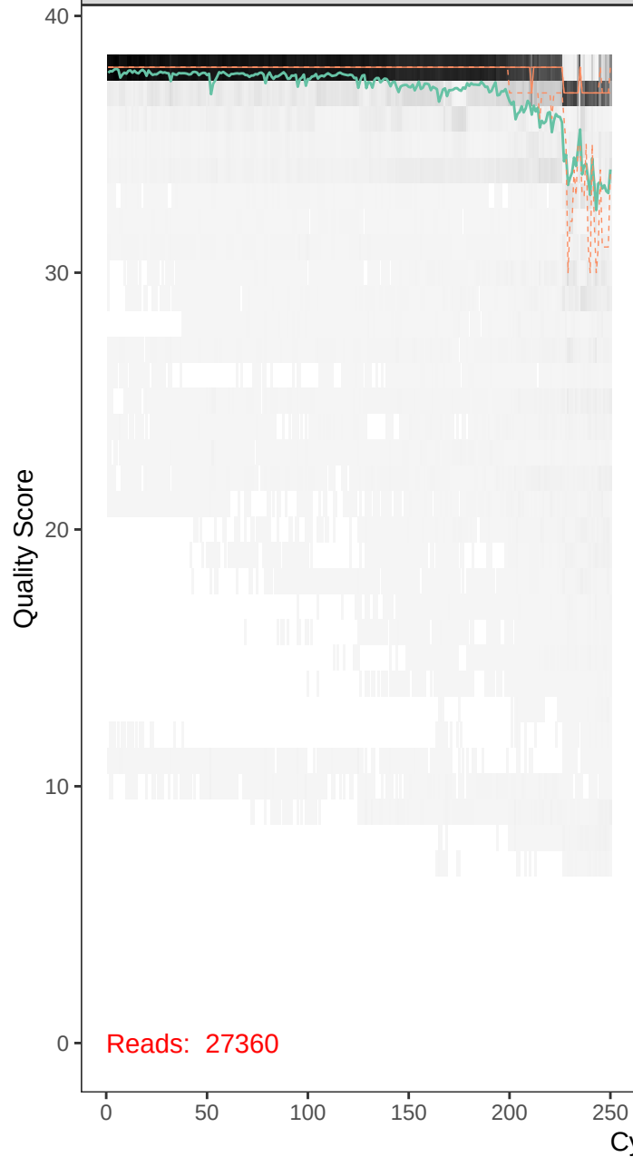
runBE08_F63R49-r1_F_filt.fastq
