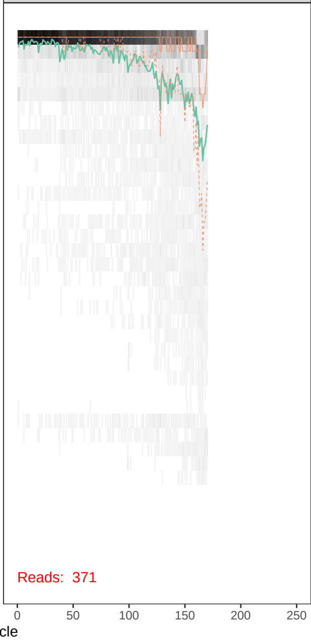
runBE08_F64R52-r1_R_filt.fastq
