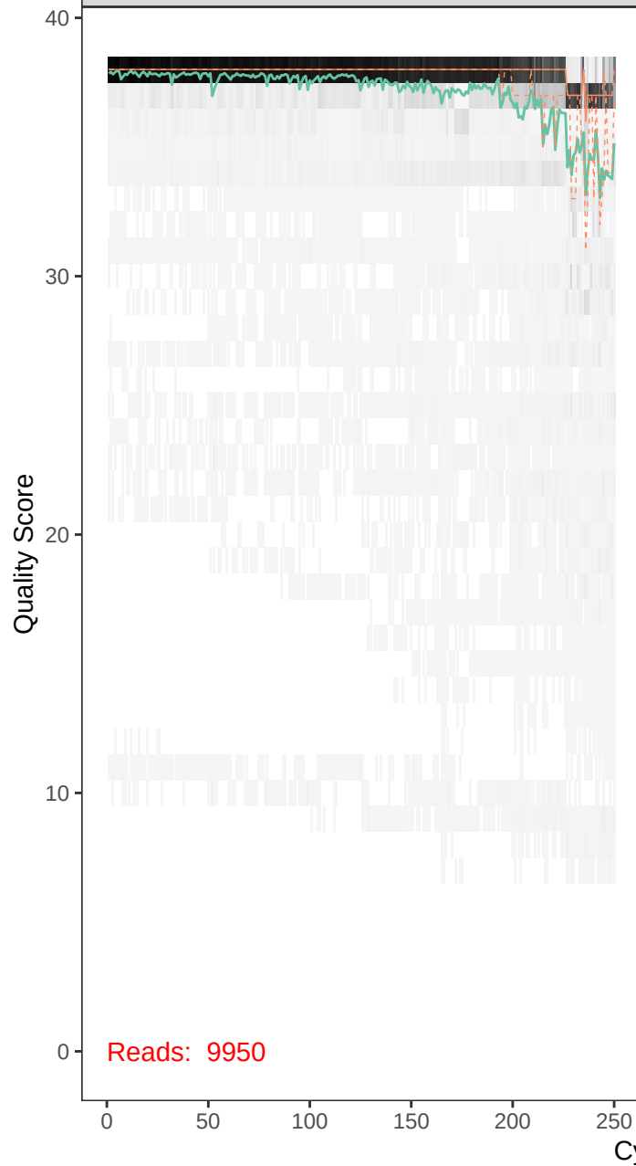
runBE08_F64R50-r1_F_filt.fastq
