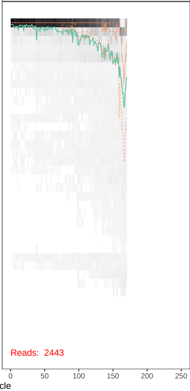
runBE08_F73R42-r1_R_filt.fastq
