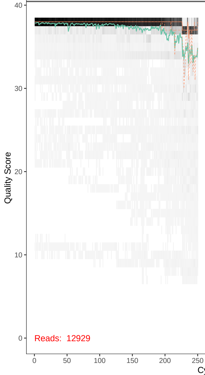
runBE08_F63R41-r1_F_filt.fastq
