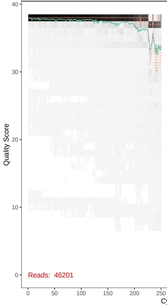
runBE08_F70R45-r1_F_filt.fastq
