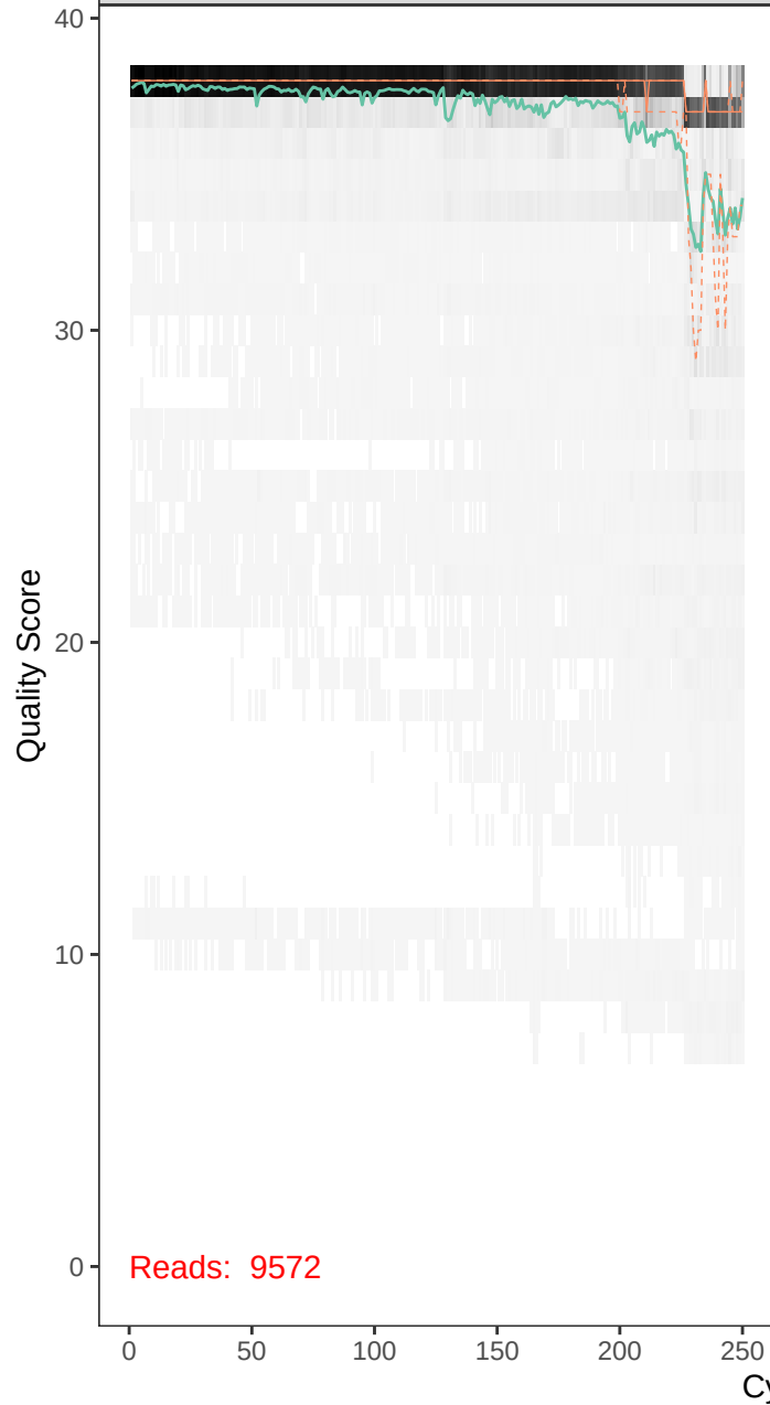
runBE08_F69R52-r1_F_filt.fastq
