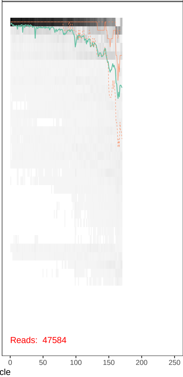
runBE08_F64R54-r1_R_filt.fastq
