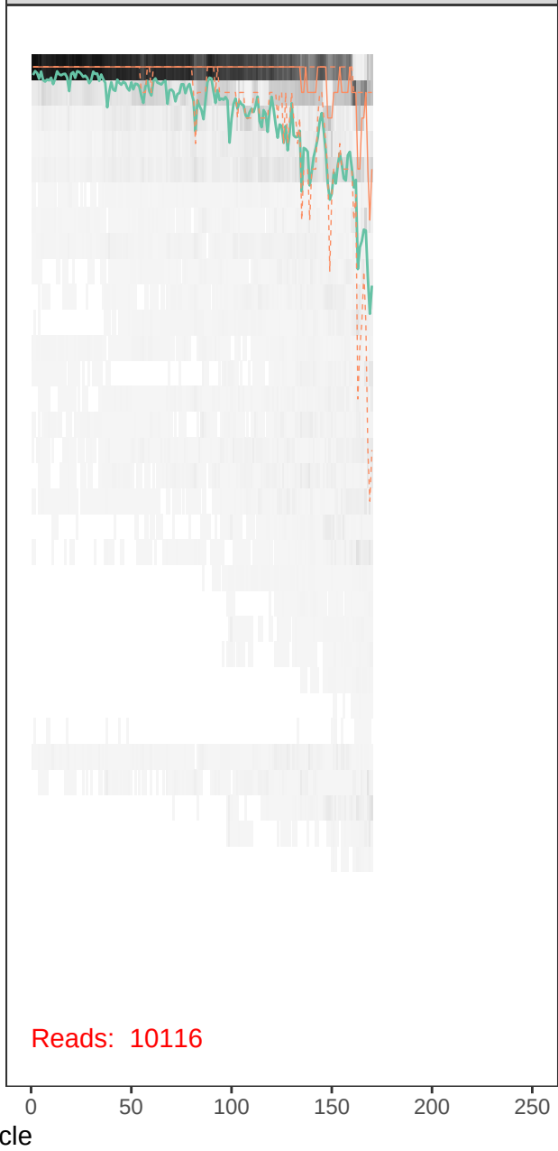
runBE08_F63R40-r1_R_filt.fastq
