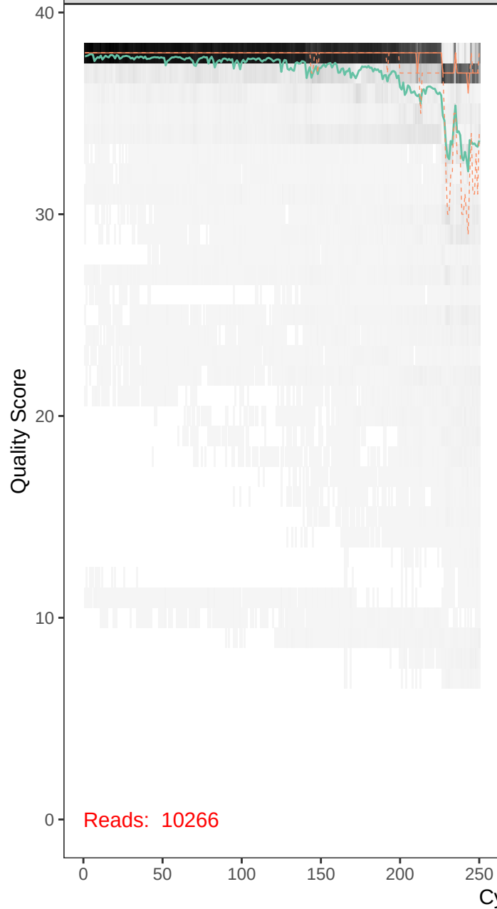
runBE08_F71R51-r1_F_filt.fastq
