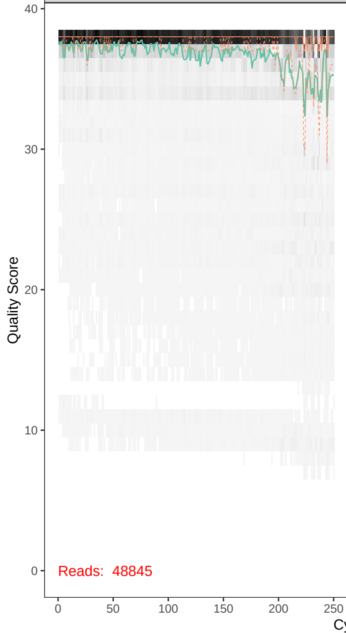
runBE05_FLD0127-r1_F_filt.fastq
