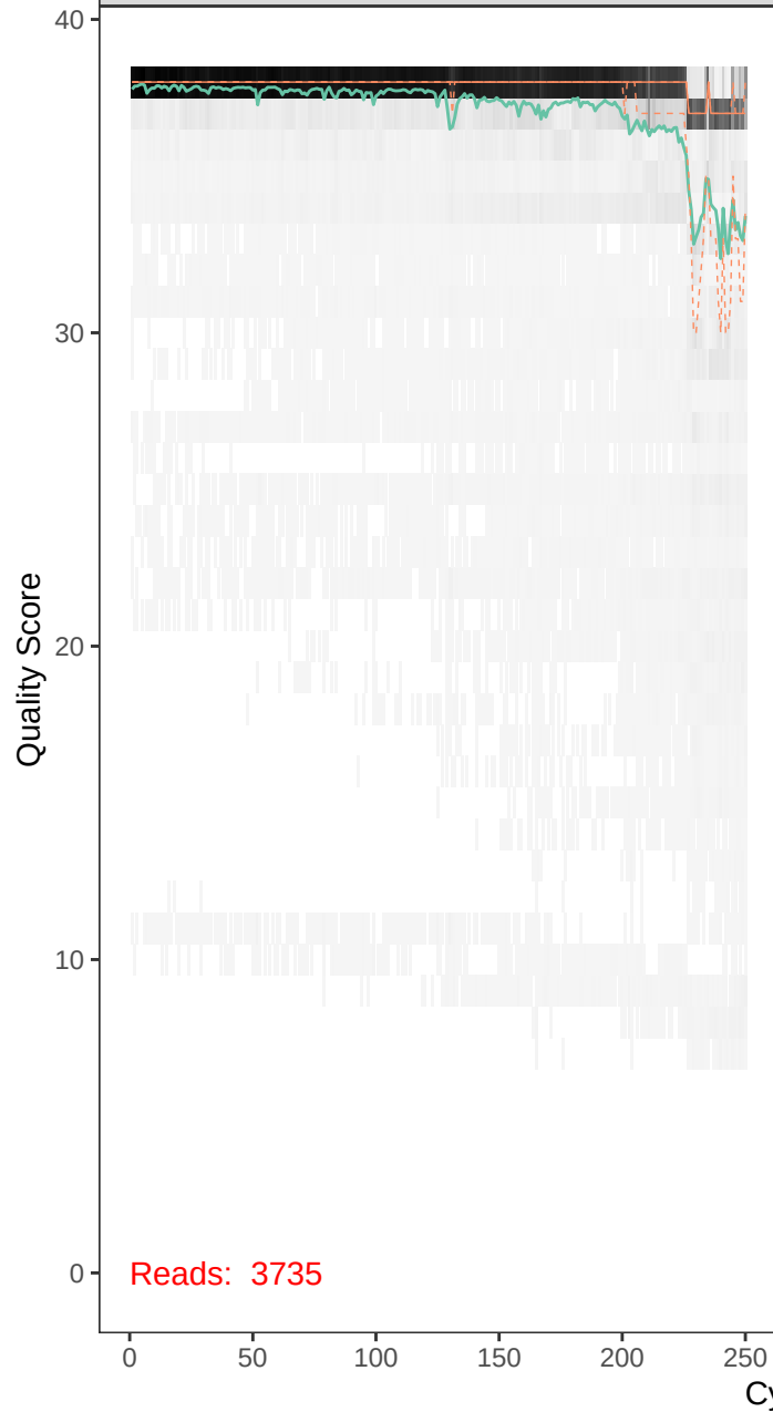
runBE08_F62R52-r1_F_filt.fastq
