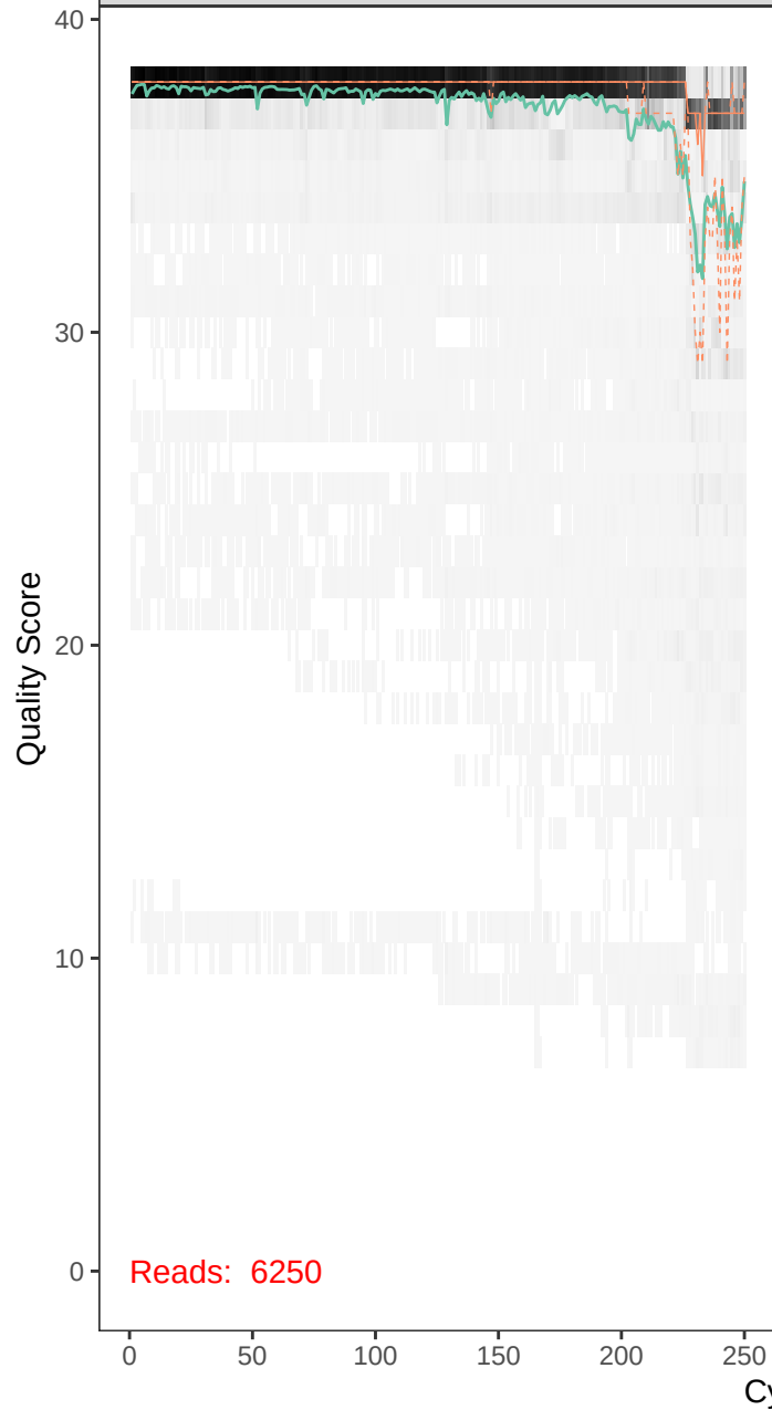
runBE08_F74R51-r1_F_filt.fastq
