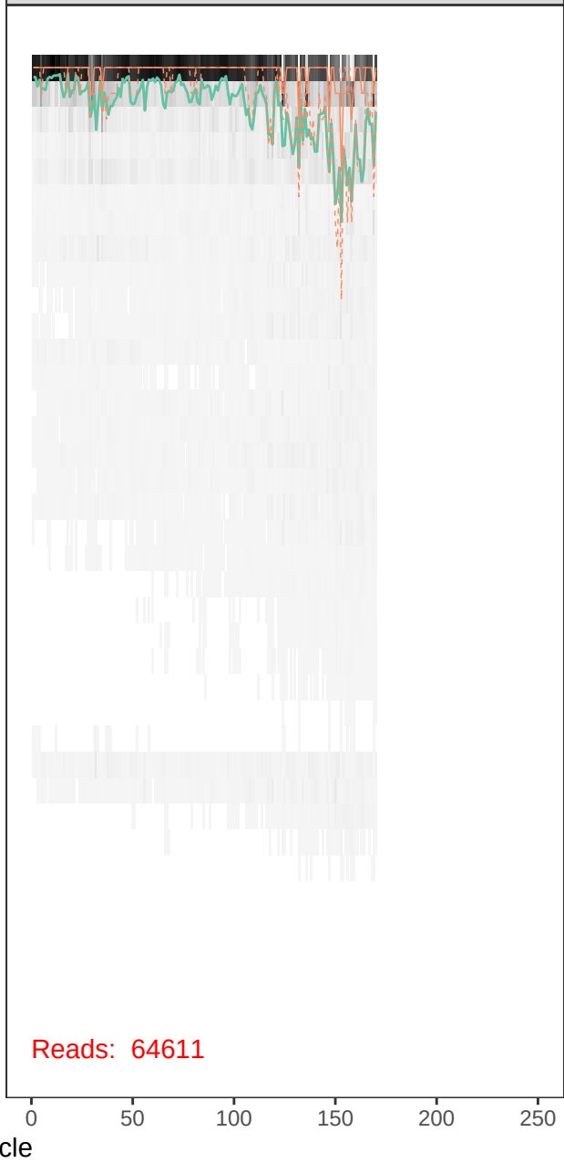
runBE05_FLD0350-r1_R_filt.fastq
