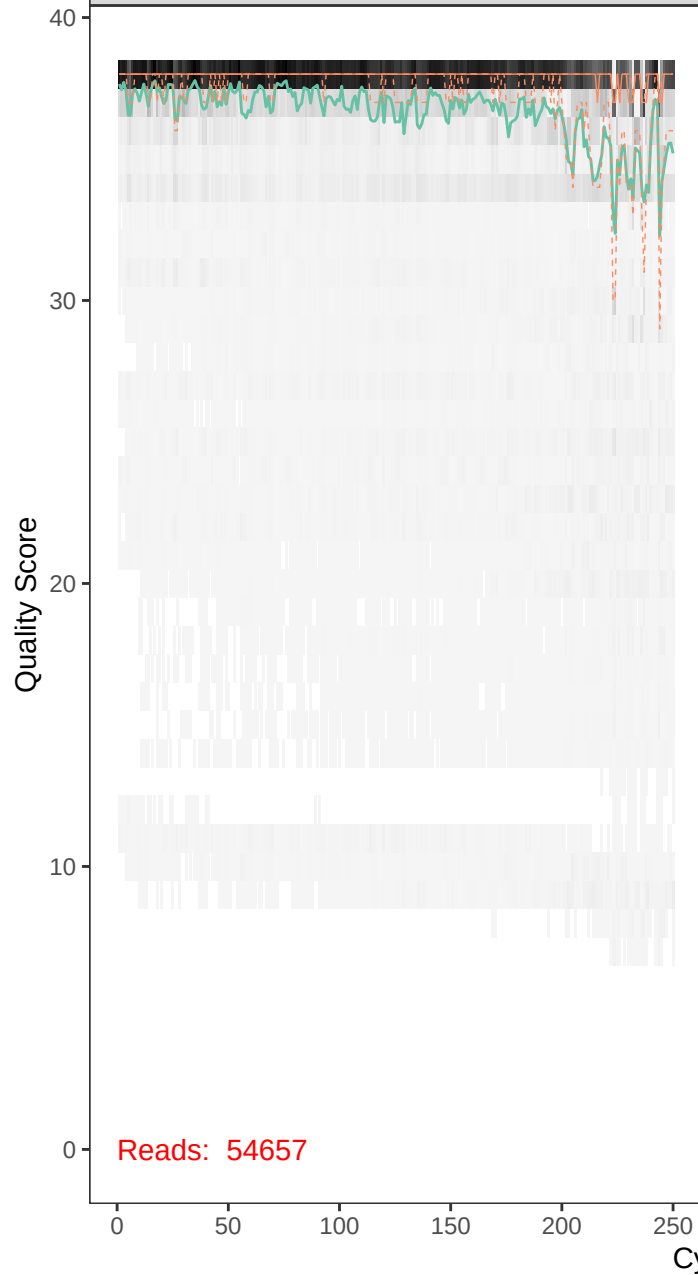
runBE05_FLD0134-r1_F_filt.fastq
