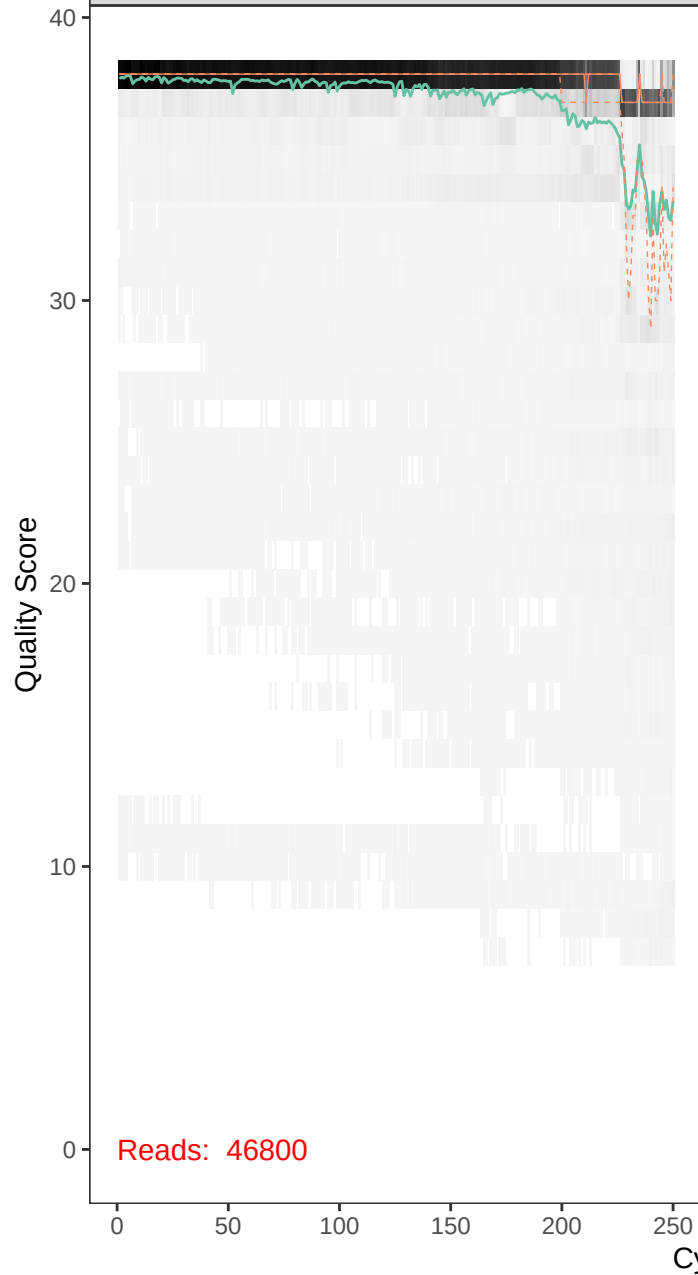
runBE08_F68R53-r1_F_filt.fastq
