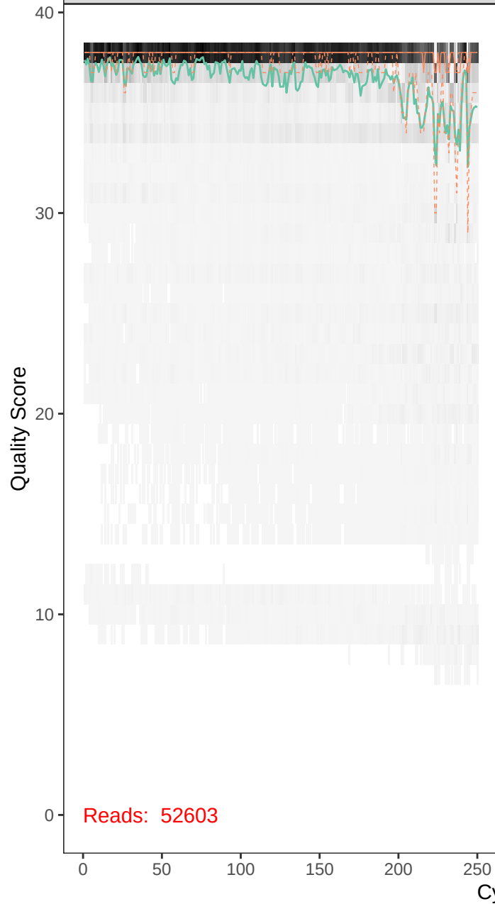
runBE05_FLD0371-r1_F_filt.fastq
