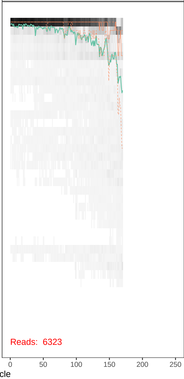
runBE08_F63R44-r1_R_filt.fastq
