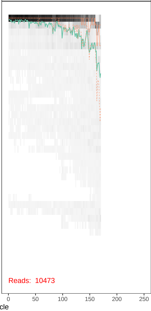
runBE08_F67R42-r1_R_filt.fastq
