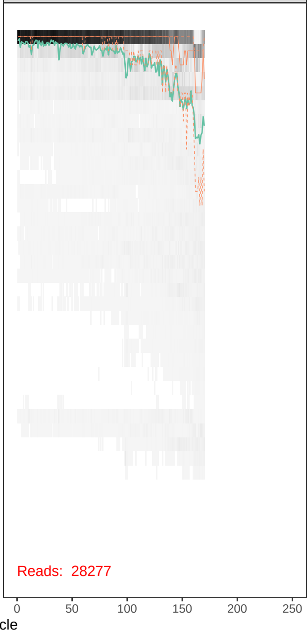
runBE08_F71R50-r1_R_filt.fastq
