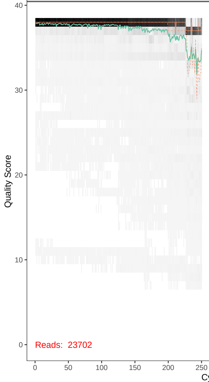
runBE08_F70R51-r1_F_filt.fastq
