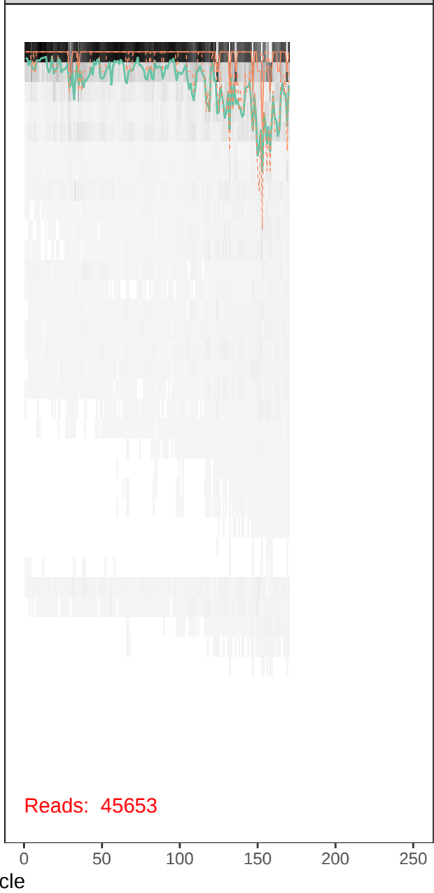
runBE05_FLD0107-r1_R_filt.fastq
