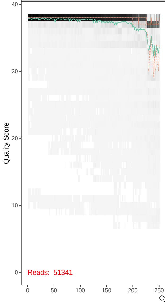
runBE08_F72R41-r1_F_filt.fastq
