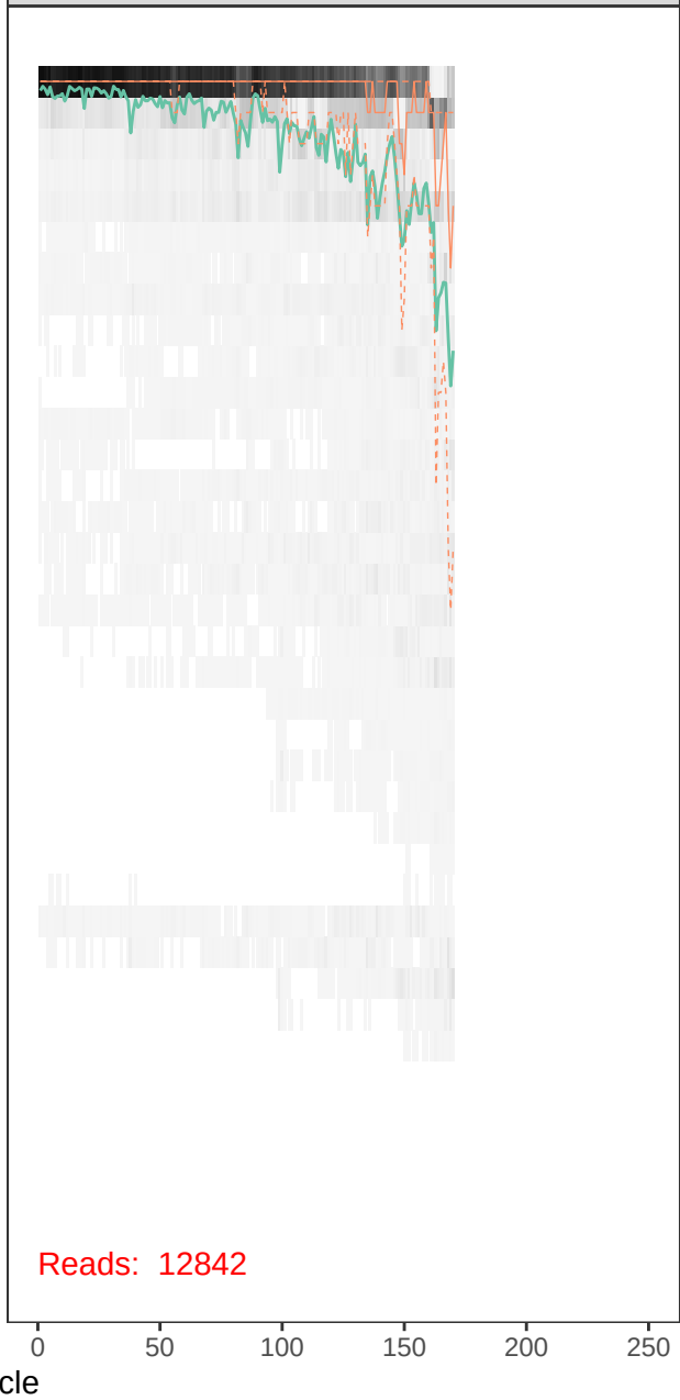
runBE08_F62R50-r1_R_filt.fastq
