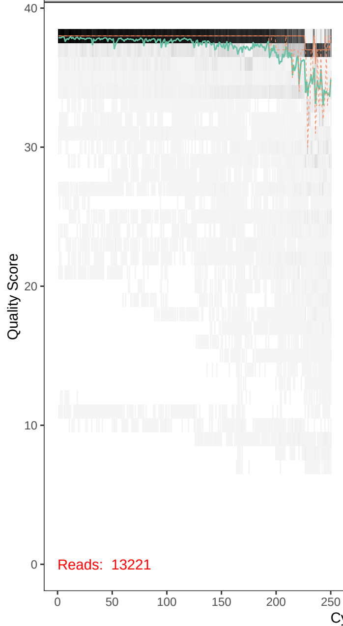
runBE08_F61R44-r1_F_filt.fastq
