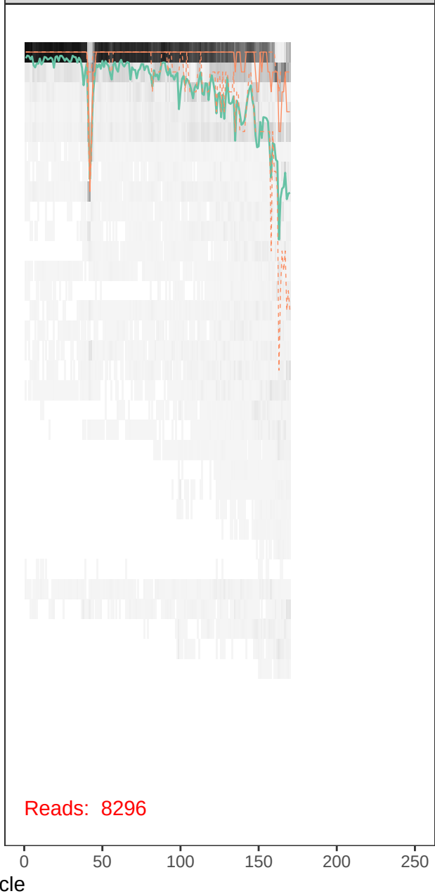
runBE08_F75R44-r1_R_filt.fastq
