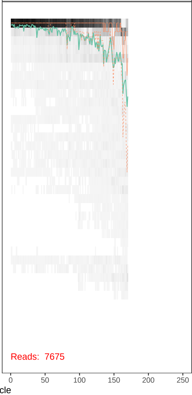
runBE08_F65R50-r1_R_filt.fastq
