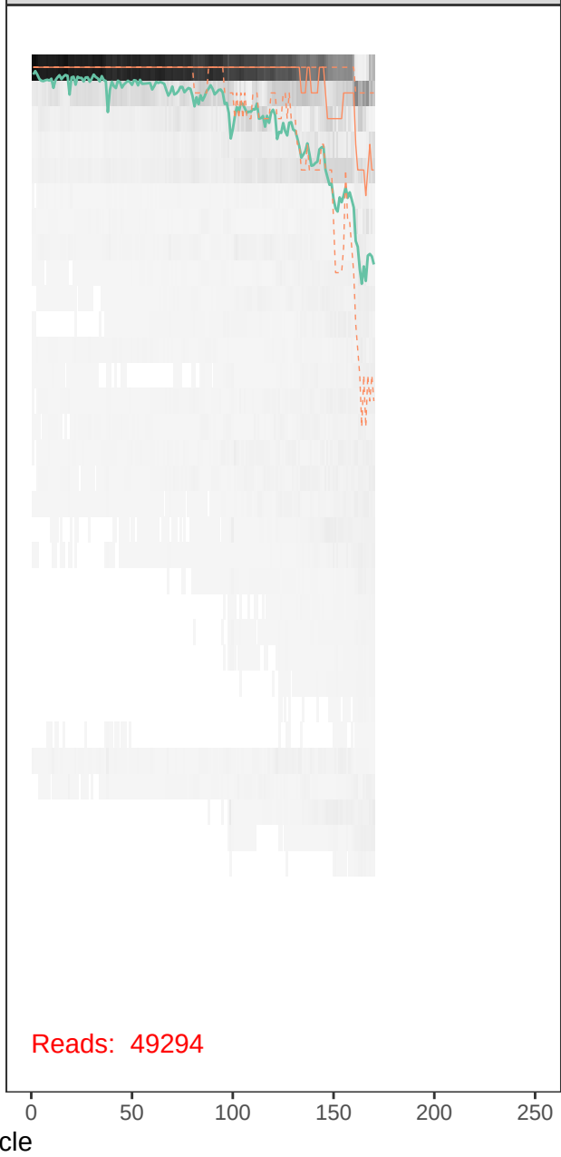
runBE08_F71R53-r1_R_filt.fastq
