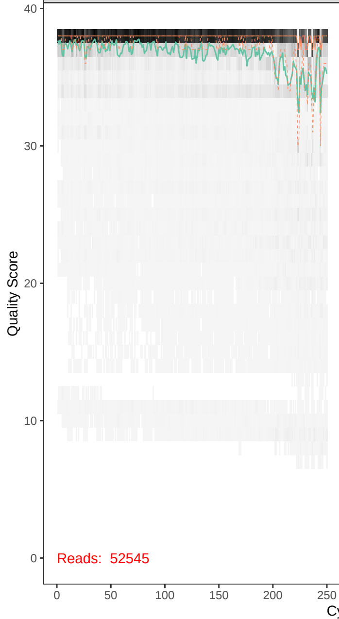
runBE05_FLD0364-r1_F_filt.fastq
