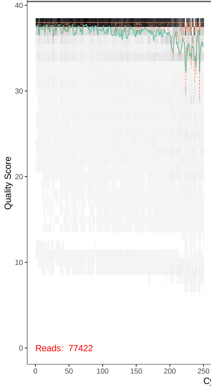
runBE05_FLD0351-r1_F_filt.fastq
