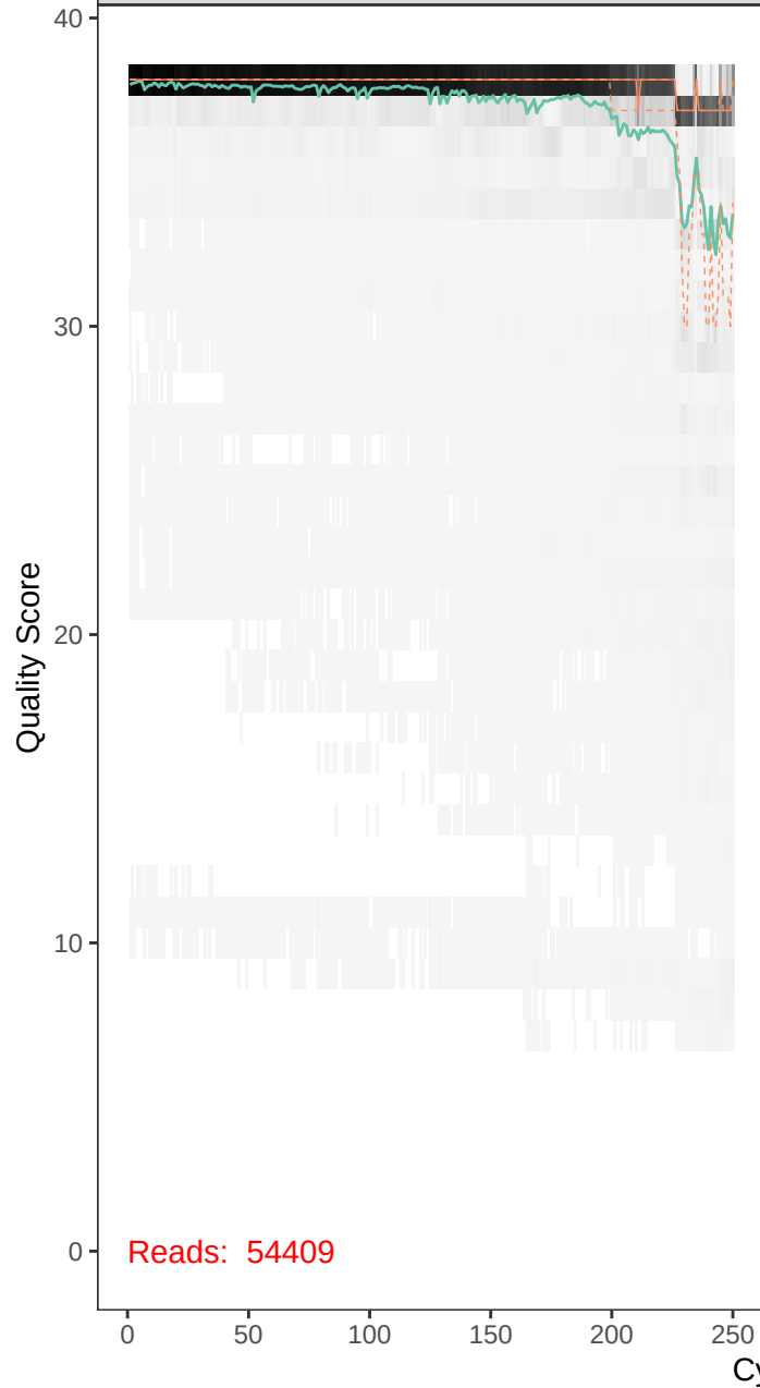
runBE08_F71R41-r1_F_filt.fastq
