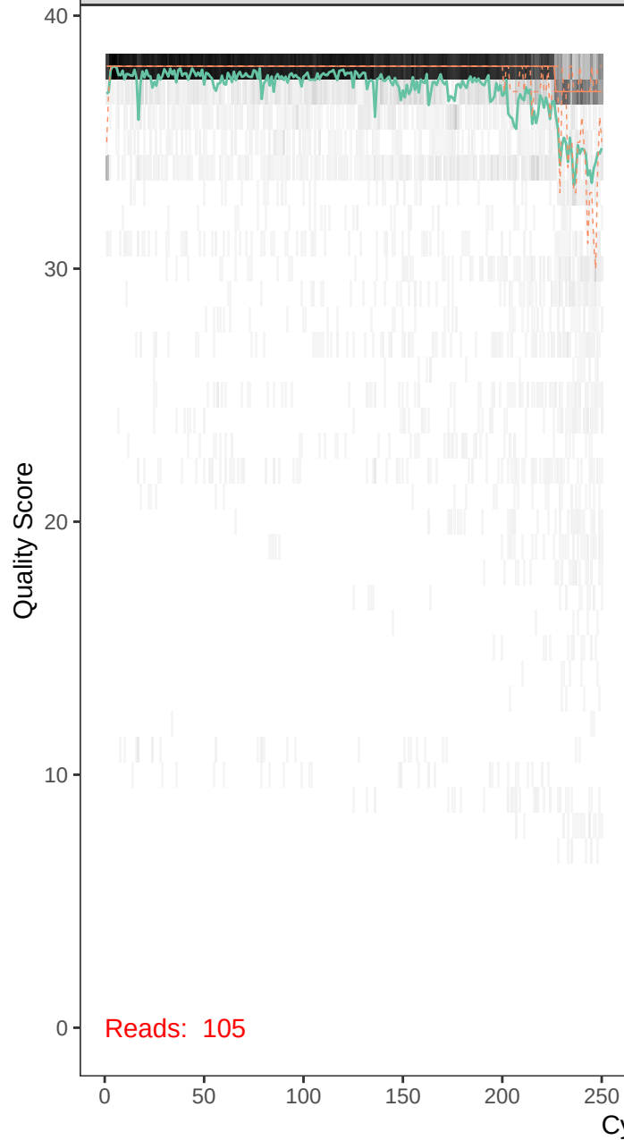
runBE08_F63R46-r1_F_filt.fastq
