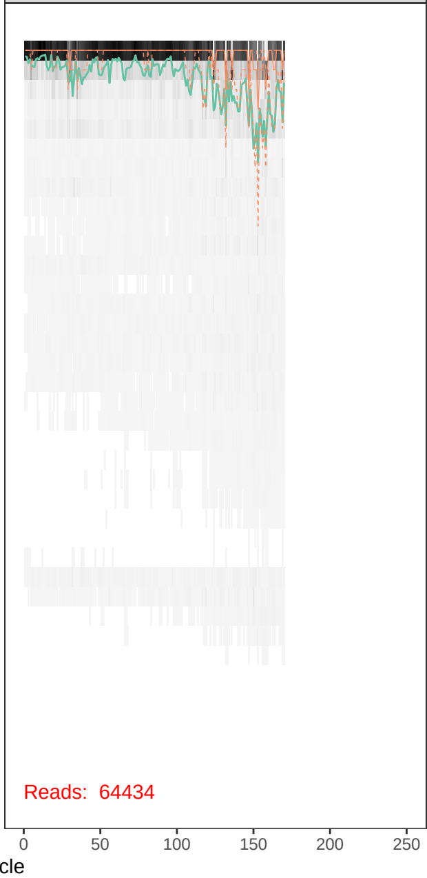
runBE05_FLD0016-r1_R_filt.fastq
