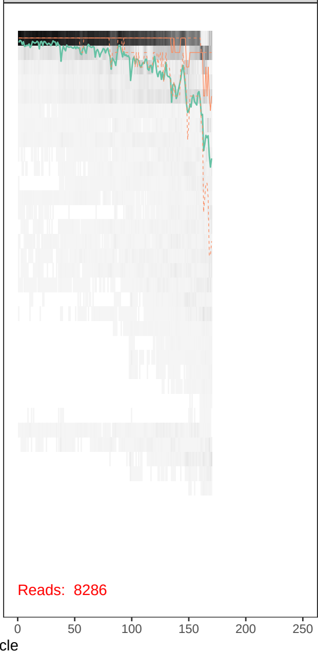
runBE08_F65R43-r1_R_filt.fastq
