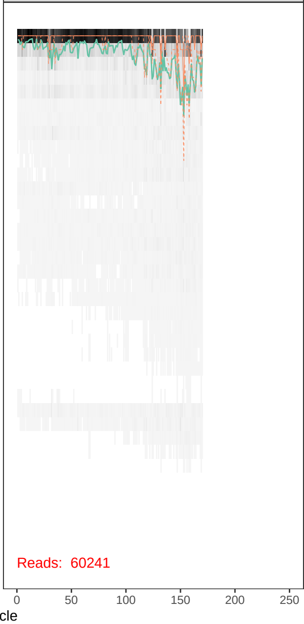
runBE05_FLD0374-r1_R_filt.fastq
