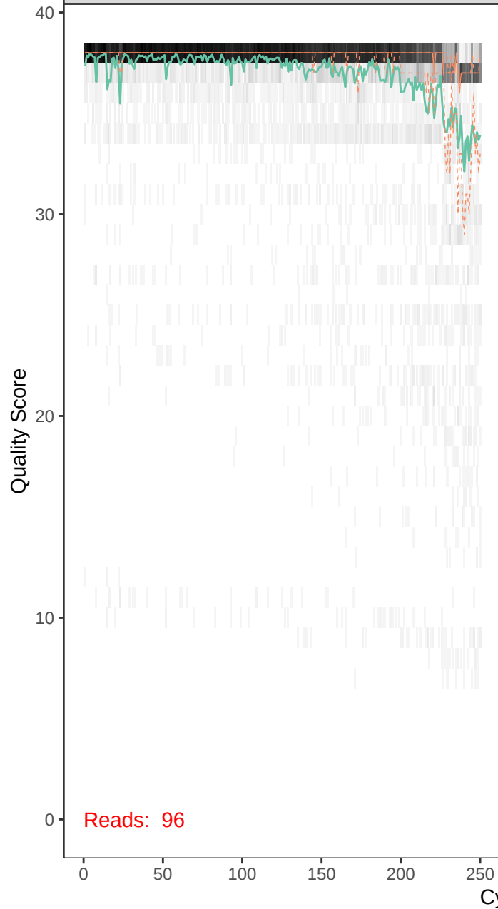
runBE08_F66R51-r1_F_filt.fastq
