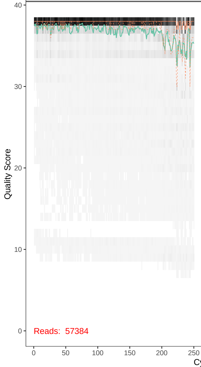
runBE05_FLD0071-r1_F_filt.fastq
