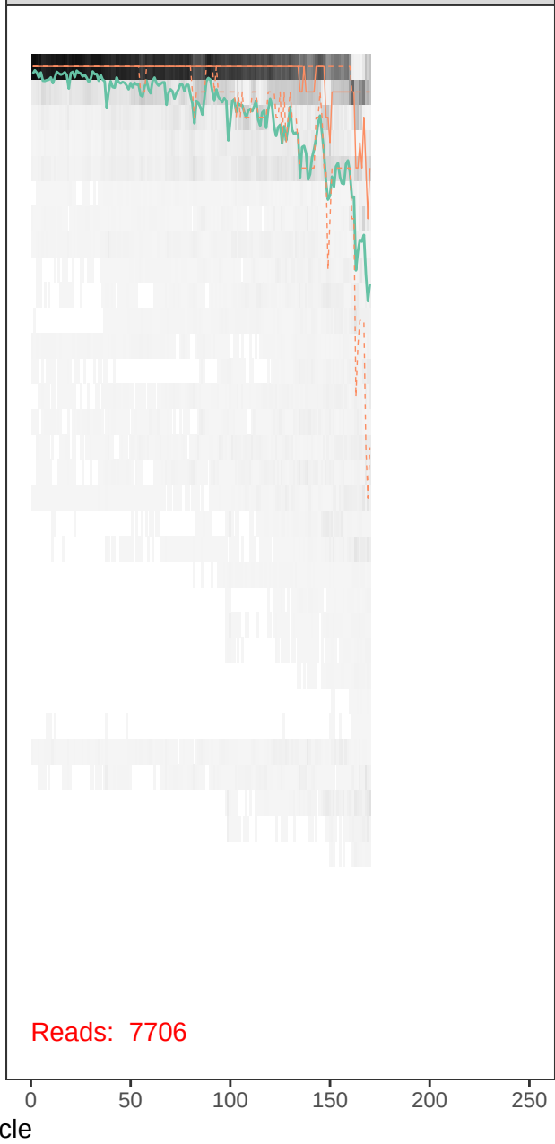
runBE08_F62R46-r1_R_filt.fastq
