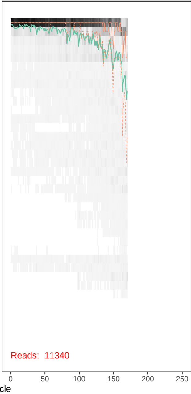
runBE08_F65R48-r1_R_filt.fastq
