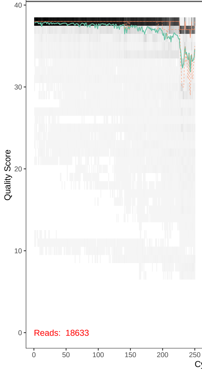
runBE08_F68R51-r1_F_filt.fastq
