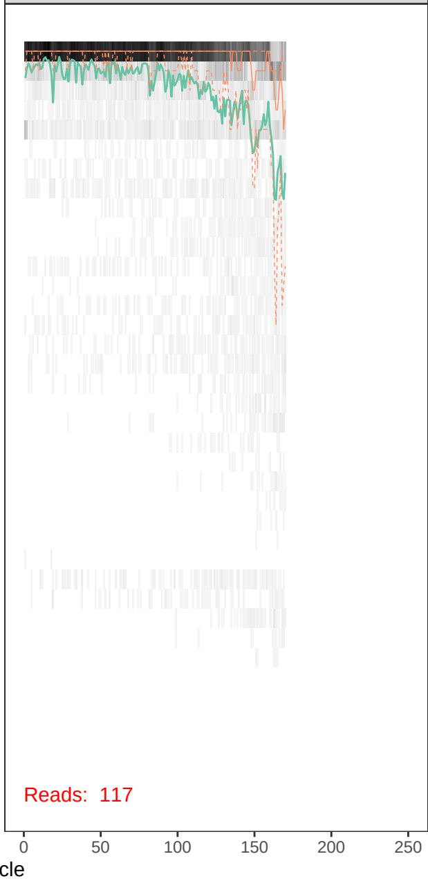
runBE08_F69R47-r1_R_filt.fastq
