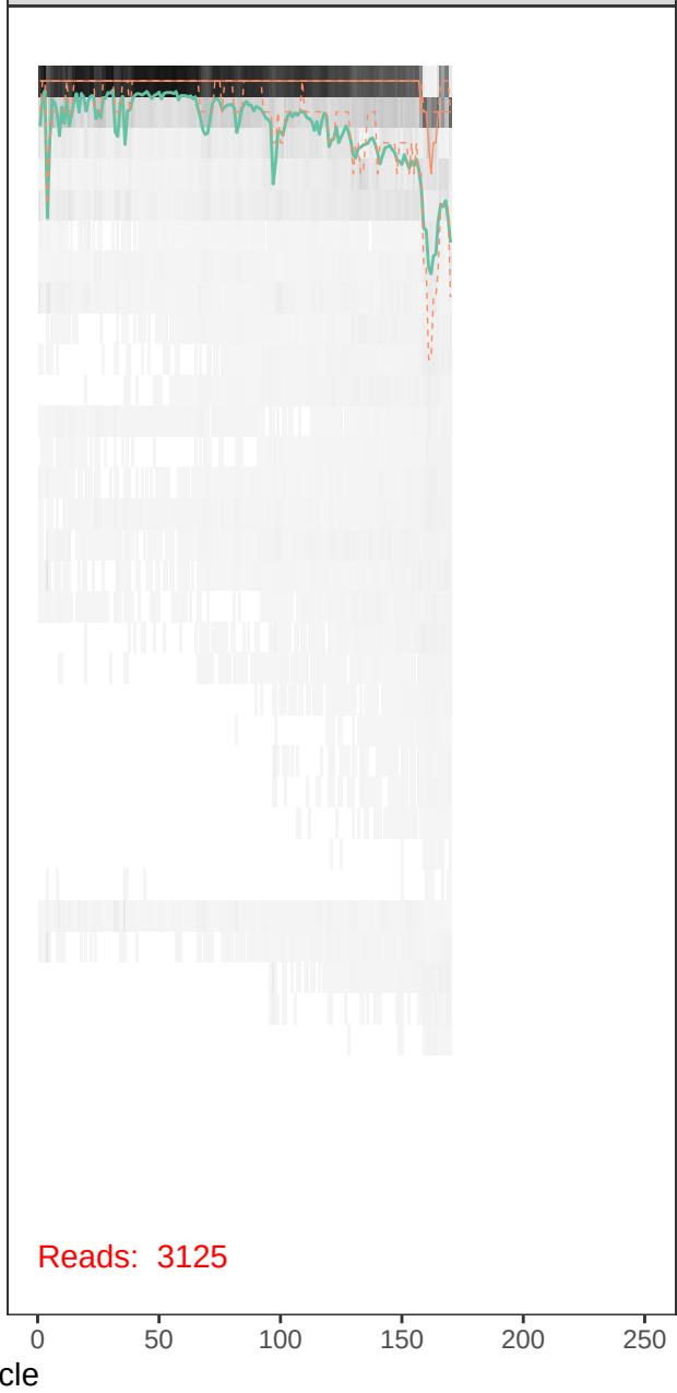
runBE08_F2R1-r1_R_filt.fastq
