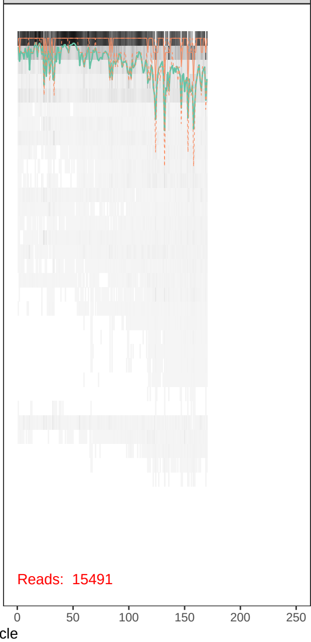
runBE05_FLD0264-r1_R_filt.fastq
