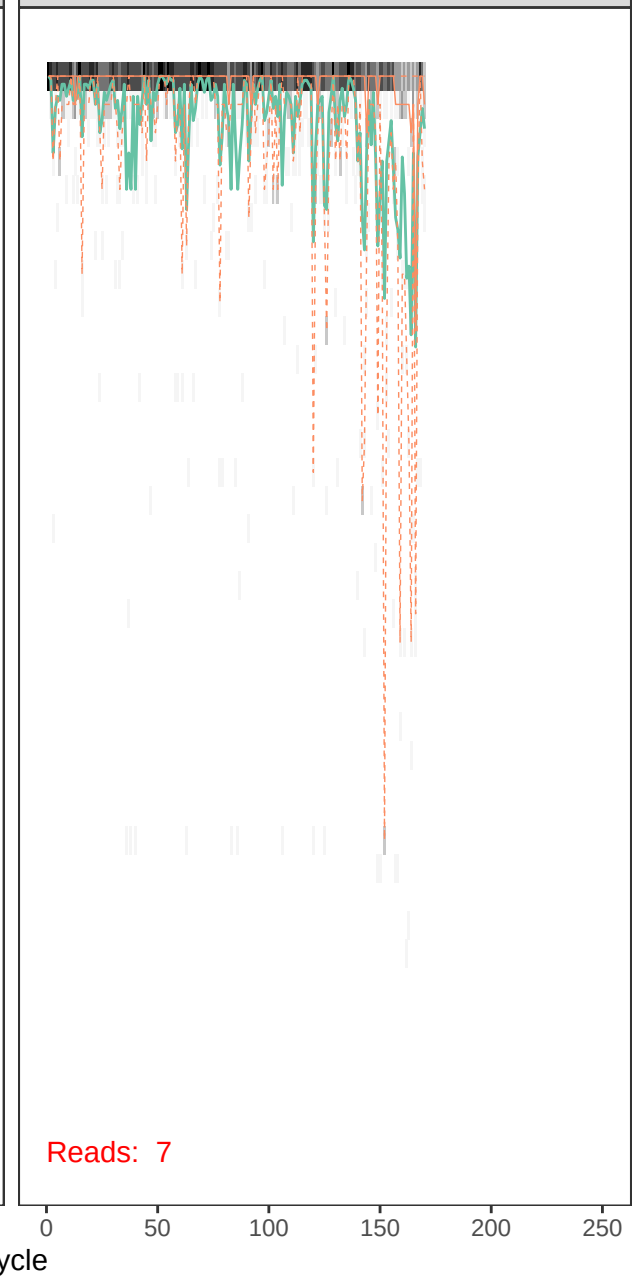
runBE08_F3R8-r1_R_filt.fastq
