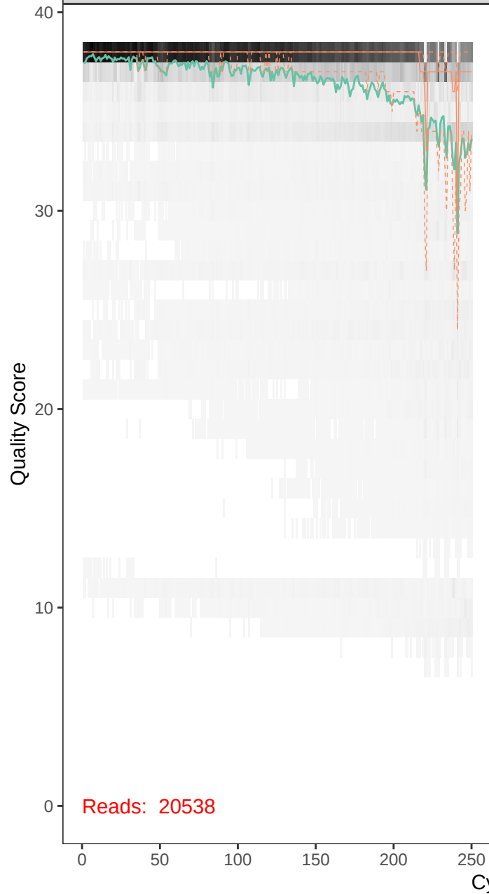
runBE05_FLD0195-r1_F_filt.fastq
