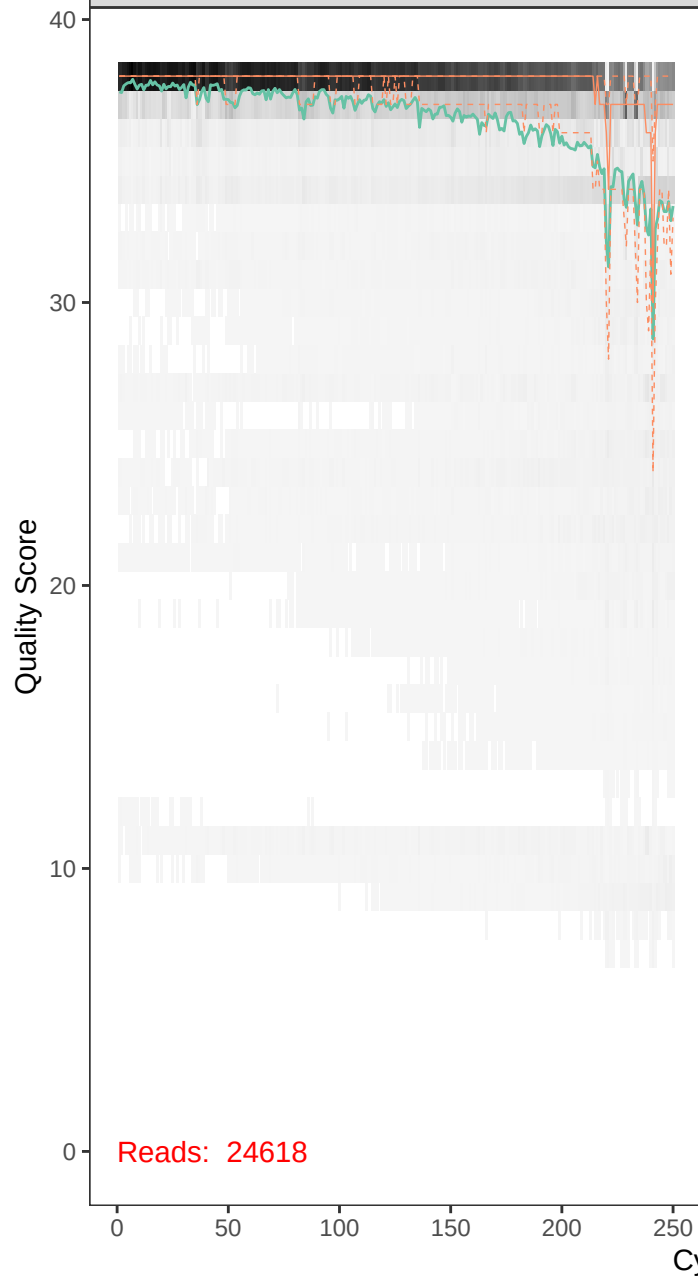
runBE05_FLD0270-r1_F_filt.fastq
