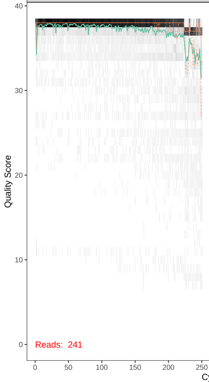
runBE08_F9R6-r1_F_filt.fastq
