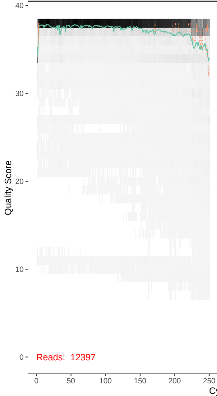
runBE08_F10R11-r1_F_filt.fastq
