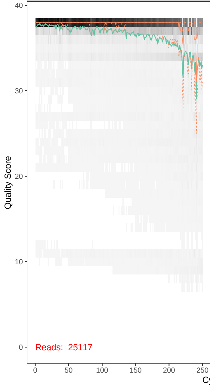
runBE05_FLD0323-r1_F_filt.fastq
