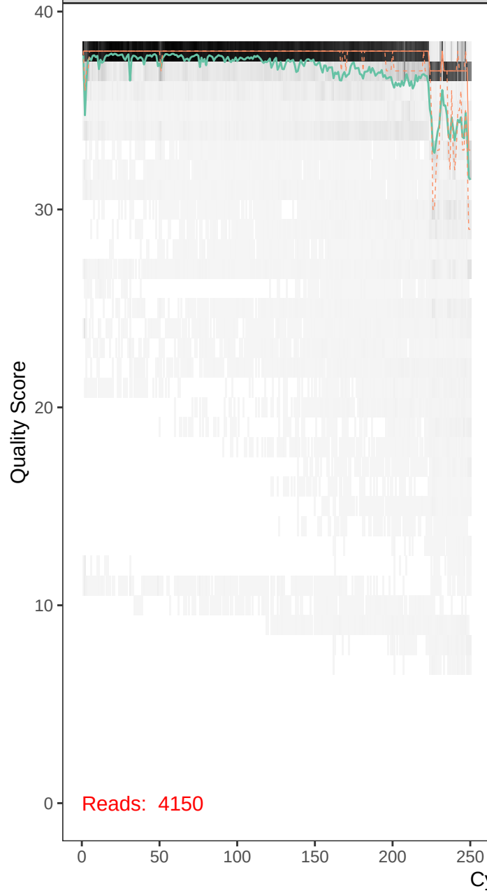
runBE08_F5R6-r1_F_filt.fastq
