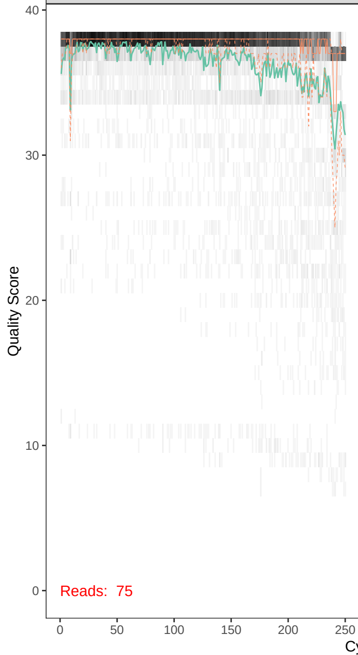
runBE08_F6R6-r1_F_filt.fastq
