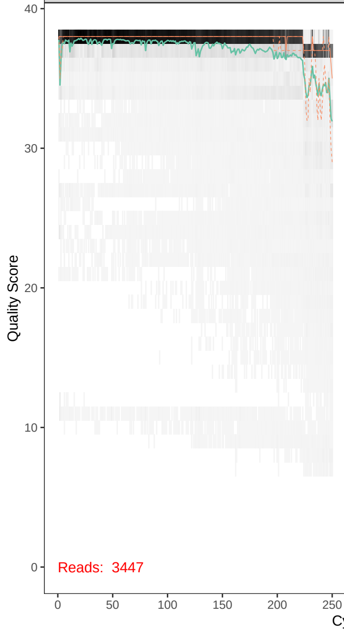
runBE08_F10R5-r1_F_filt.fastq
