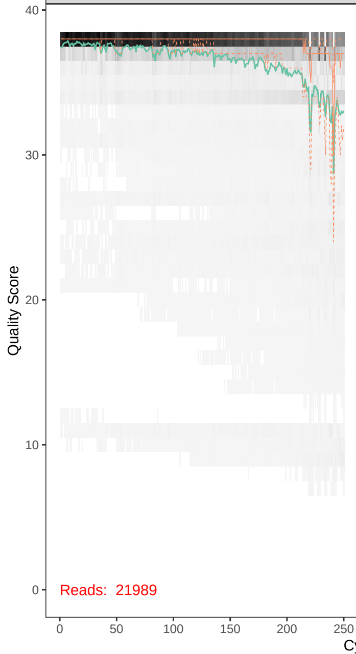
runBE05_FLD0283-r1_F_filt.fastq
