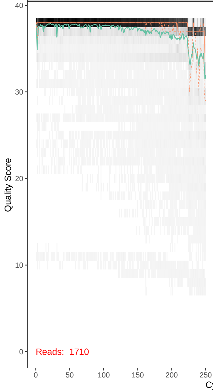
runBE08_F10R10-r1_F_filt.fastq
