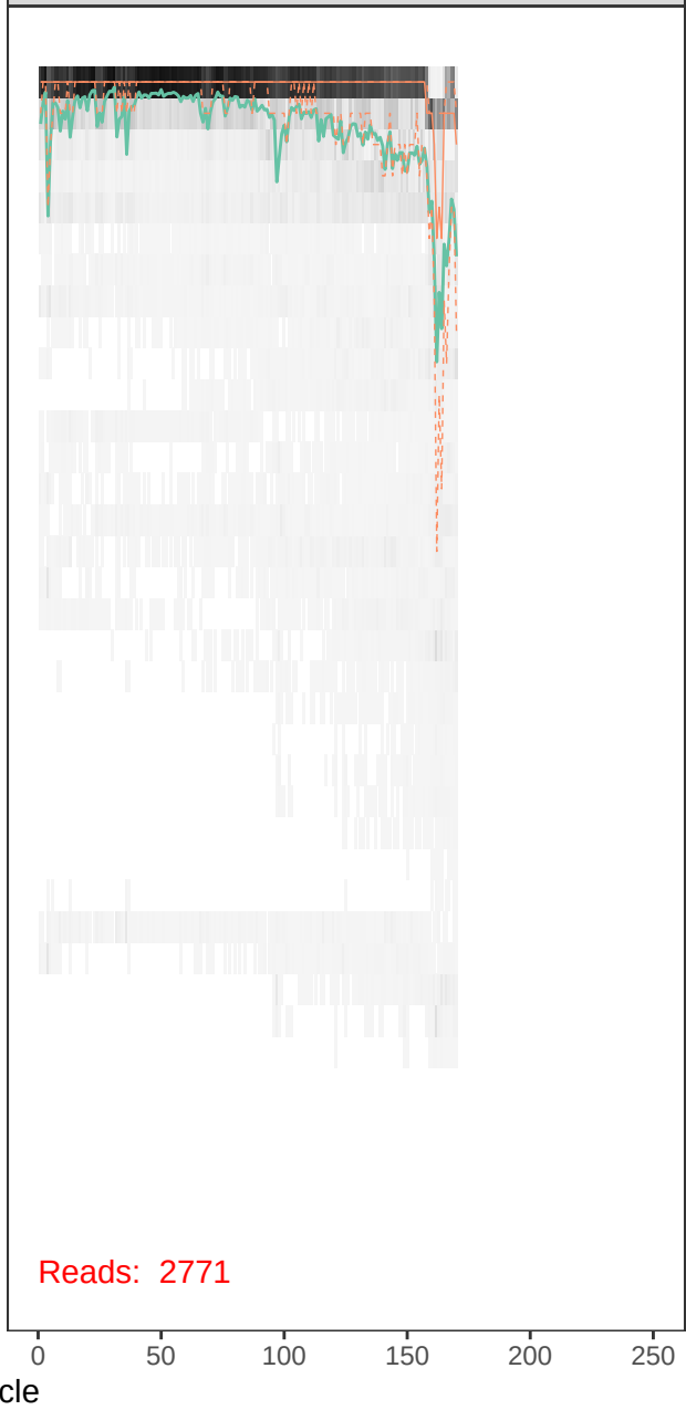
runBE08_F10R8-r1_R_filt.fastq
