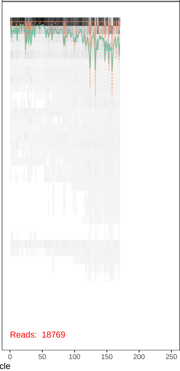
runBE05_FLD0256-r1_R_filt.fastq
