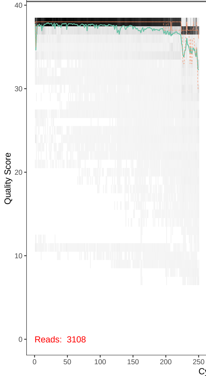
runBE08_F4R1-r1_F_filt.fastq
