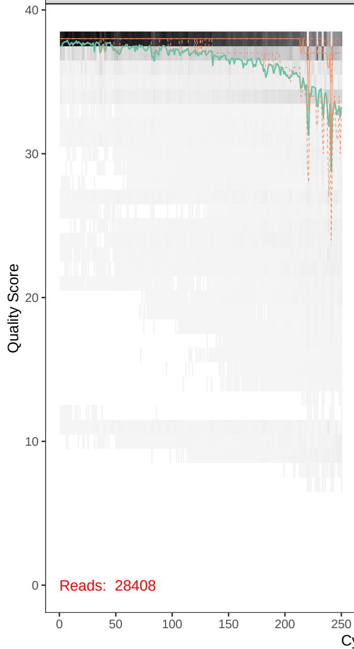
runBE05_FLD0247-r1_F_filt.fastq
