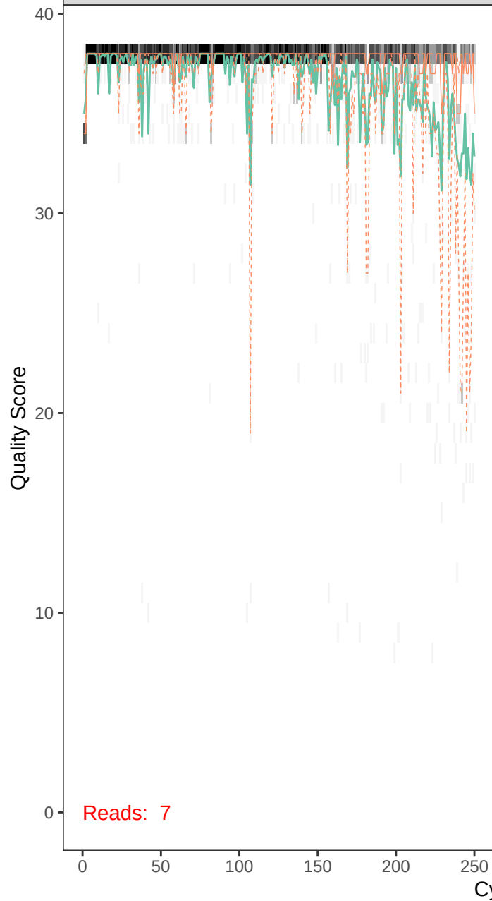
runBE08_F4R9-r1_F_filt.fastq
