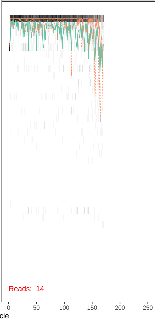
runBE08_F15R6-r1_R_filt.fastq
