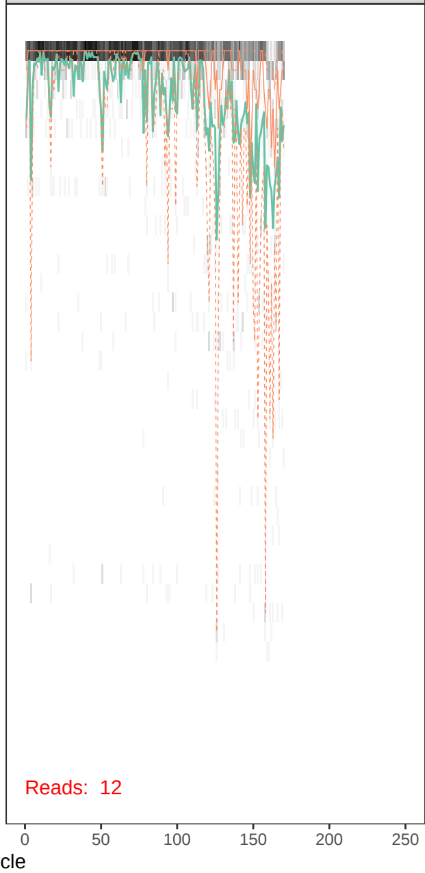
runBE08_F14R3-r1_R_filt.fastq
