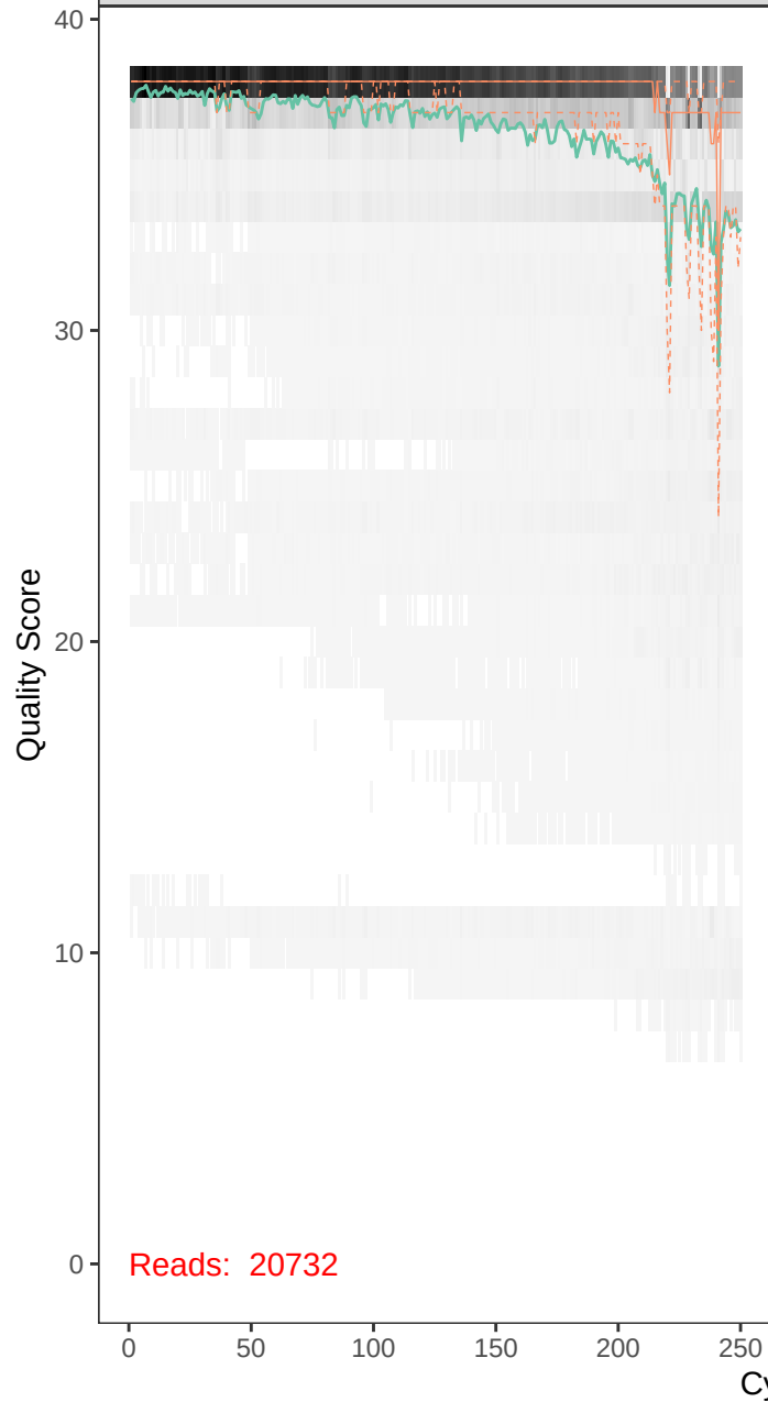
runBE05_FLD0280-r1_F_filt.fastq
