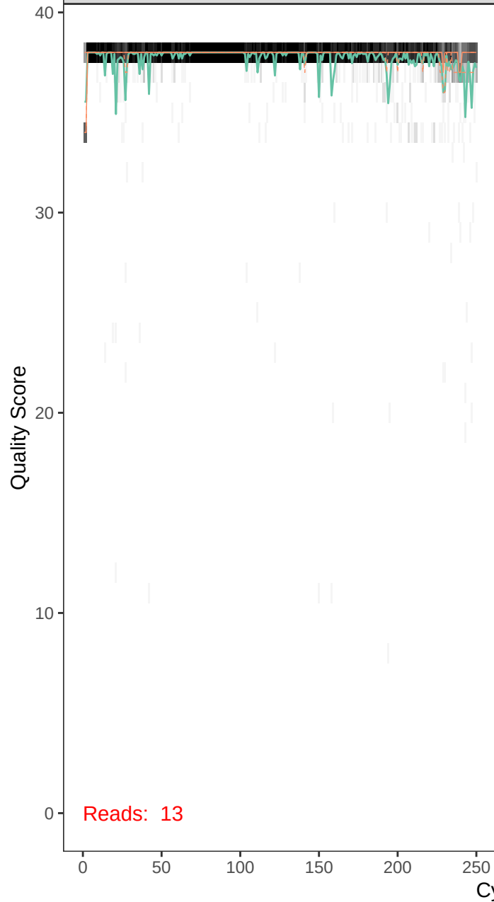
runBE08_F16R7-r1_F_filt.fastq
