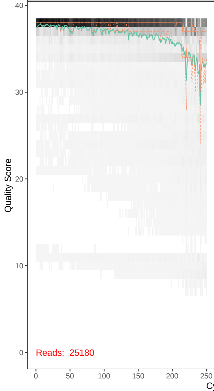
runBE05_FLD0332-r1_F_filt.fastq
