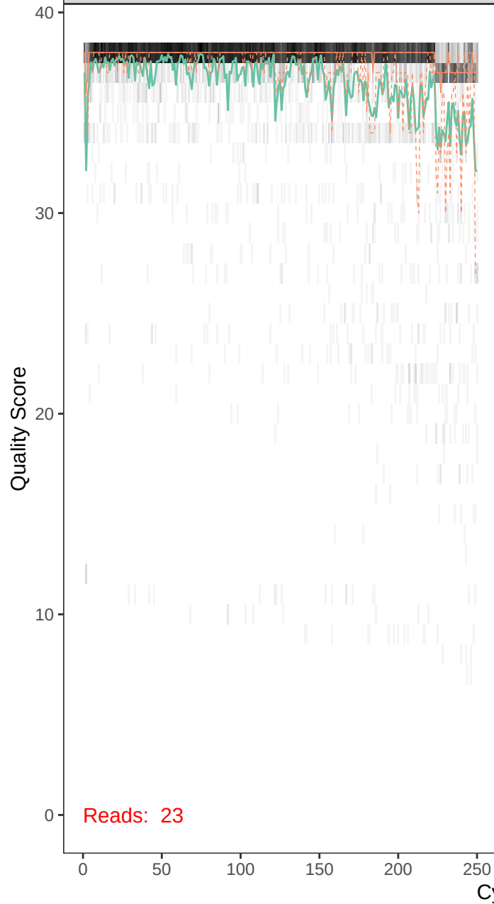
runBE08_F12R3-r1_F_filt.fastq
