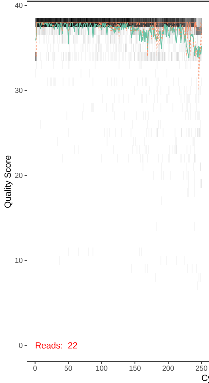
runBE08_F14R6-r1_F_filt.fastq
