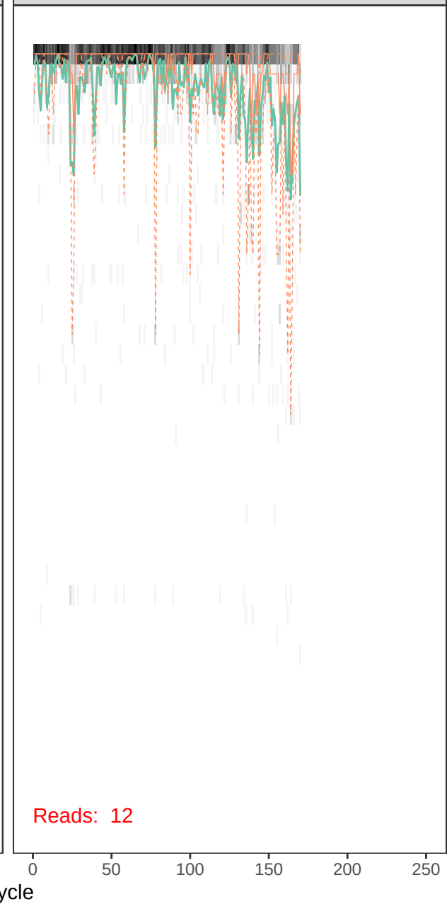
runBE08_F2R8-r1_R_filt.fastq
