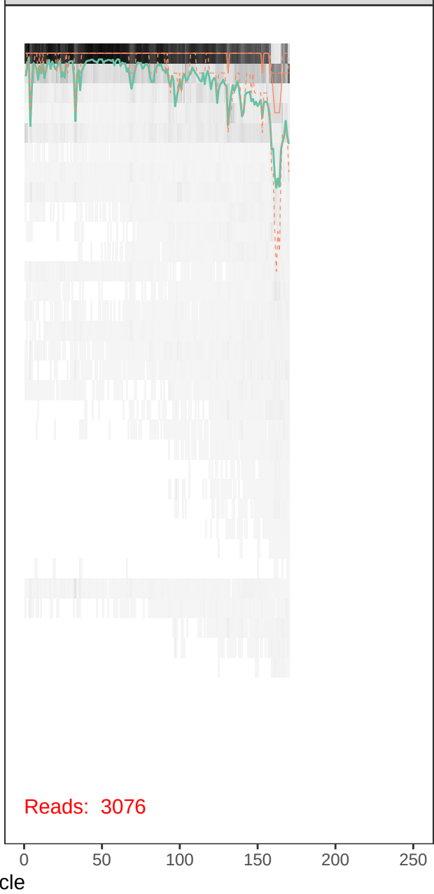
runBE08_F5R1-r1_R_filt.fastq
