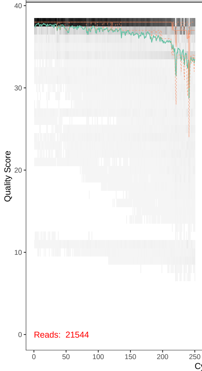
runBE05_FLD0294-r1_F_filt.fastq
