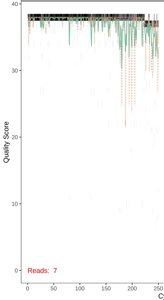
runBE08_F1R8-r1_F_filt.fastq
