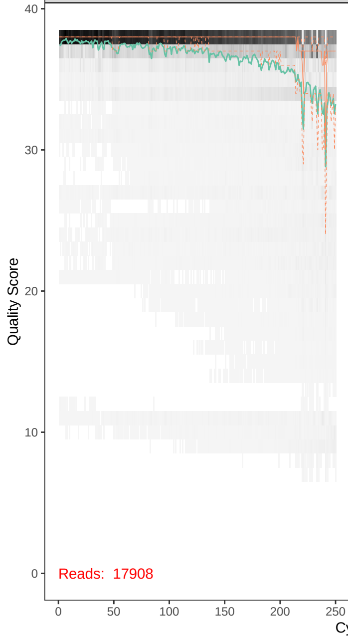
runBE05_FLD0197-r1_F_filt.fastq
