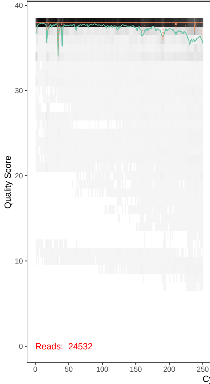
runBE08_F5R11-r1_F_filt.fastq
