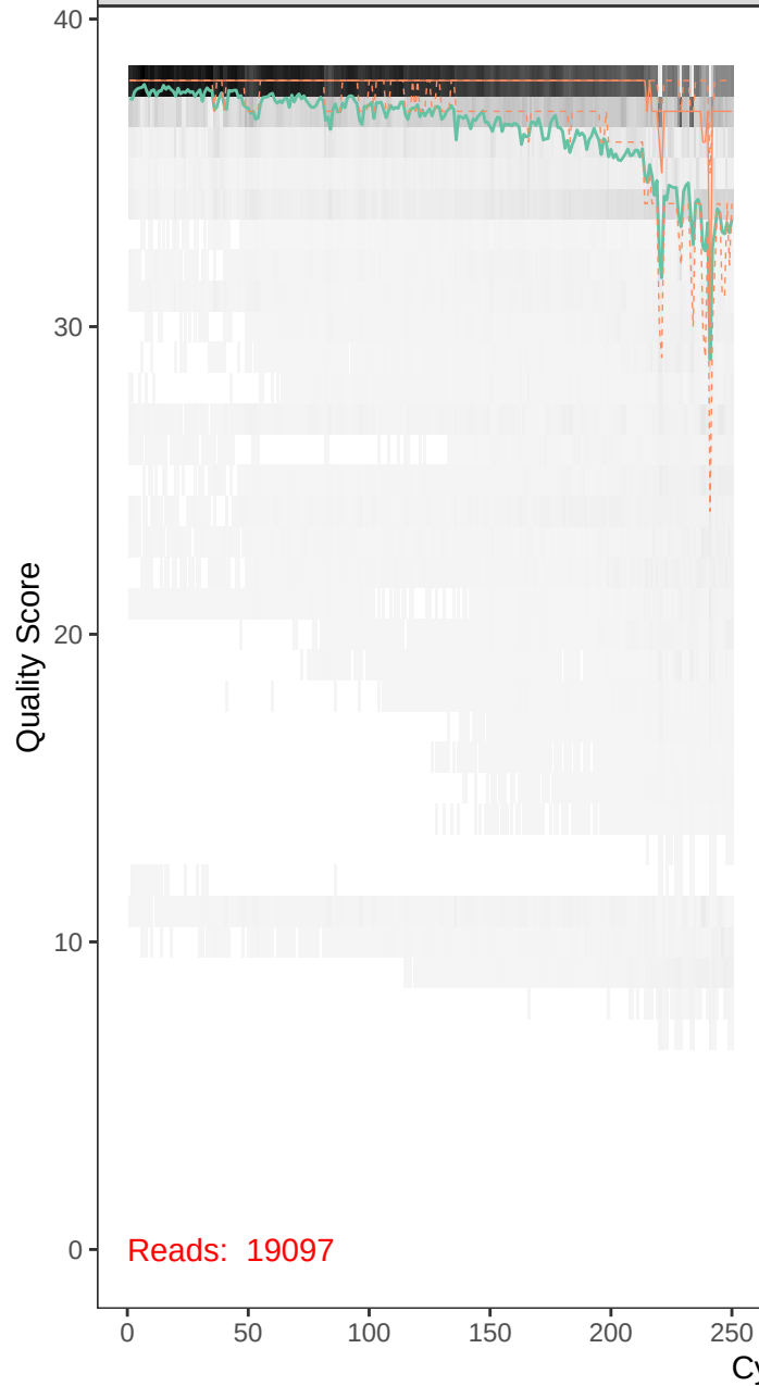
runBE05_FLD0235-r1_F_filt.fastq
