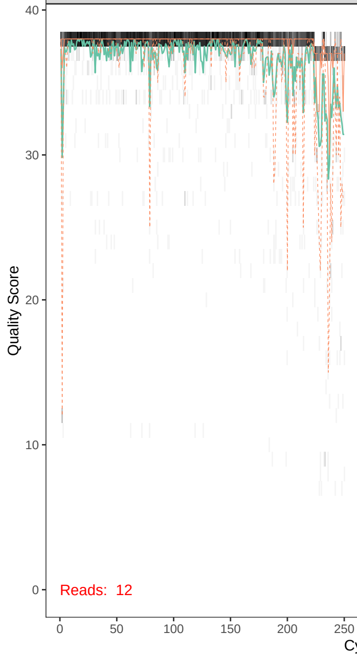
runBE08_F2R8-r1_F_filt.fastq
