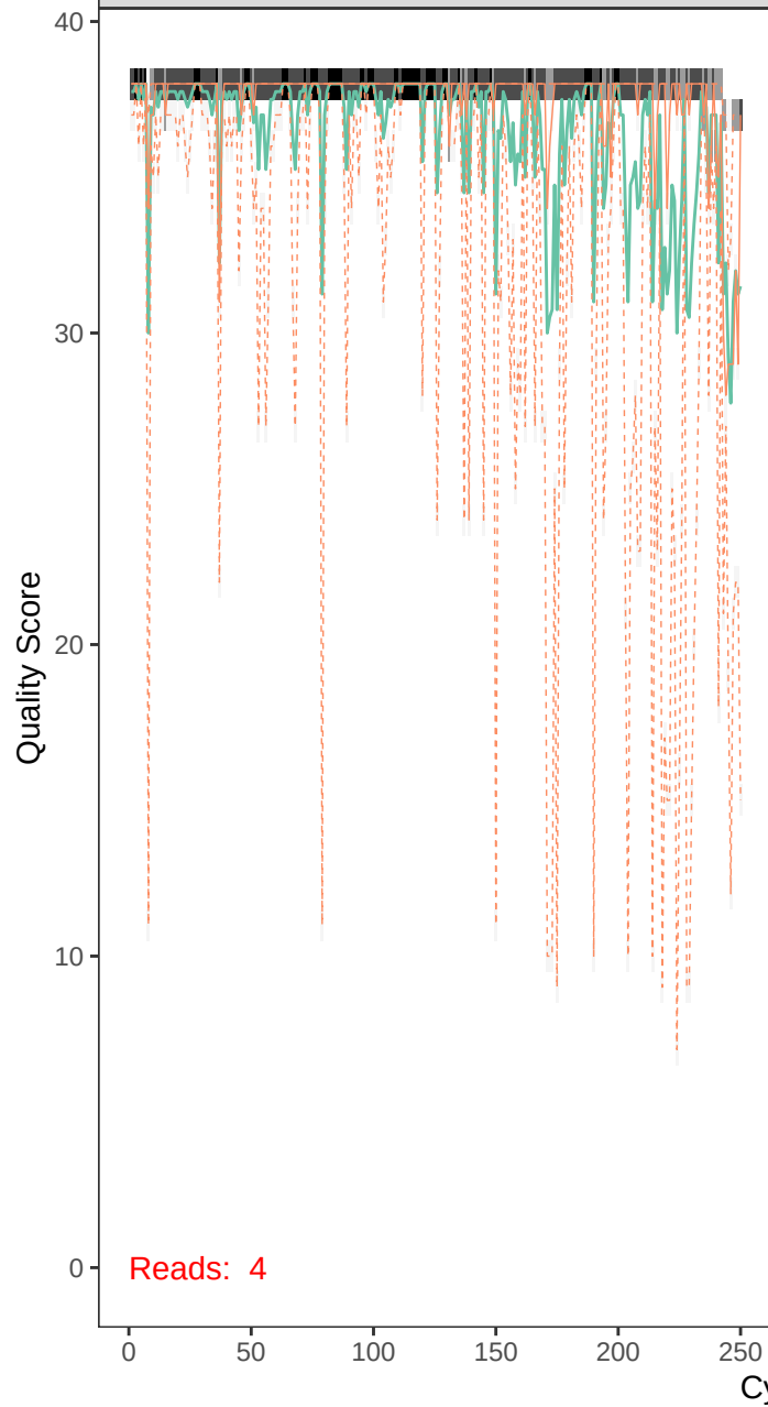
runBE08_F14R8-r1_F_filt.fastq
