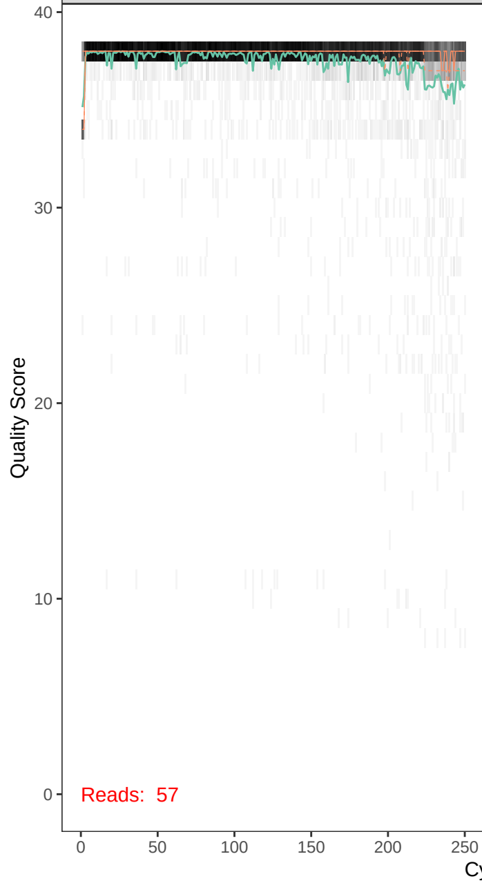
runBE08_F4R7-r1_F_filt.fastq
