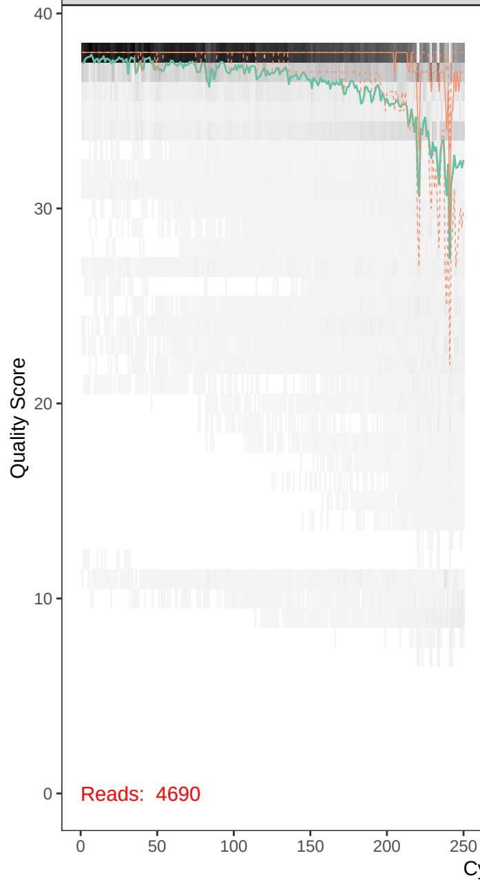
runBE05_FLD0324-r1_F_filt.fastq
