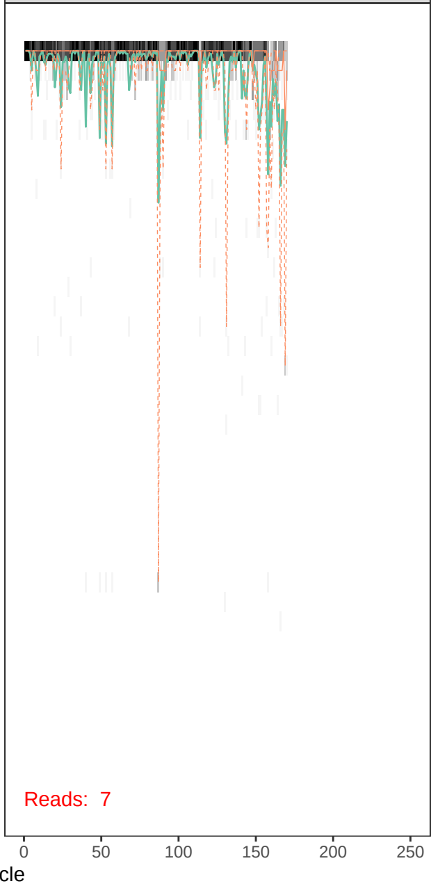
runBE08_F1R8-r1_R_filt.fastq
