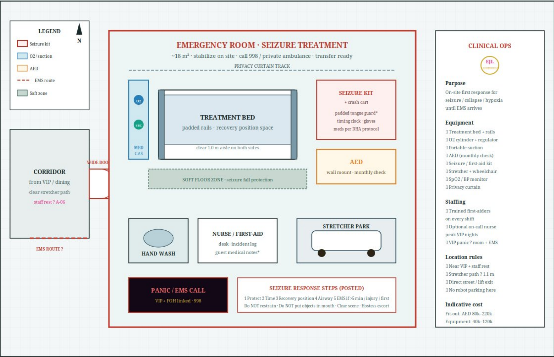
EJL LIGHTHOUSE — ON-SITE EMERGENCY / SEIZURE ROOM First-response medical room · seizure stabilization · AED · oxygen · EMS handoff · staff-trained protocol DRAWING A-05
