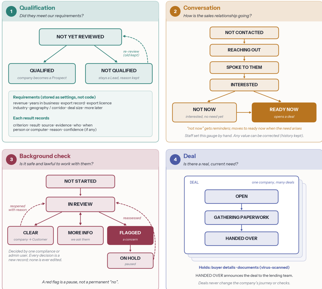
Figure 2. The three gauges and the deal. Dashed arrows are re-reviews and reopenings, which always add a new record.
