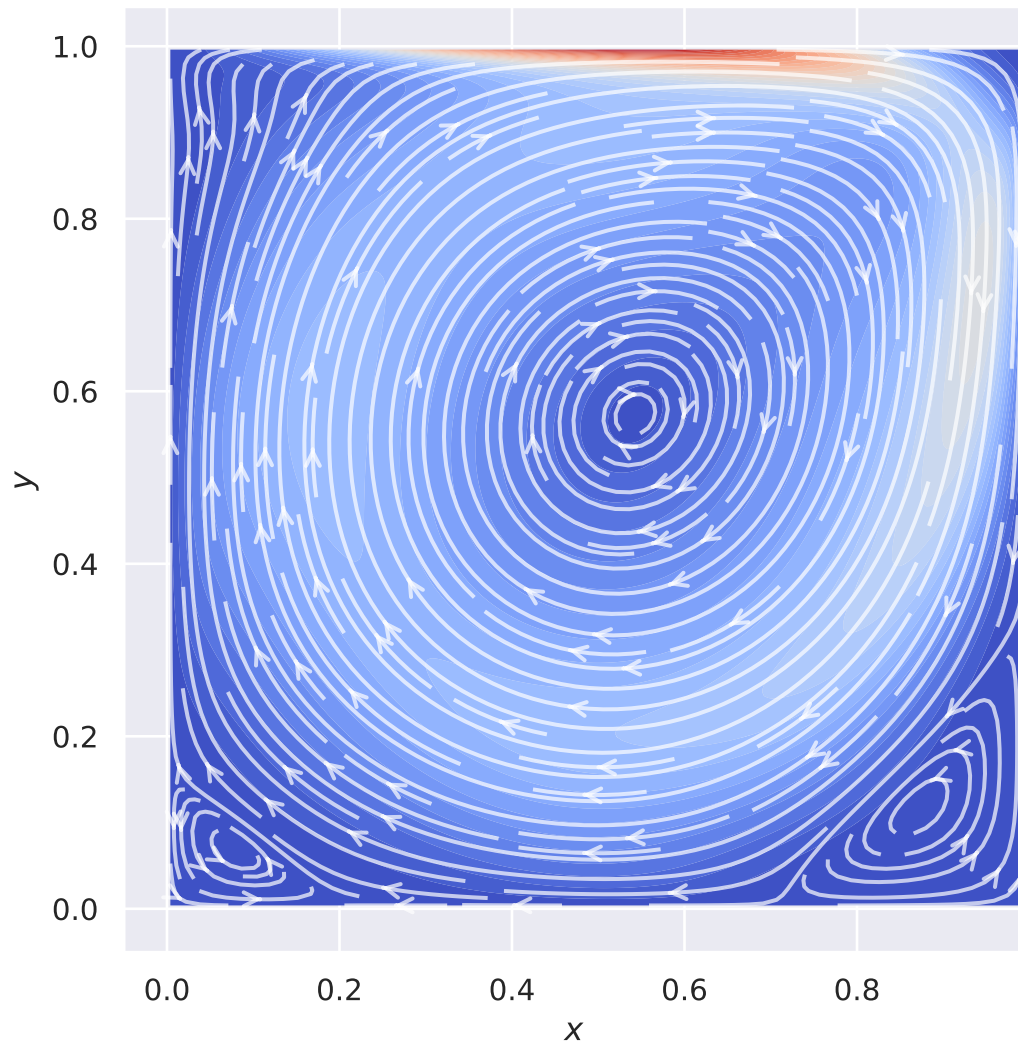
Streamlines: FV, N = 128 , Re = 1000
