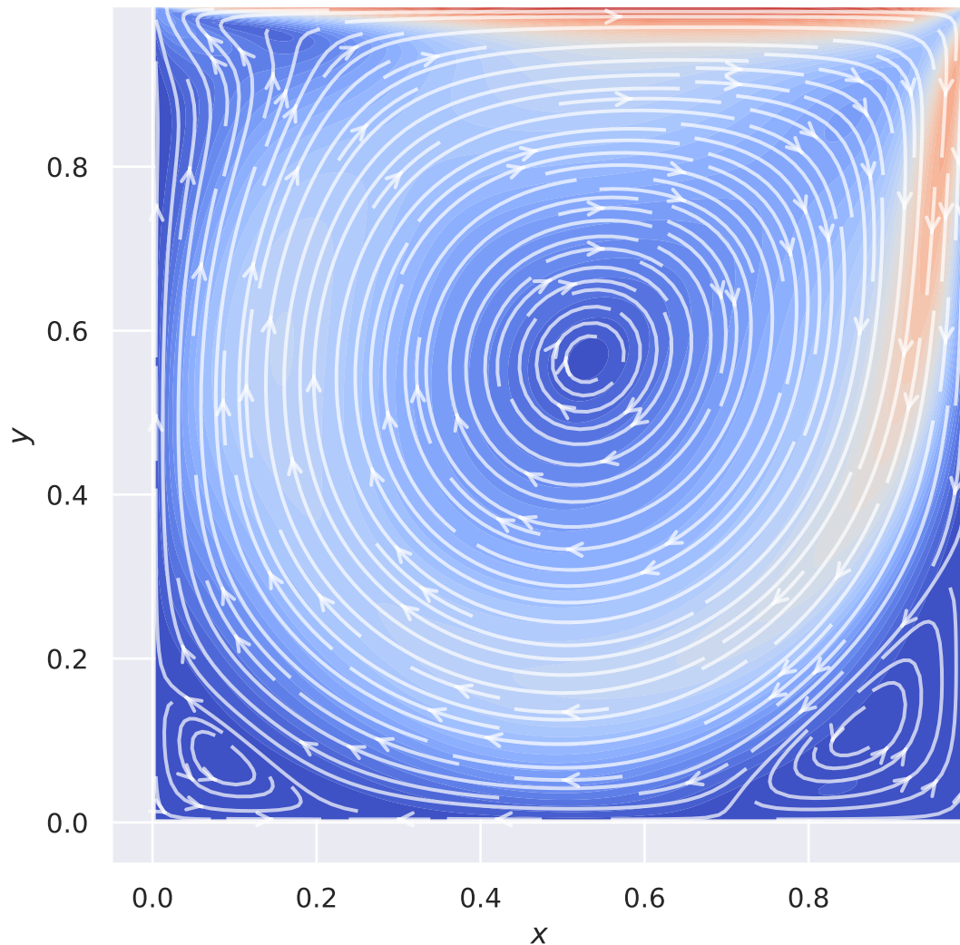
Streamlines: FV, N = 128 , Re = 1000
