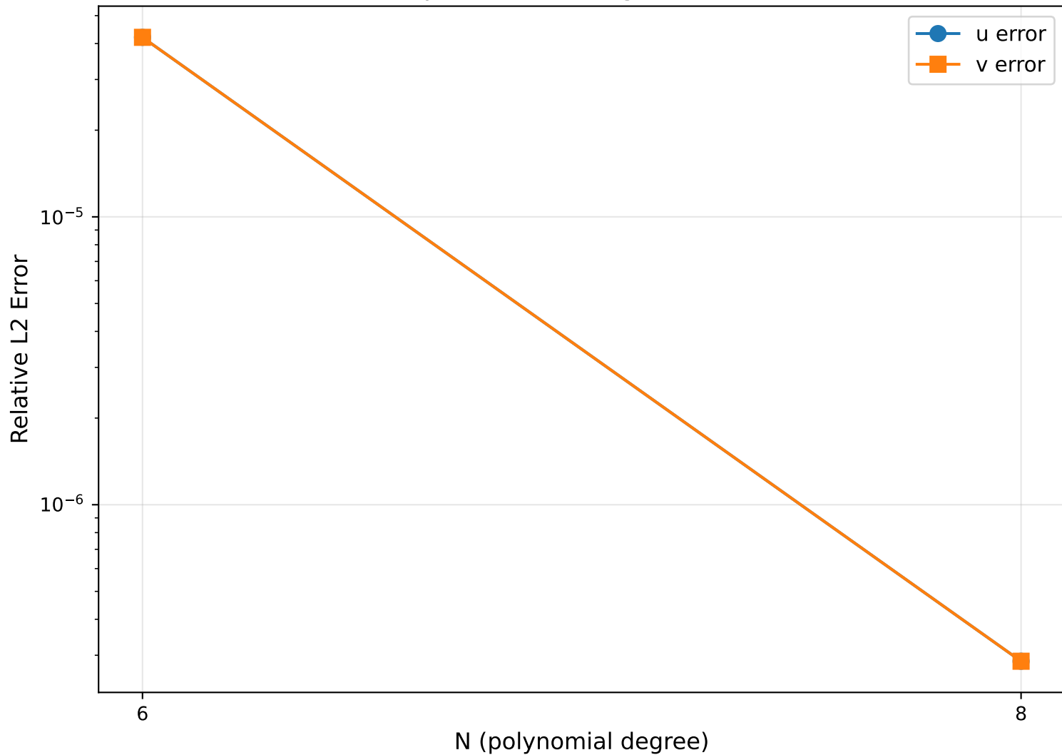
MMS Spectral Convergence (Re=1.0)
