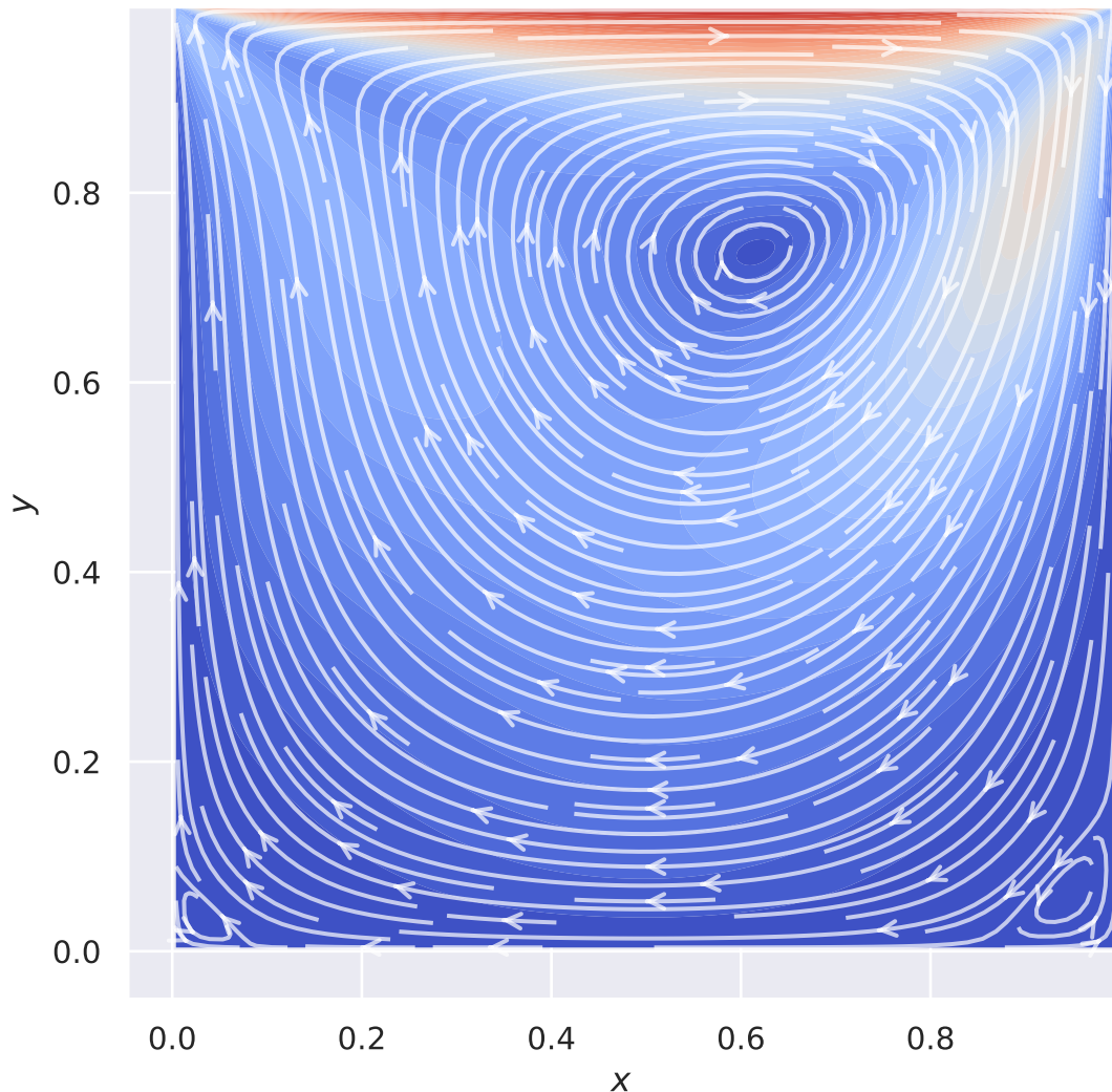
Streamlines: FV, N = 128 , Re = 100
