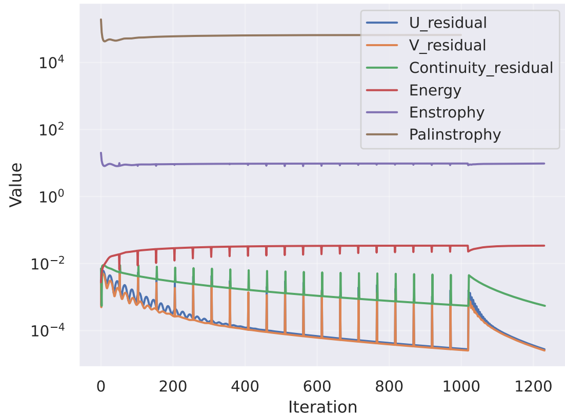
Convergence History --- FV, N = 128 , Re = 100
