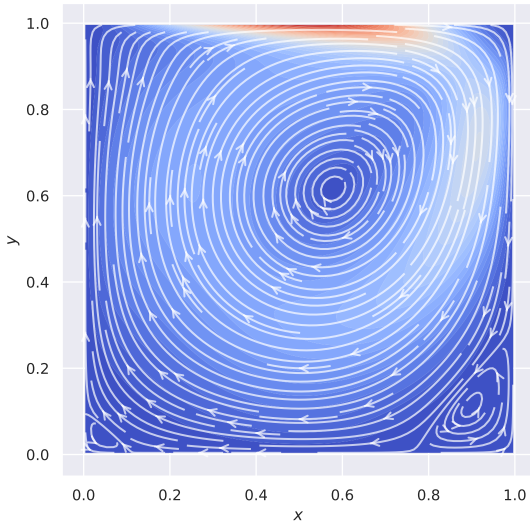
Streamlines: FV, N = 128 , Re = 400
