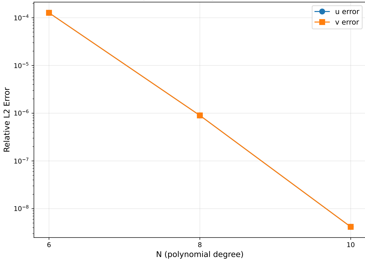
MMS Spectral Convergence (Re=10.0)
