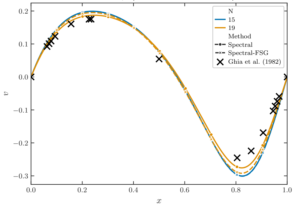
v -velocity (horizontal centerline)
