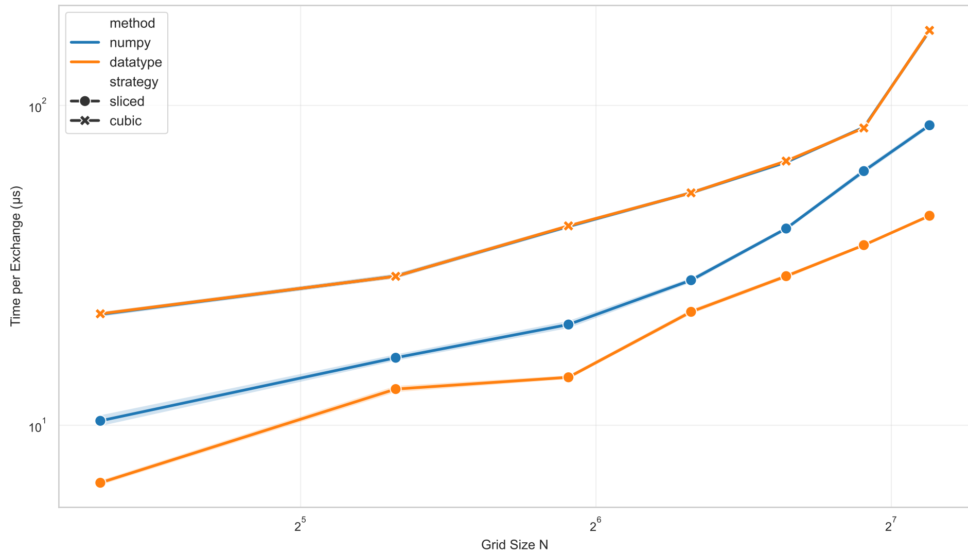
Communication Overhead: Method and Strategy Comparison
