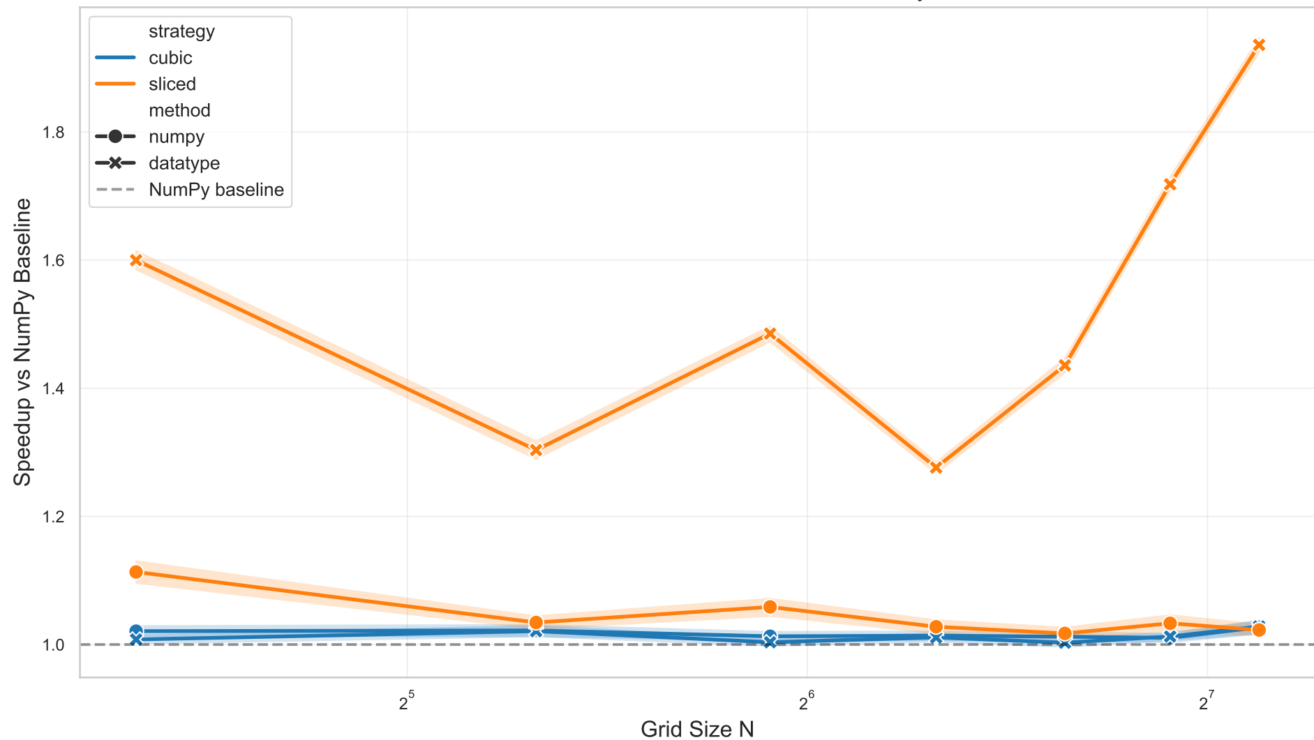
Communication Performance: Normalized to NumPy Baseline
