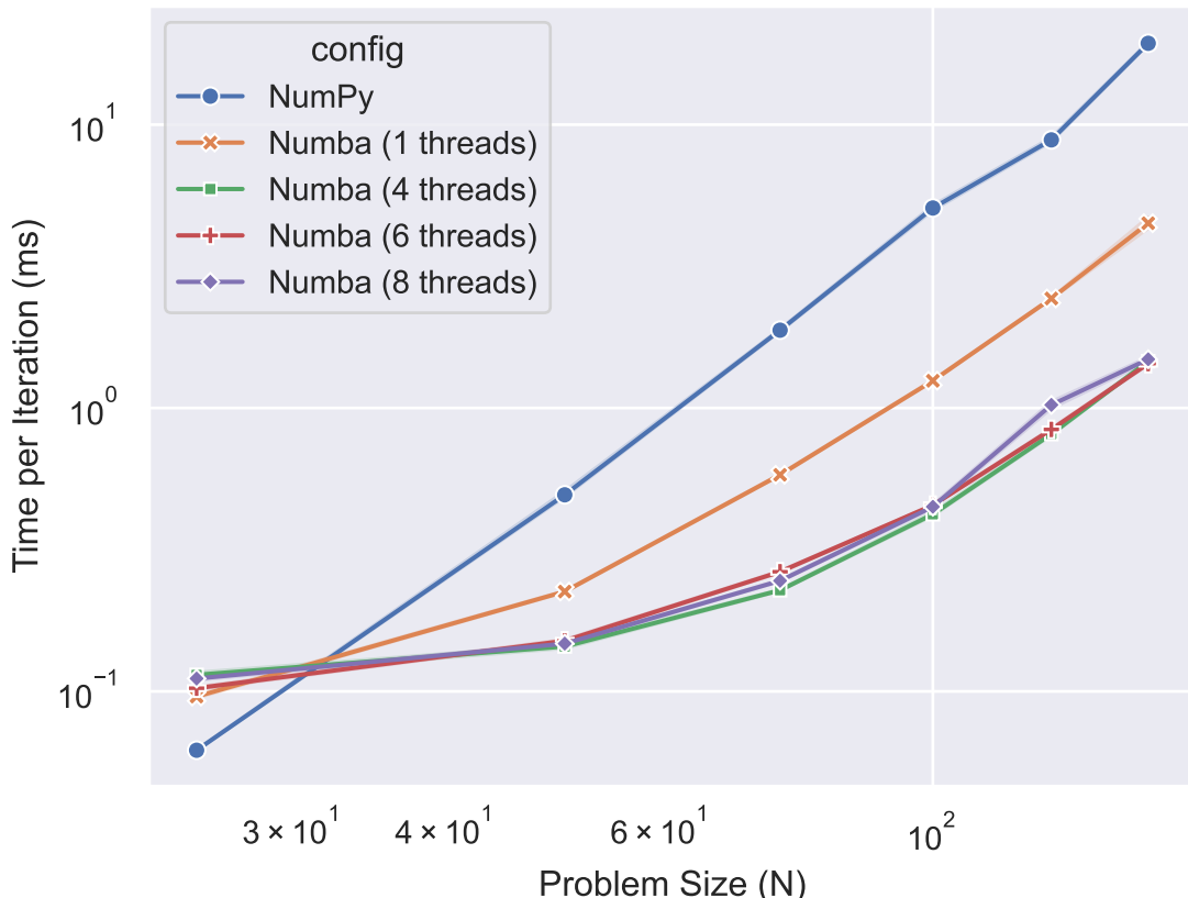
Kernel Performance Comparison
