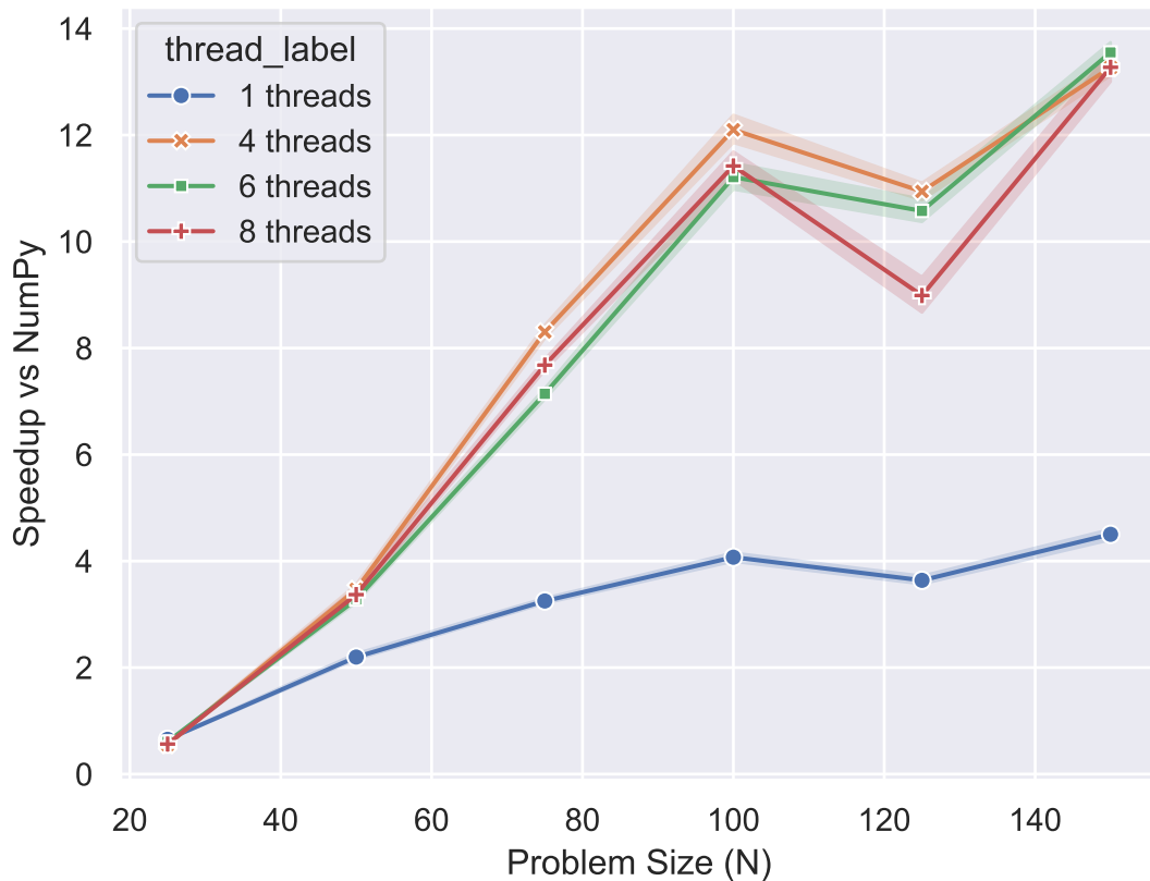
Fixed Iteration Speedup (200 iterations)
