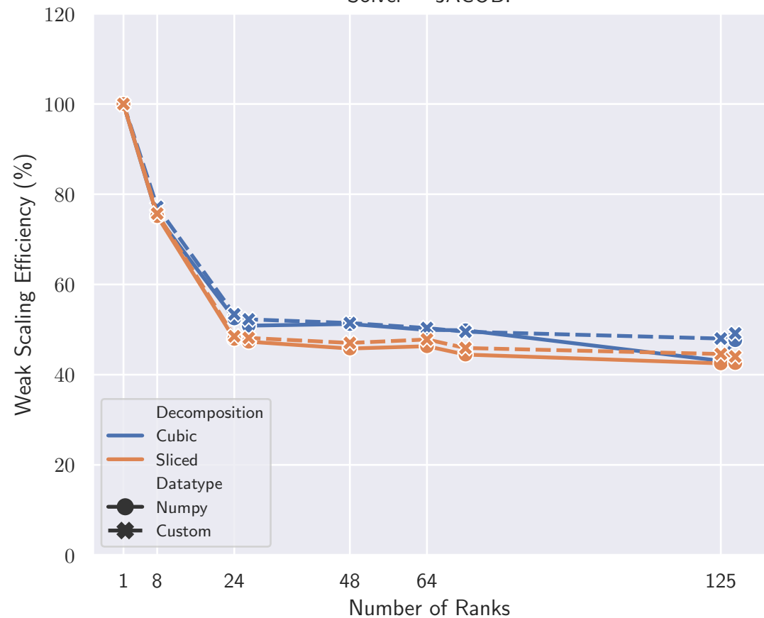
Solver = JACOBI
