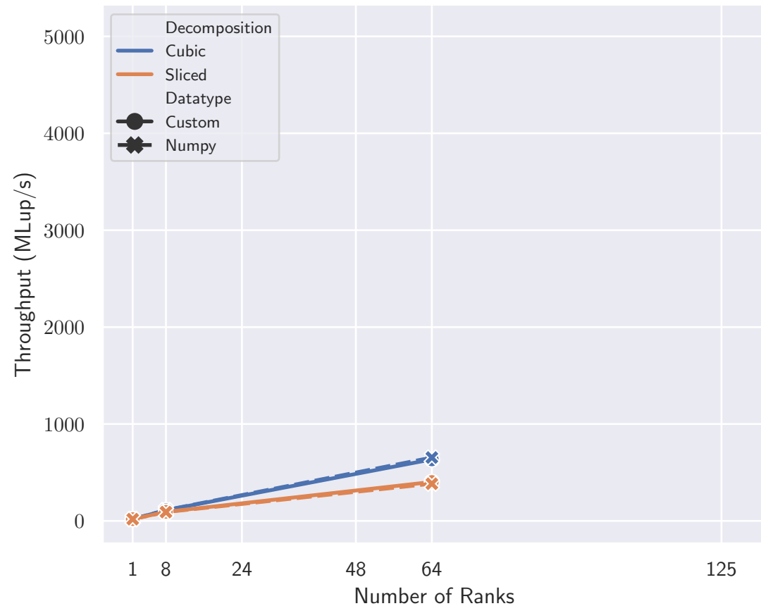
Solver = FMG
