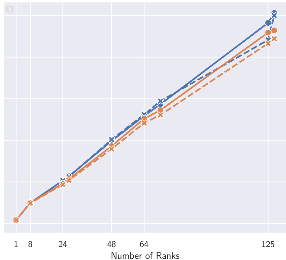
Solver = JACOBI
