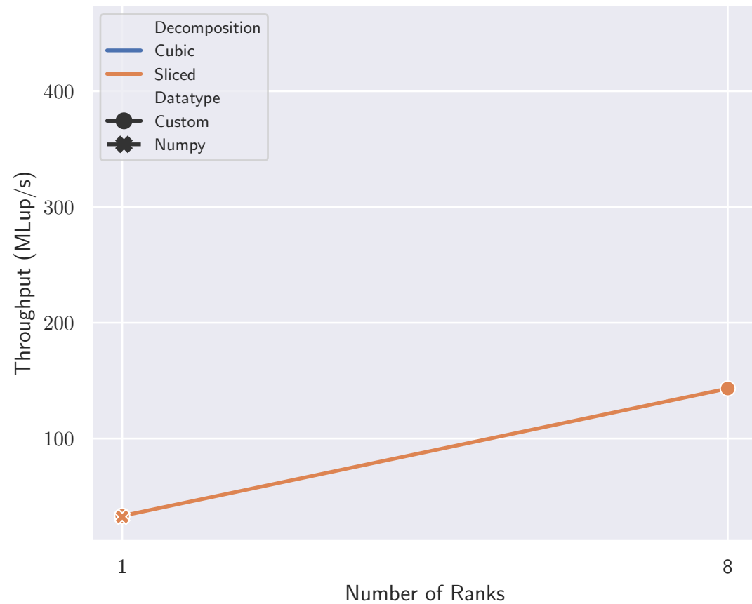
Solver = FMG
