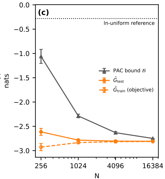
certificate vs truth
