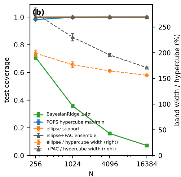
coverage and width vs N
