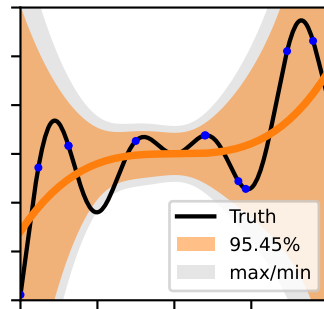
POPS Ellipse
