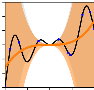
POPS Hypercube
