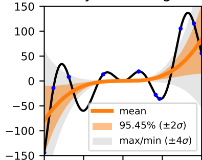
Bayesian Ridge
