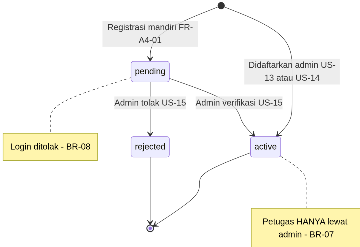
Diagram 3 — 8.1 Siklus hidup akun (FR-A4-01, FR-A4-05..07)
