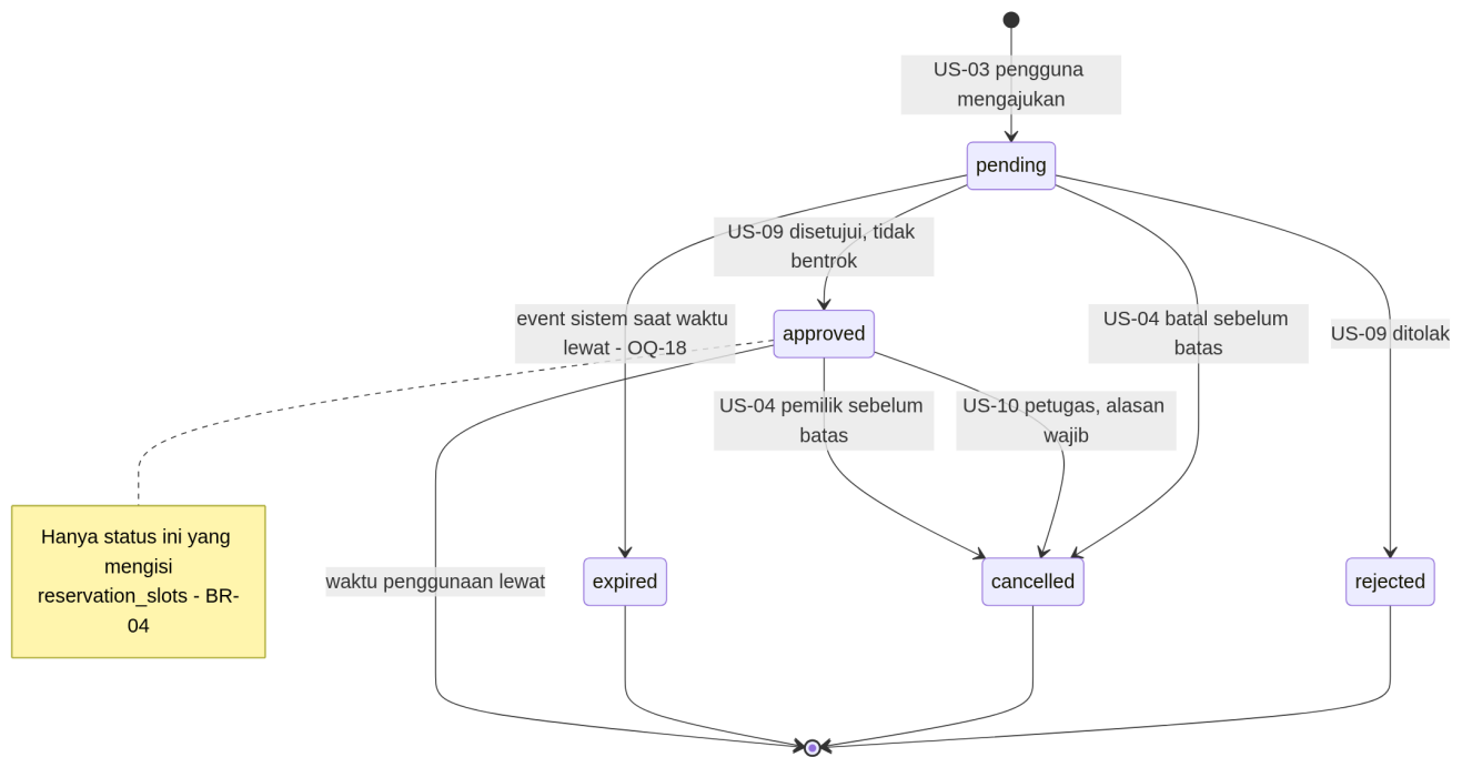
Diagram 3 — 8.1 State machine reservasi
