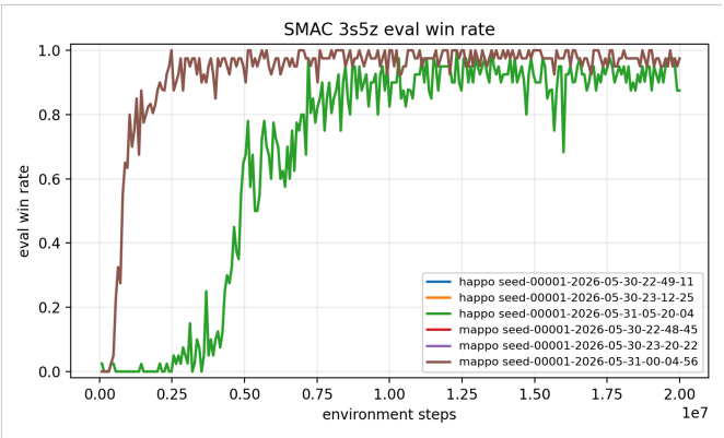
3s5z smoke/pilot/full eval win rate.
