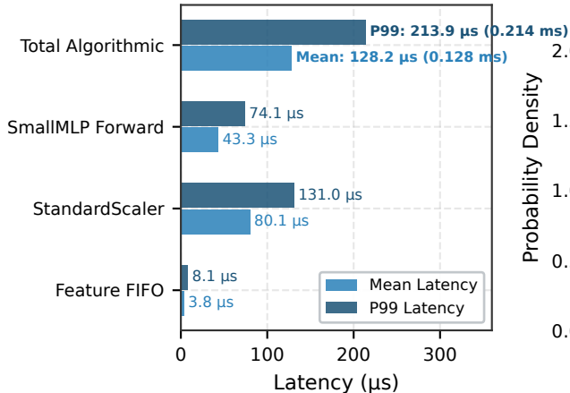
(a) Algorithmic Stage Latency
