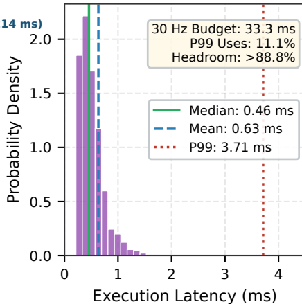
(b) ROS 2 Execution Latency
