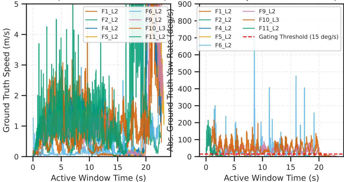
(a) Linear Speed Profiles (50 Hz Resampled) (b) Yaw Rate Dynamics (50 Hz Resampled)
