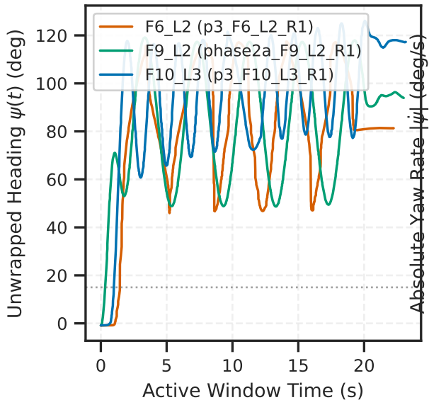
(a) Heading Profiles &amp; Excursions
