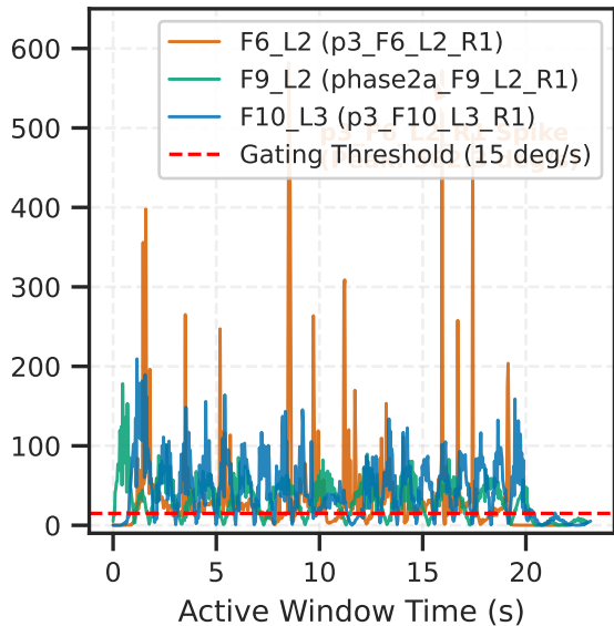
(b) Achieved Yaw-Rate Dynamics
