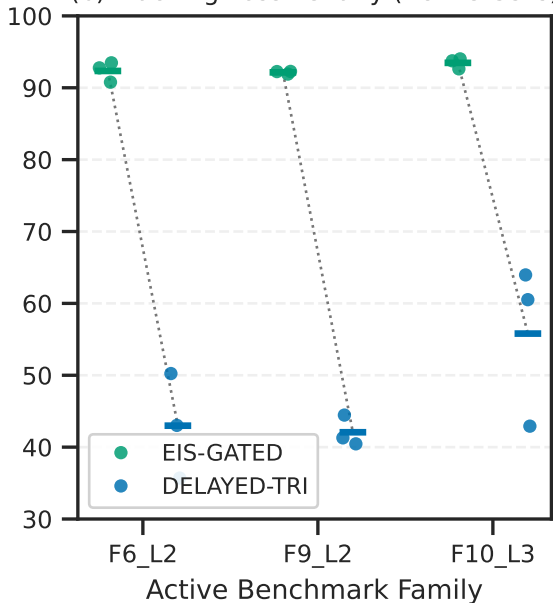
(b) Tracking Loss Penalty (Active Cells)
