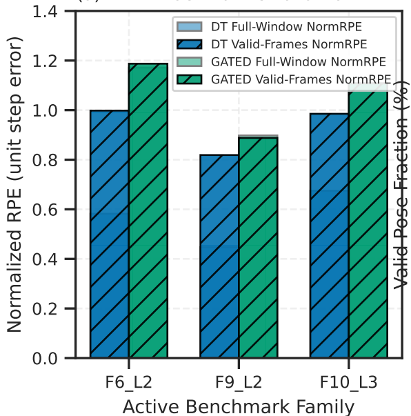
(a) DT Artifact: Full vs Valid NormRPE
