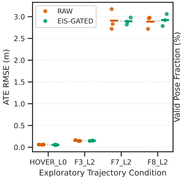
(a) Trajectory Accuracy (ATE RMSE)
