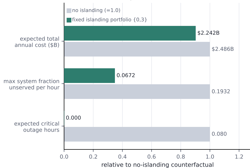
IEEE-39: fixed portfolio, 15 retained scenarios
