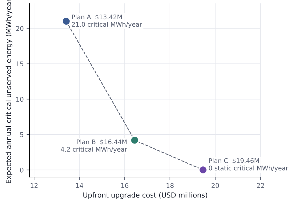
IEEE-33 feeder: cost-resilience Pareto (exact optima)
