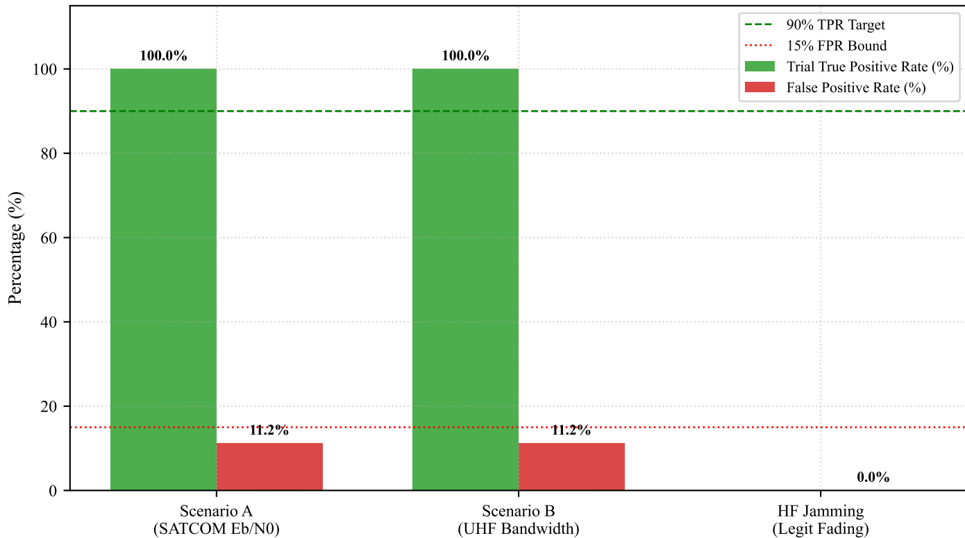
Adversarial Channel-Spoofing Detection Performance Across 30 Seeds
