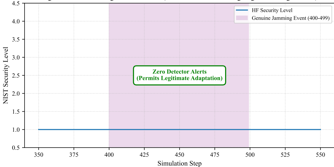
Figure 11: HF Jamming Discrimination (Zero False Alerts During Legitimate Degradation)
