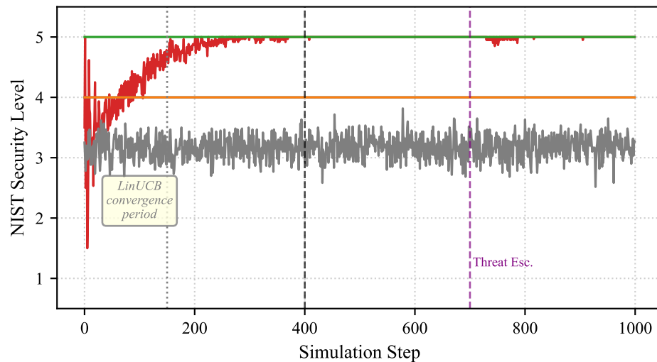
Link Profile: SATCOM
