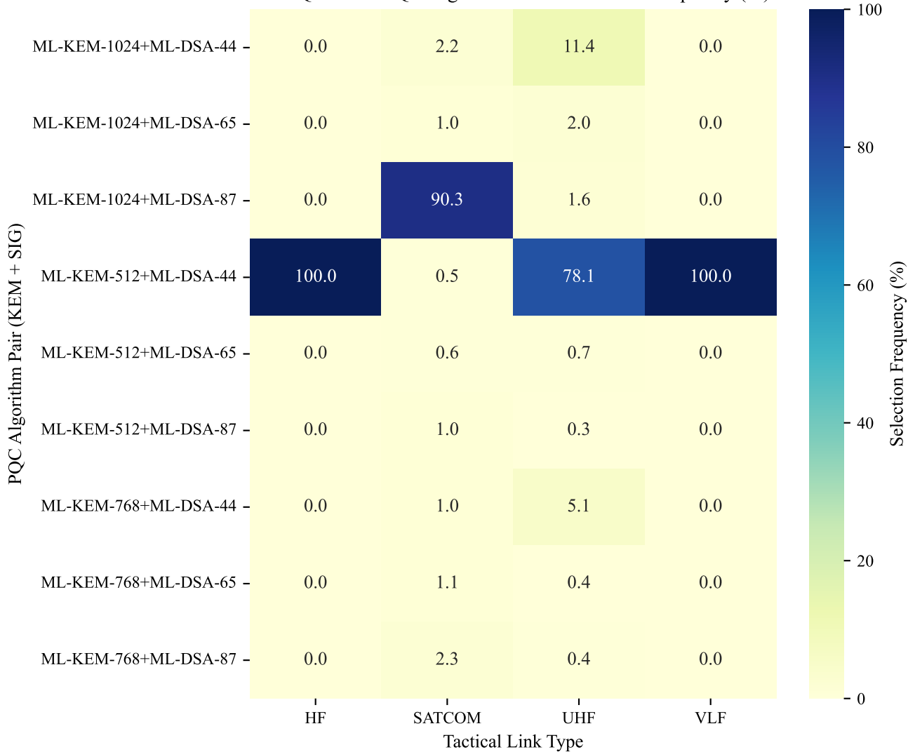
XAPQ-TacNet PQC Algorithm Suite Selection Frequency (%)
