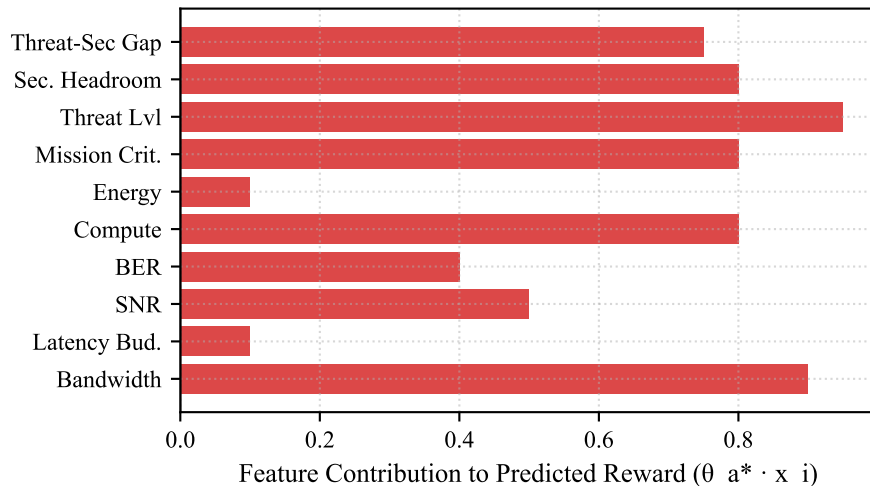
Link: SATCOM
