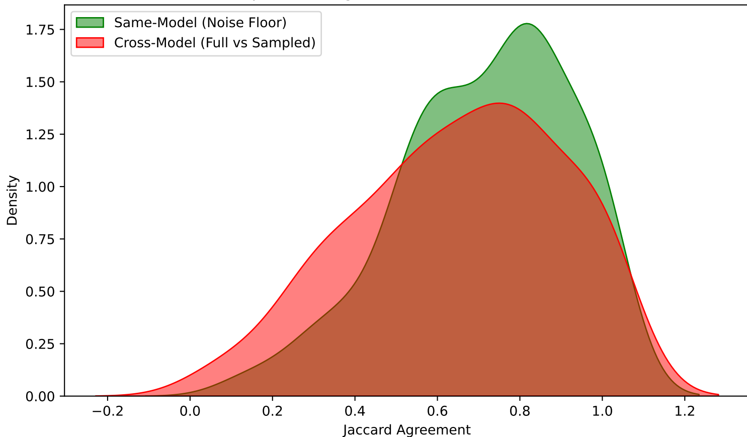
Explanation Agreement Distributions (cora)
