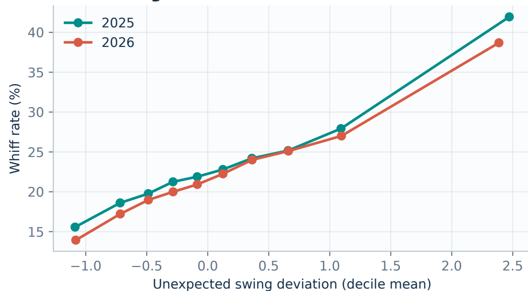
Swing deviation and observed whiff rates
