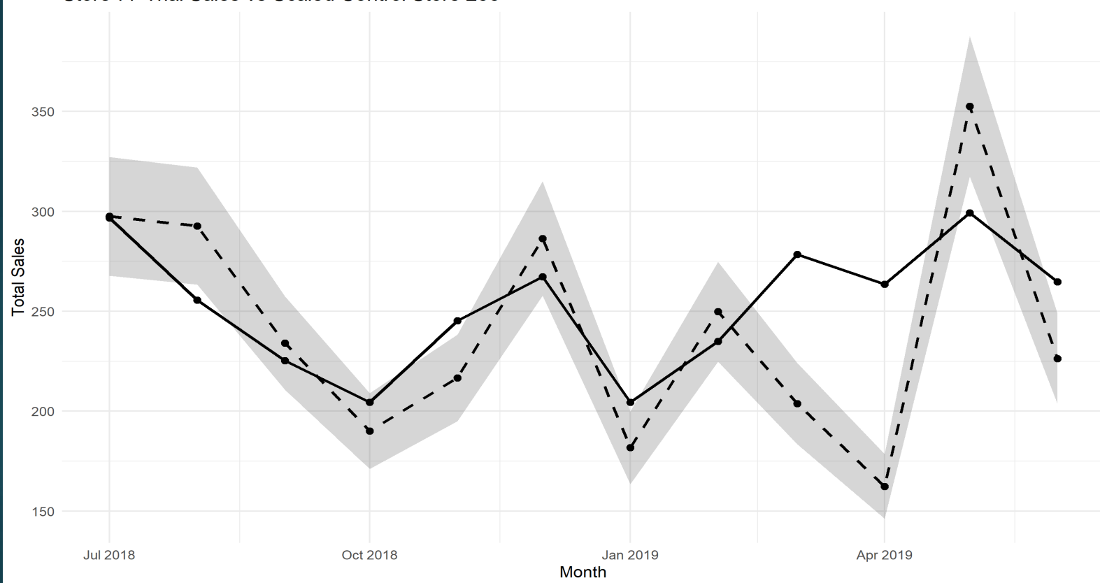
Store 77 Trial Sales vs Scaled Control Store 233
