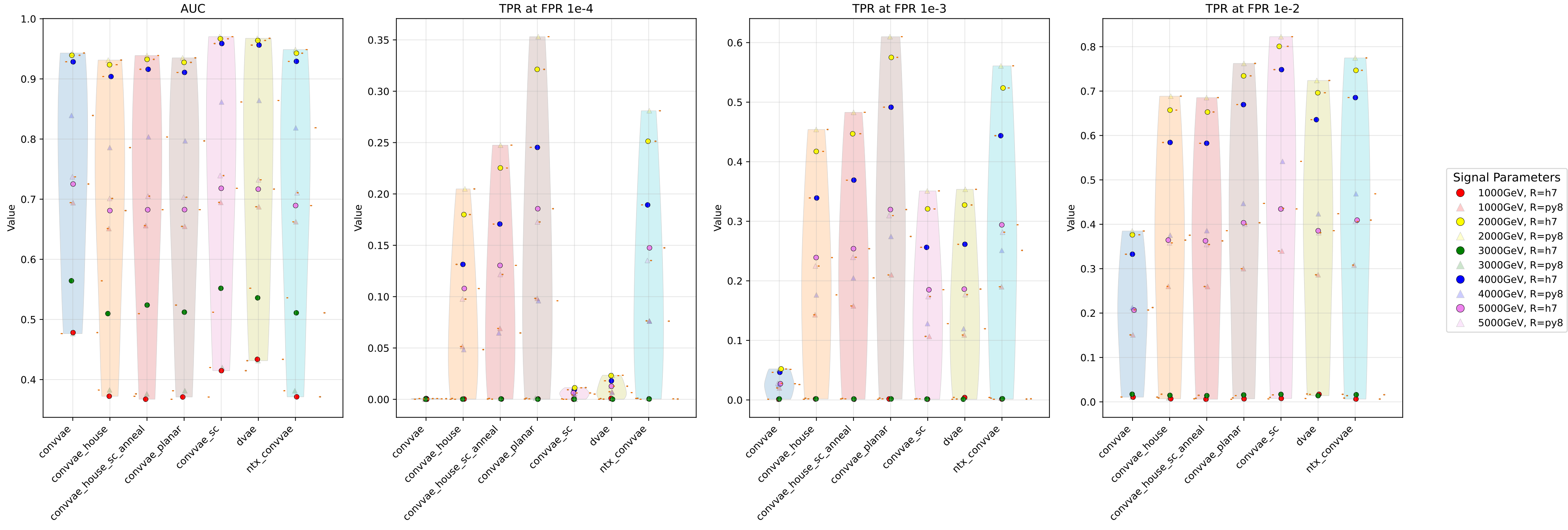
Model Performance by Signal Parameters (Combined) - zprime
