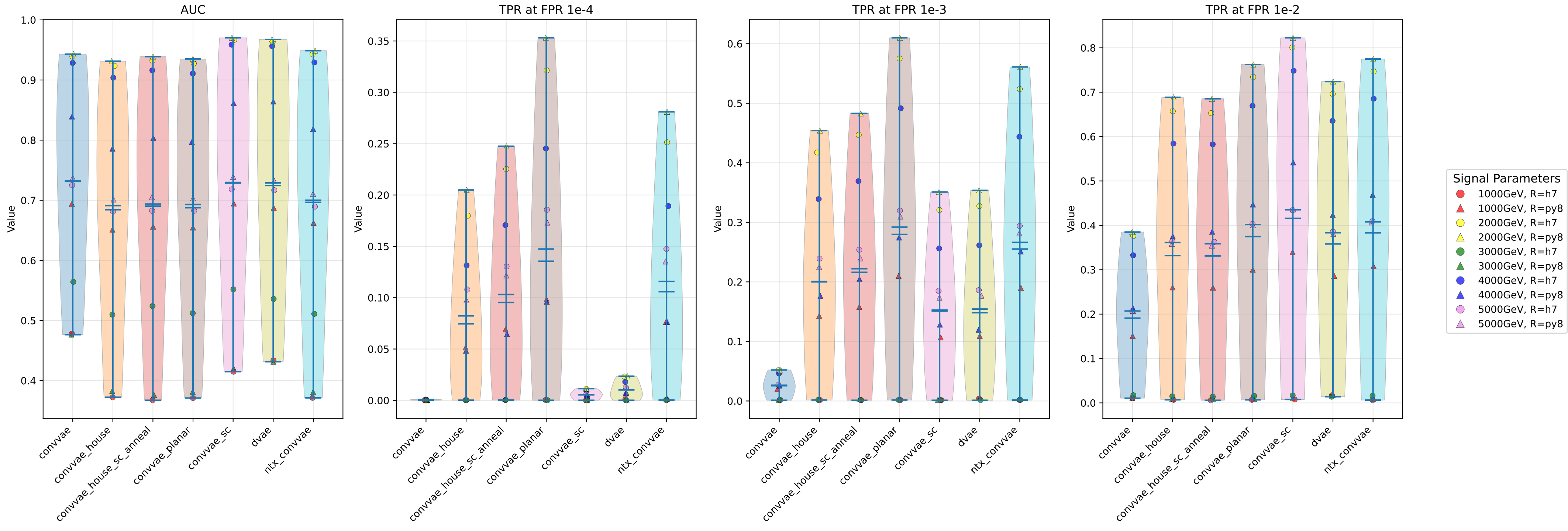
Model Performance by Signal Parameters - zprime
