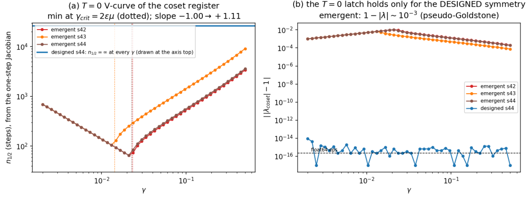
Figure 6: The emergent V-curve un-collapsed, and the negative beside it. (a) The T = 0 half-life against friction per emergent seed from the one-step Jacobian, each with its own \gamma_{crit} = 2\epsilon\mu_{soft} dotted; the designed coset has no finite half-life at any \gamma and is drawn at the axis top. (b) ||\lambda_{coset}|| - 1|| : exact to the float64 floor for the designed symmetry and short by \sim 10^{-3} on every emergent seed, which is the pseudo-Goldstone statement of this section in one panel. Three emergent MLP seeds plus a matched designed control: evidence.
