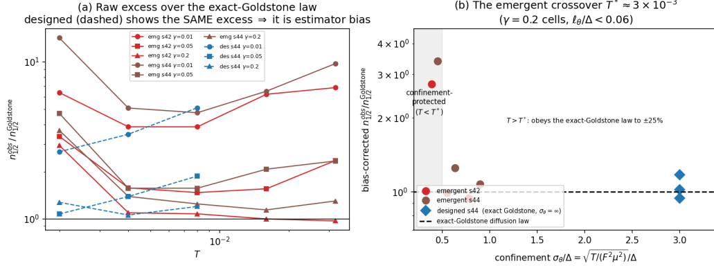
Figure 8: The crossover T^* , and why the raw curve cannot be read directly. (a) The raw excess over the exact-Goldstone law is the same on the matched designed control as on the emergent seeds, so the excess is estimator bias rather than physics. (b) Bias-corrected, the emergent coset joins the exact-Goldstone law above T^* \approx 3 \times 10^{-3} , the shaded band being the confinement-protected cells below it. Multi-seed status, stated plainly: two emergent seeds and one matched designed control, an n < 3 cell. \Delta = 0.5 rad, \ell_{\theta}/\Delta < 0.06 , langevin_noise="fdt", Newtonian kinetic mode: evidence.
