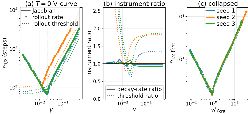
Figure 9: The V-curve measured a second way. (a) T = 0 n_{1/2}(\gamma) per emergent seed on the one-step Jacobian (I-J, lines), the rollout envelope-rate instrument (I-R3, circles) and the rollout first-crossing threshold (I-R1, dotted), at \delta = 0.05 rad. (b) The per- \gamma instrument ratio: the rate ratio sits on 1, the threshold ratio is offset and flat in \gamma above \gamma_{crit} . (c) The same data in collapsed variables. ( Emergent MLP, 3 seeds, dim 4, hidden 64, \varepsilon = 0.05 , float64, T = 0 , pre-registered \Rightarrow evidence. )
