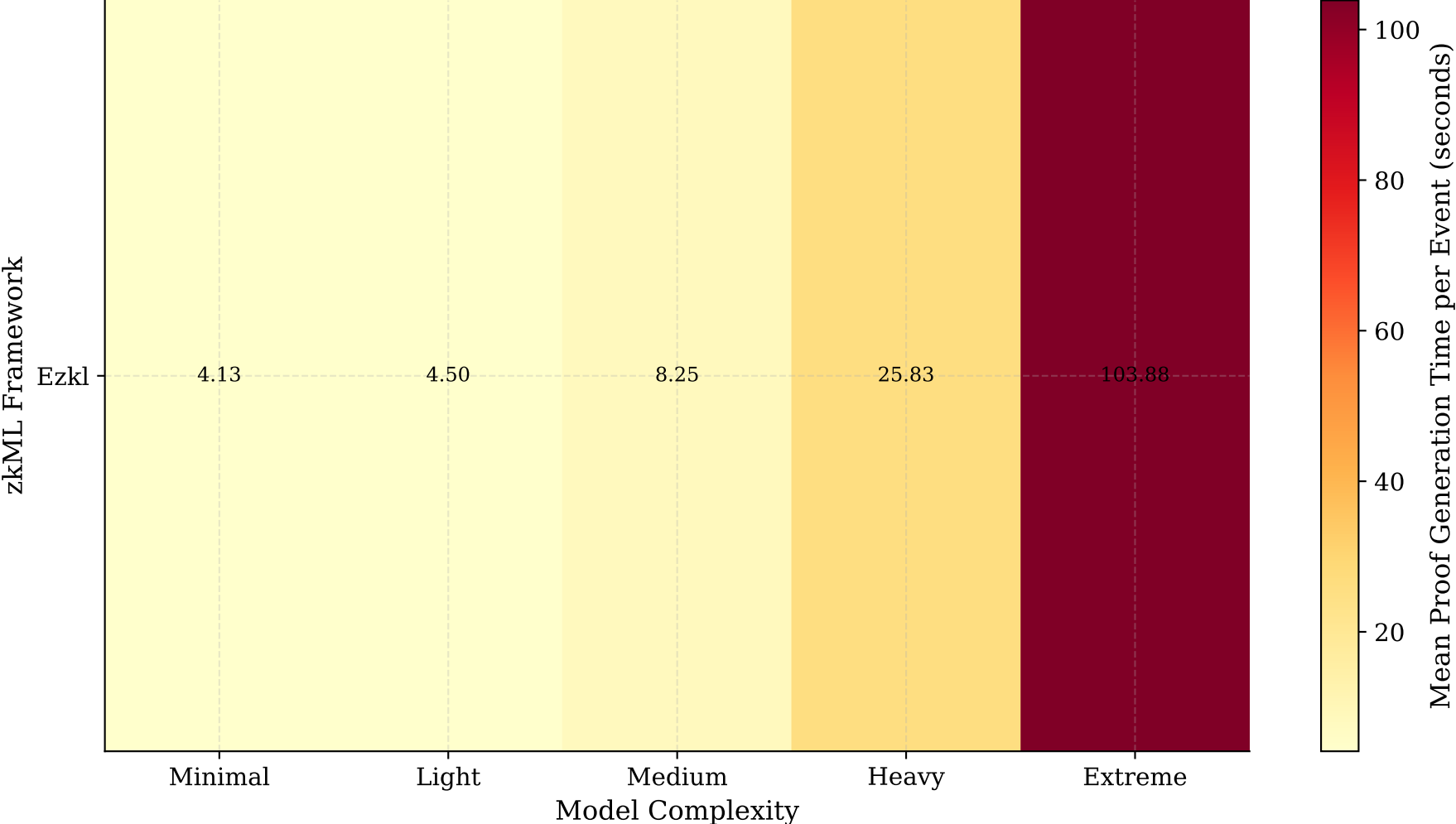
zkML Framework Performance Matrix (Proof Generation Time by Framework and Complexity)
