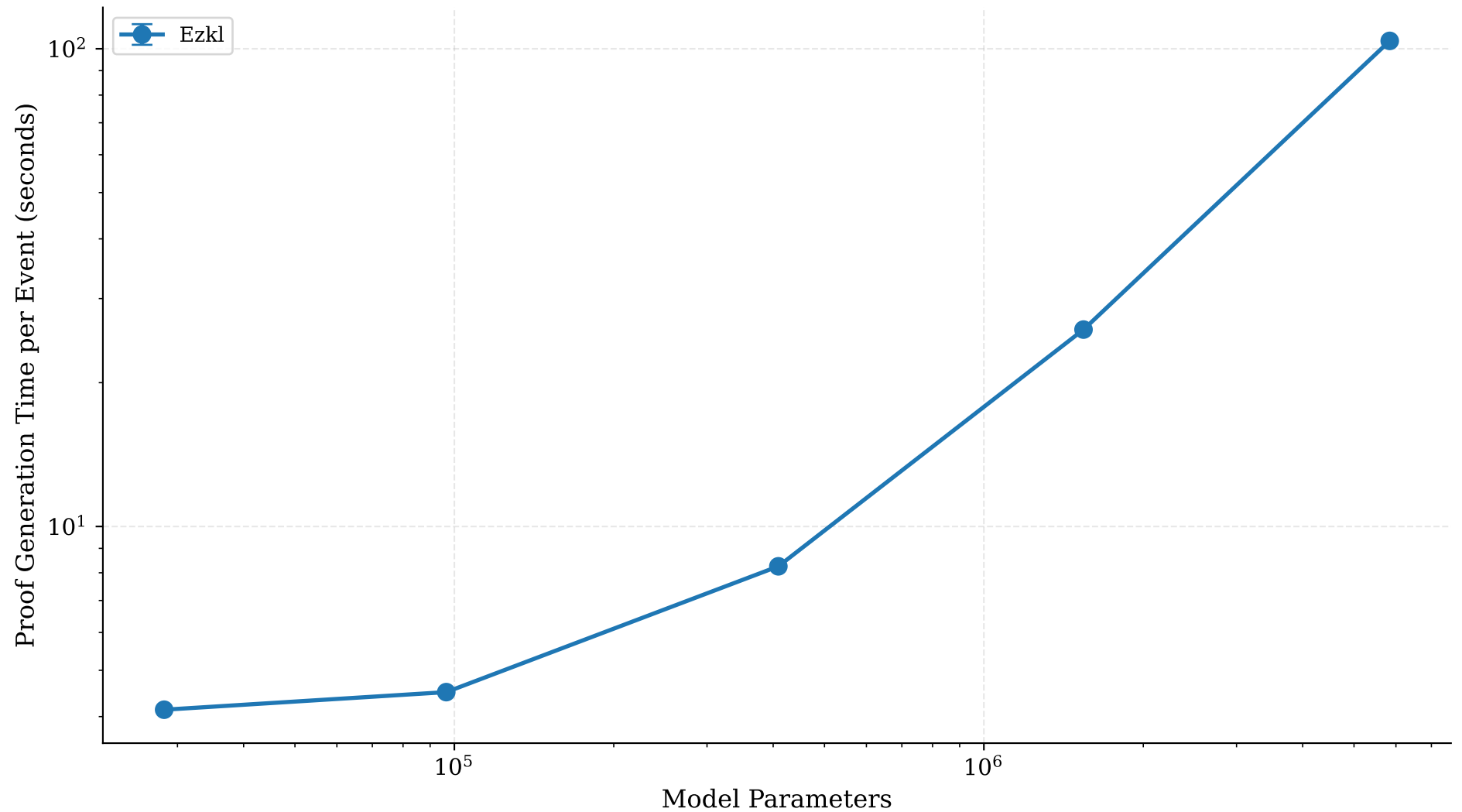
zkML Framework Proof Generation Performance
