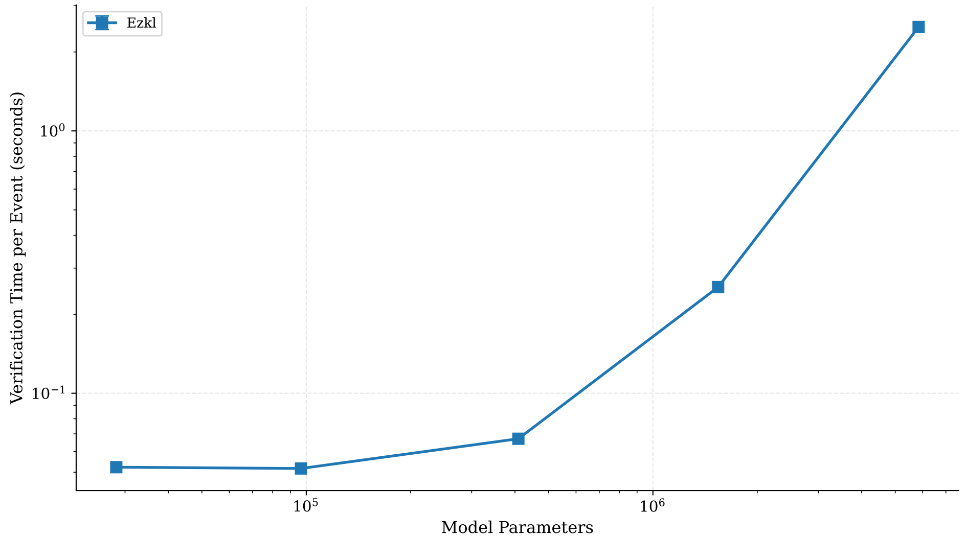
zkML Framework Verification Performance
