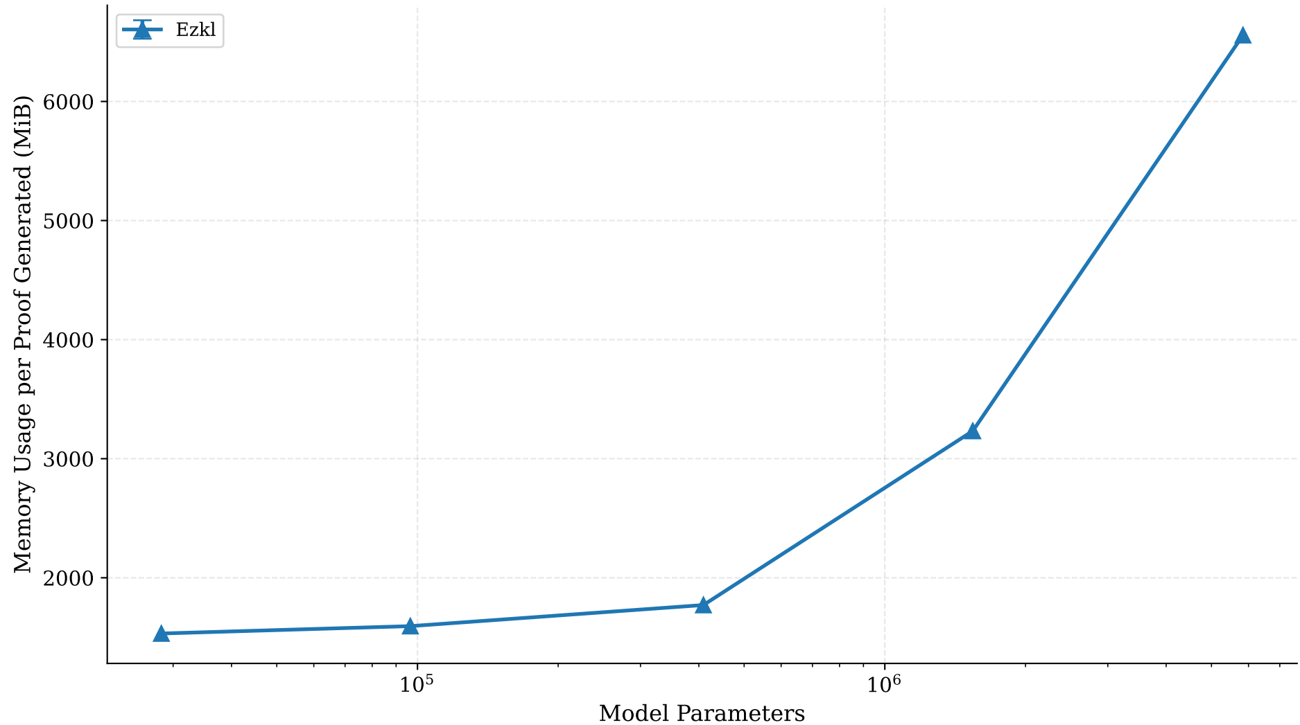
zkML Framework Memory Consumption
