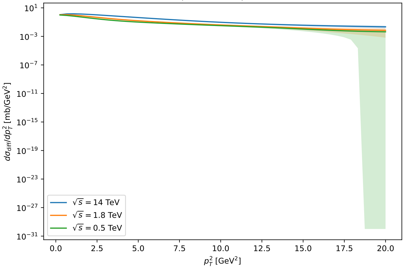
Diffractive charm production - production mechanism
