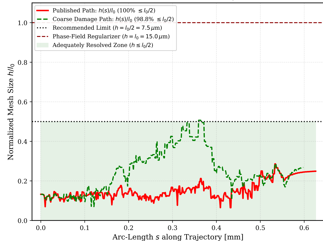
(c) Local Element Resolution h(s)/l_0 along Crack Paths
