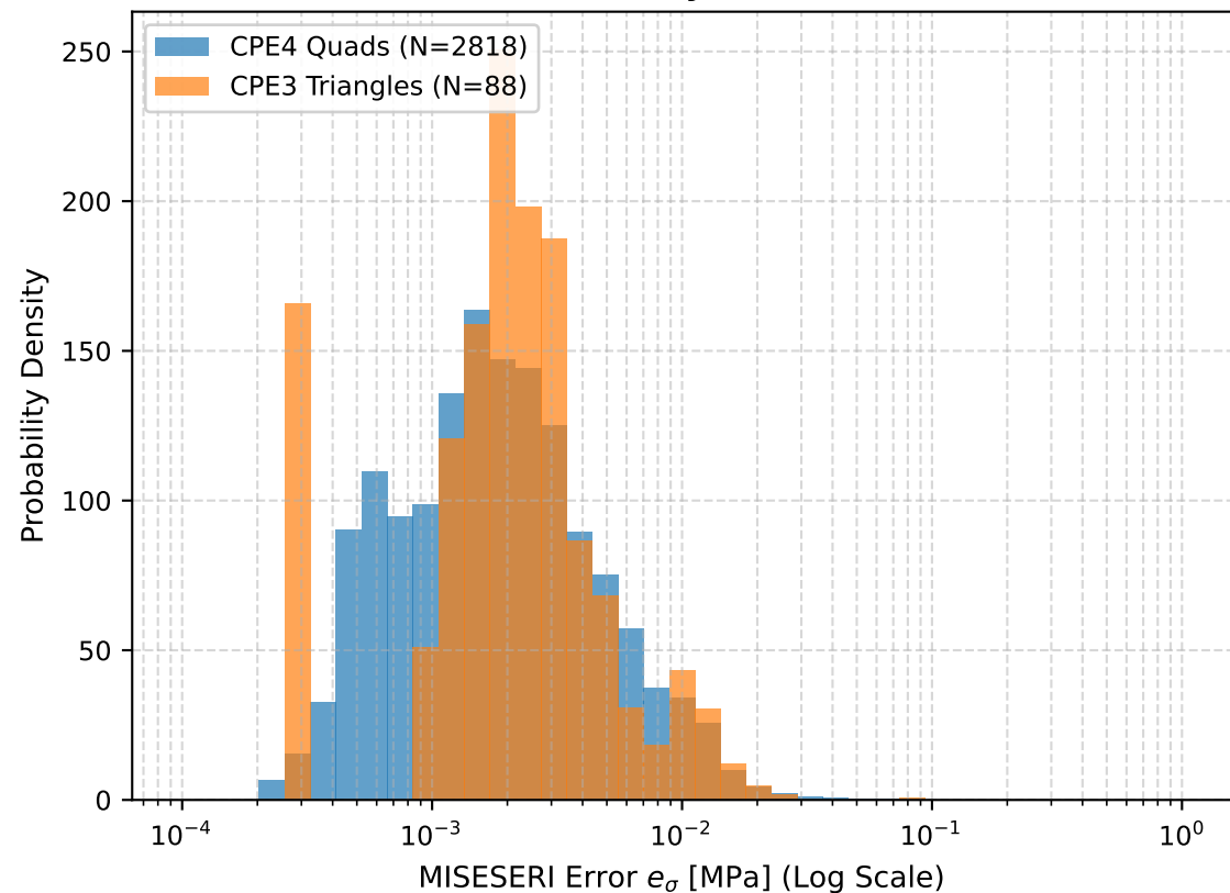
(b) Error Distribution by Element Formulation
