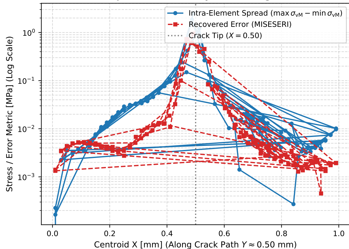
(a) Stress Spread vs Recovery Error along Crack Plane
