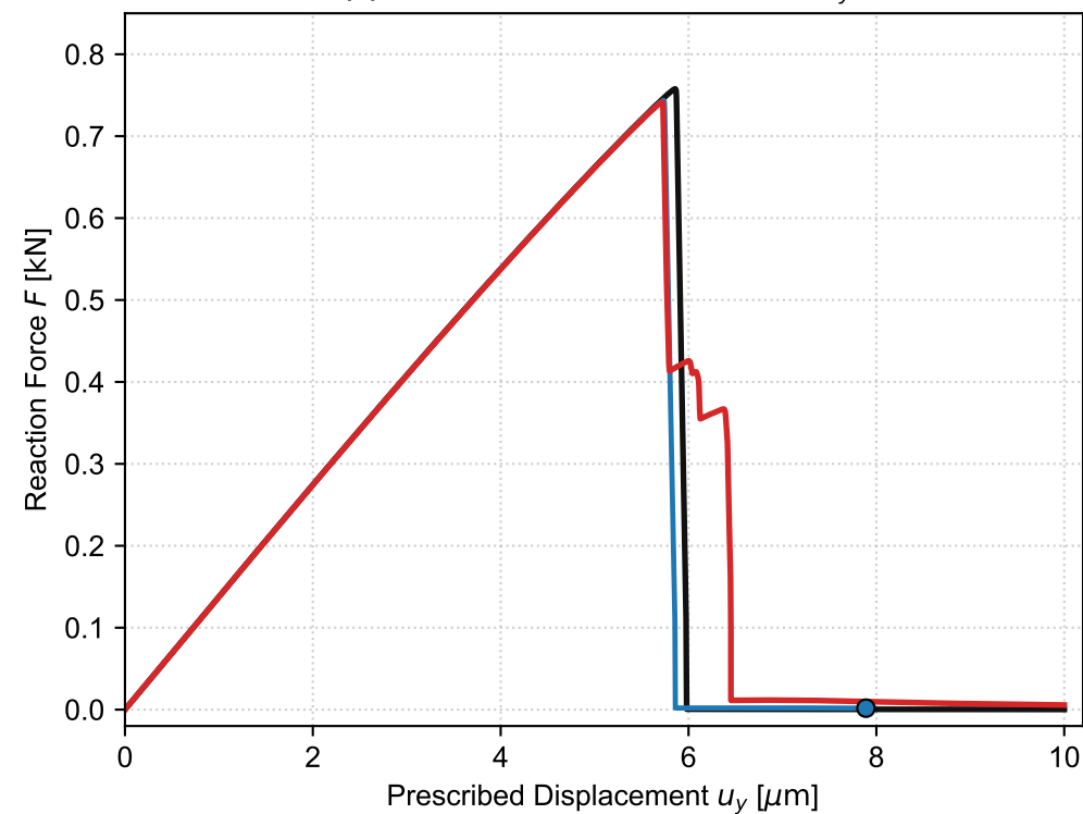
(a) Structural Reaction Force F(u_y)
