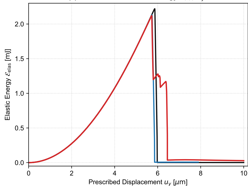
(c) Stored Elastic Strain Energy \mathcal{E}_{\text{elas}}(u_y)
