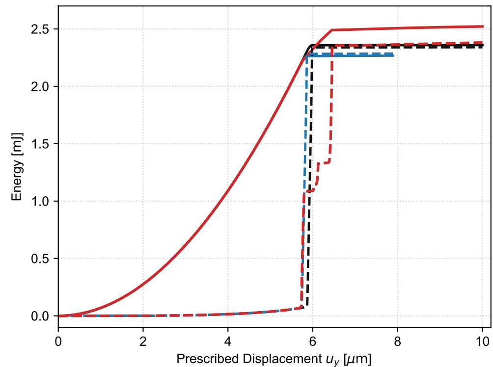
(b) External Work W_{\text{ext}} & Fracture Surface Functional \mathcal{E}_{\text{frac}}
