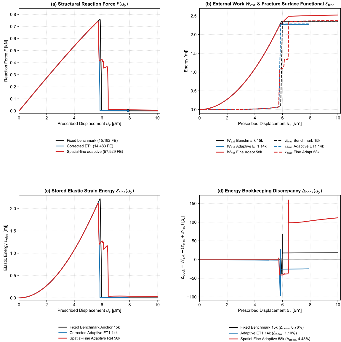
Figure 4: Three-case Gate-6B global synthesis: (a) reaction force; (b) external work and phase-field fracture-energy functional; (c) stored elastic energy; and (d) energy-bookkeeping difference. ET1 is censored at u = 0.007889 mm after a 98.5% load drop; no values are forward-filled.
