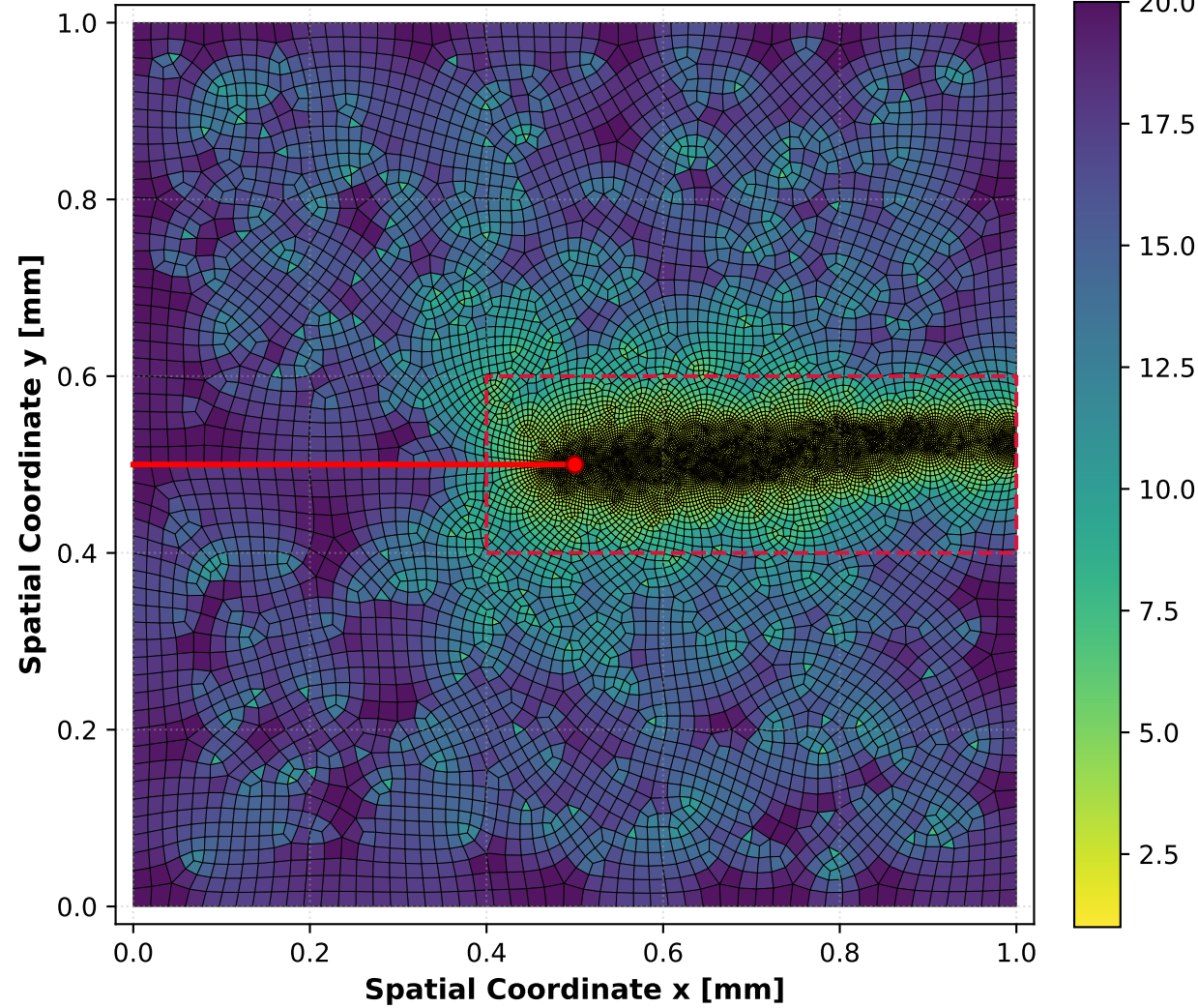
Full Specimen Mesh (errorTarget = 1.0%)
