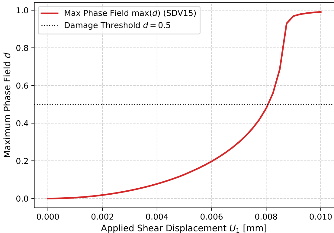
Mode-II Phase-Field Damage Evolution ( H_0 )
