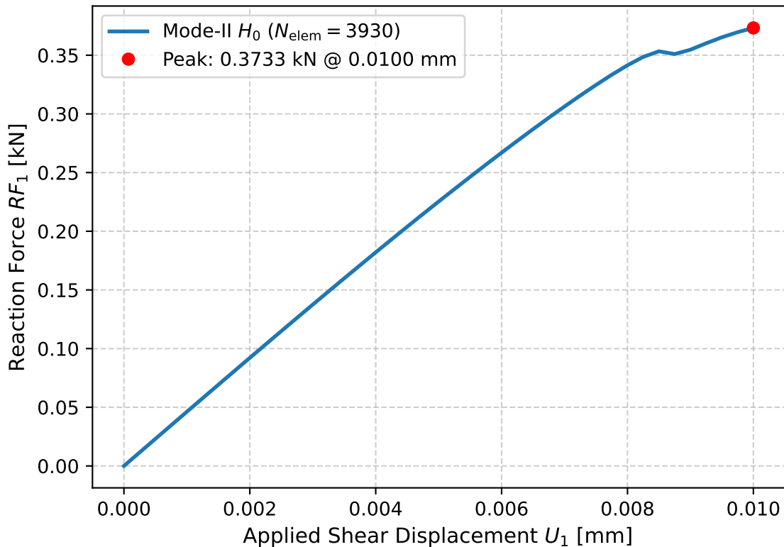
Mode-II Pure Shear Baseline Response ( H_0 , Endpoint-Corrected)
