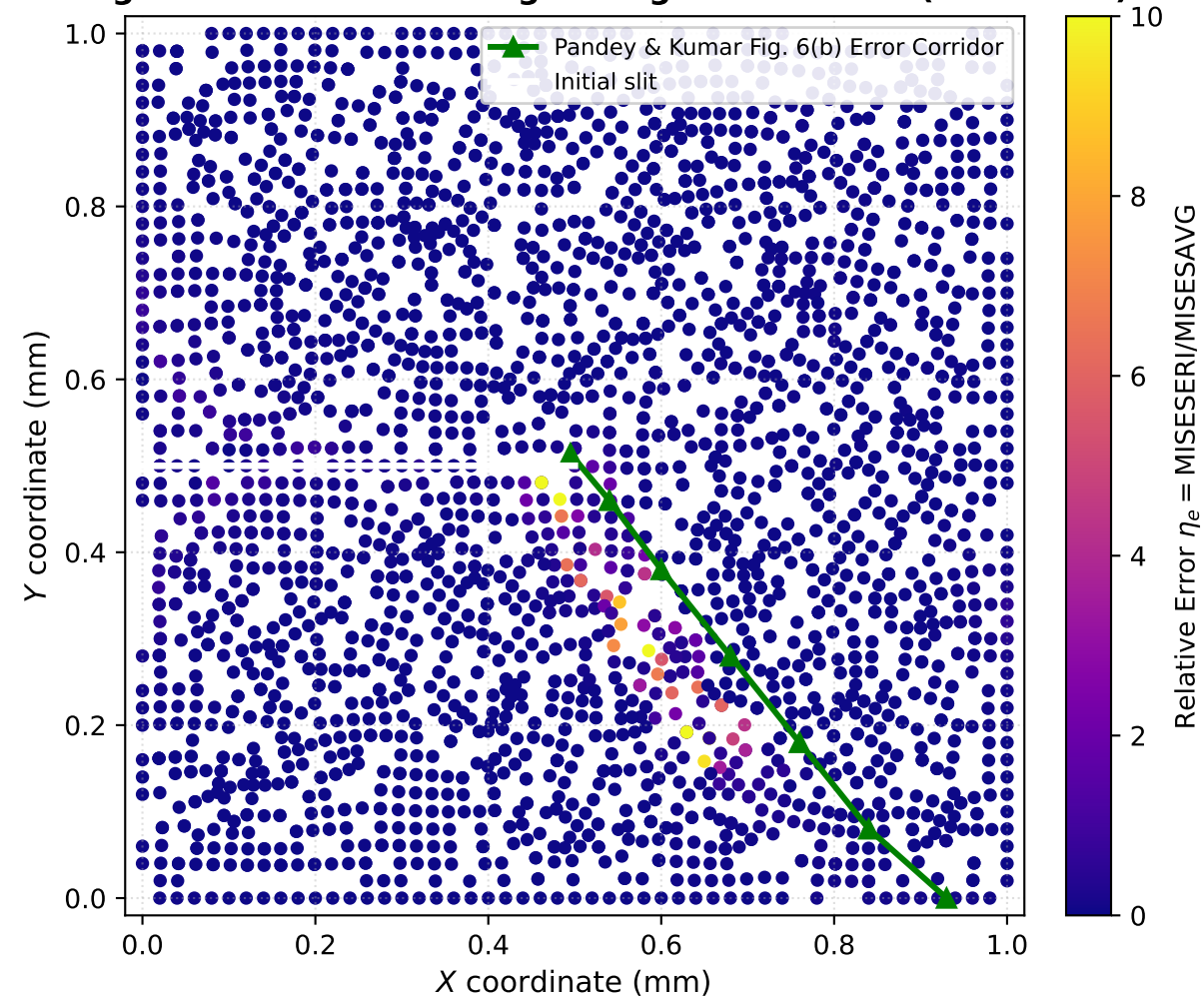
(c) Corrected Stress Discretization Error Field: Emergence of Downward-Right Diagonal Corridor ( \theta = -34.1^\circ )
