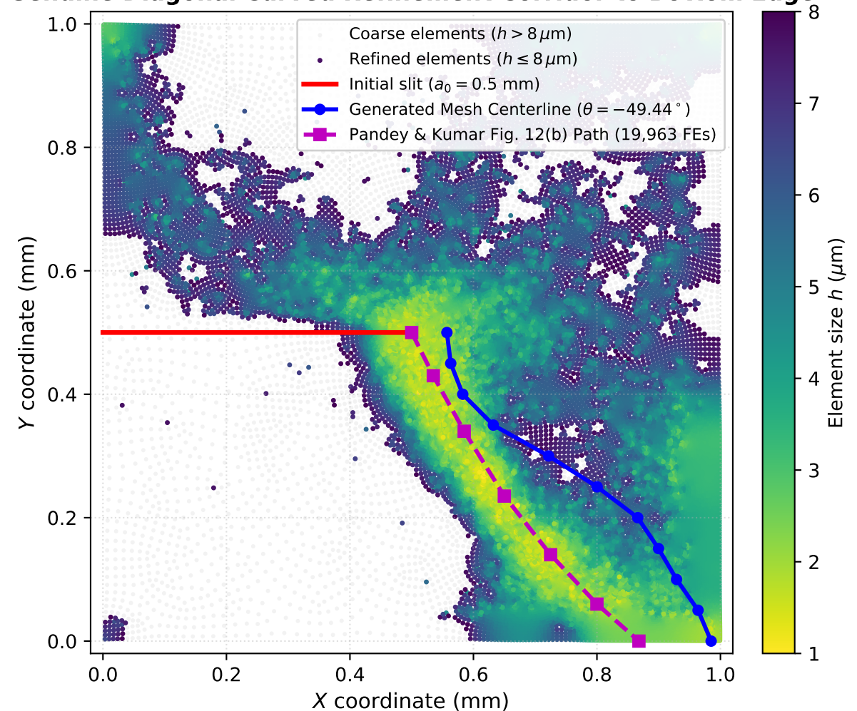
(d) Corrected Native Adaptive Mesh (`ET_2PCT`, 37,575 FEs): Genuine Diagonal Curved Refinement Corridor to Bottom Edge
