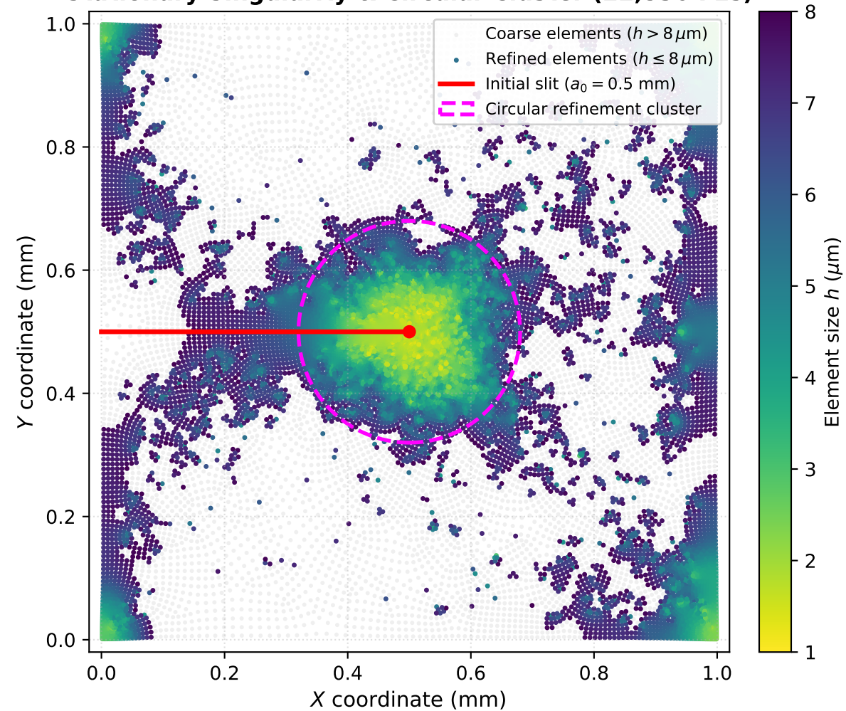
(a) Original Pre-Analysis (Job 1410790, d \equiv 0 ): Stationary Singularity & Circular Cluster (22,530 FEs)
