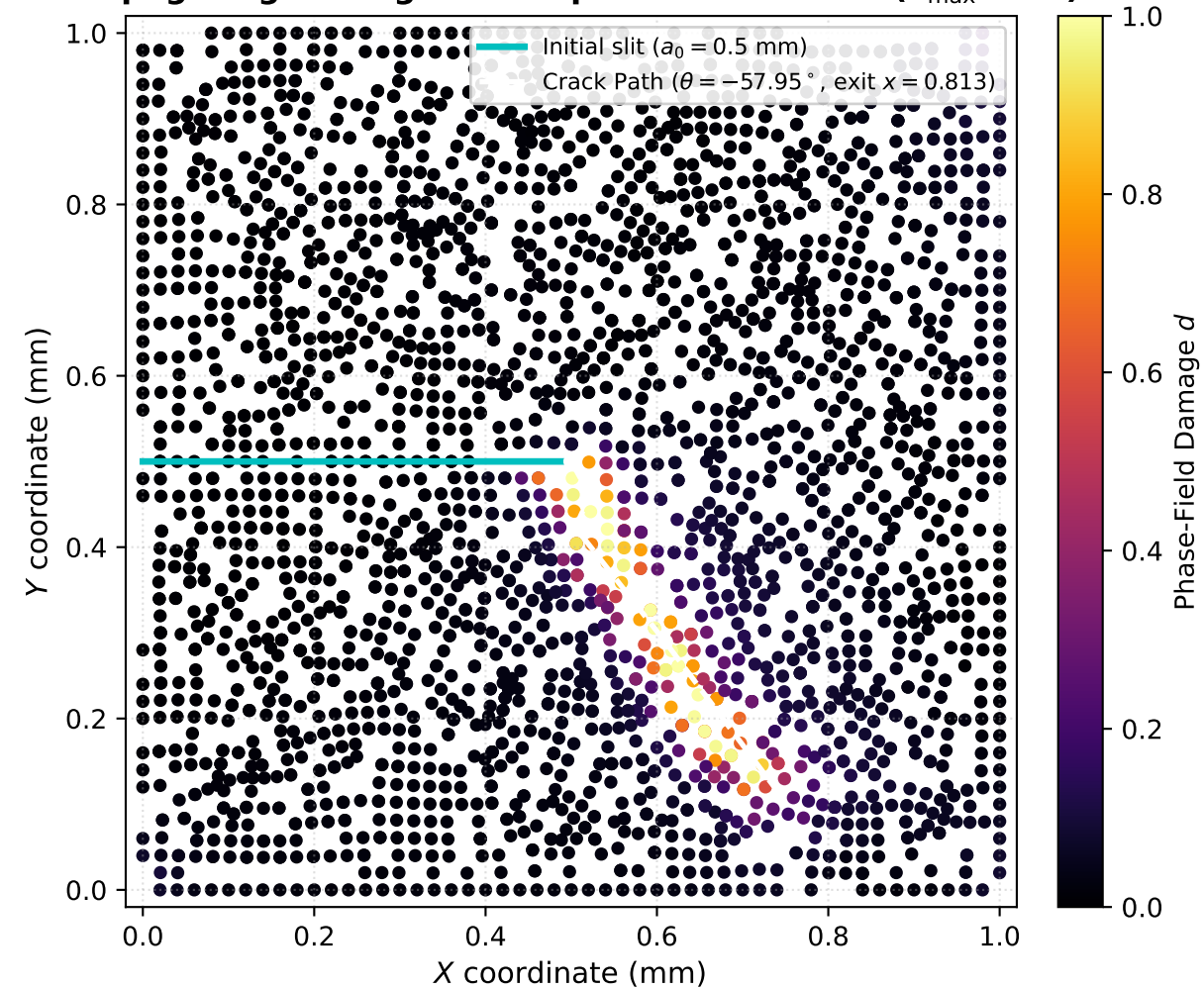
(b) Corrected Pre-Analysis (Job 1411104, RHS Repaired): Propagating Damage & Oblique Mode-II Crack ( d_{\text{max}} = 1.0 )
