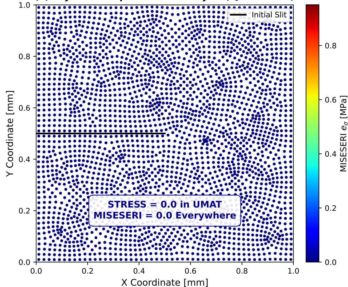
(a) Layered Companion Pre-Analysis ( e_\sigma \equiv 0.0 MPa)
