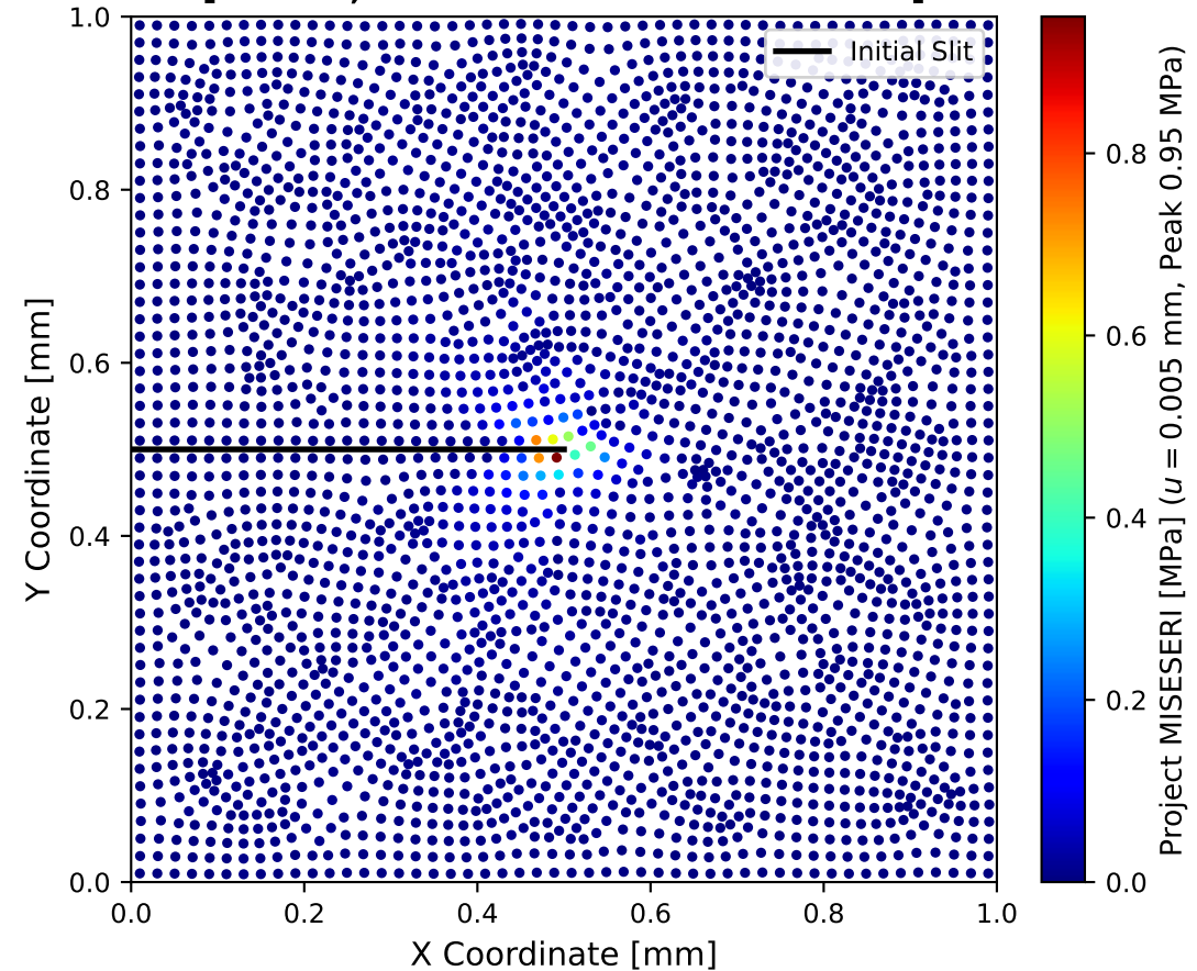
(b) Project Pre-Analysis Control [Exact 2,906-Element Continuum Solve]
