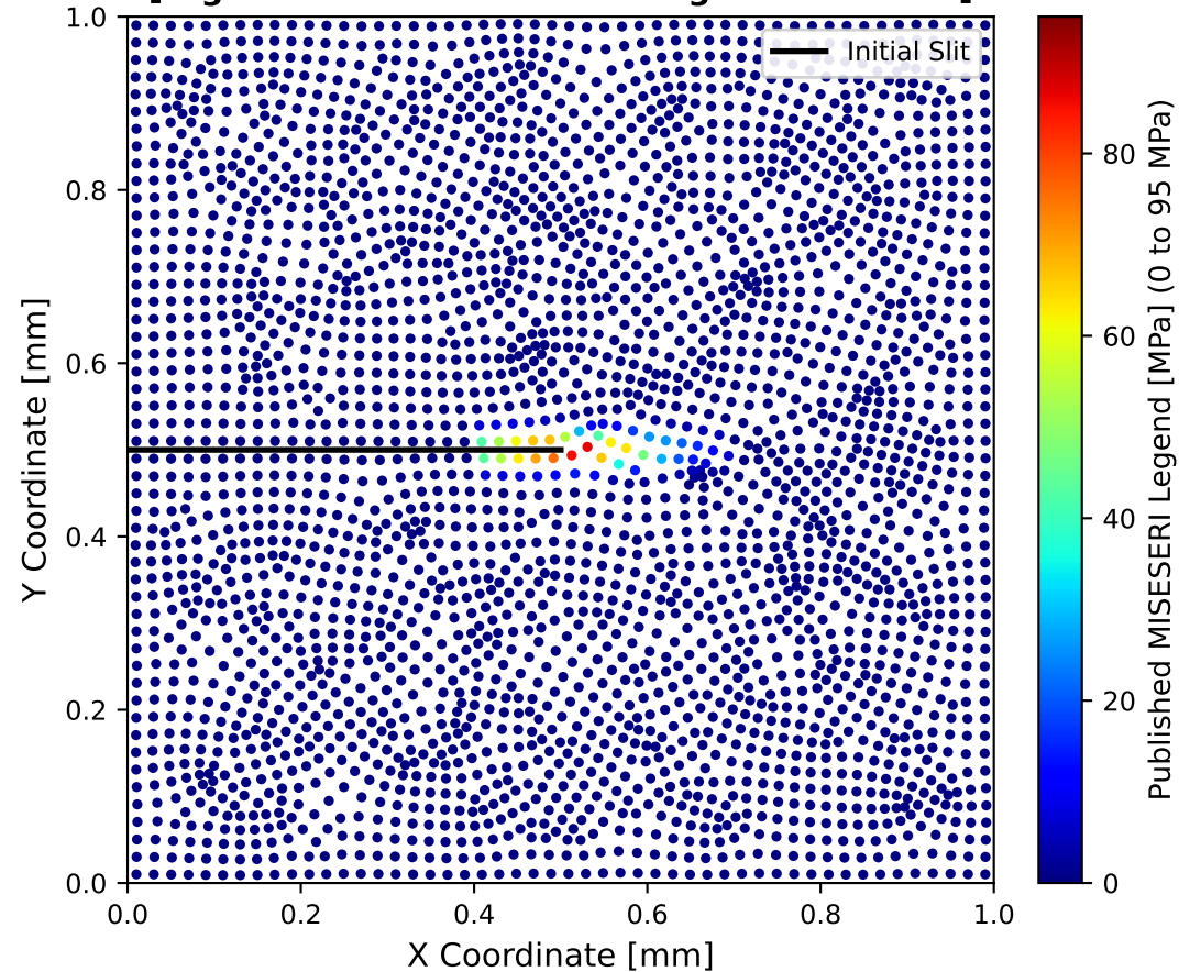
(a) Pandey & Kumar (2025) Fig. 6(a) [Digitized Visual Evidence: Legend 0-95 MPa]
