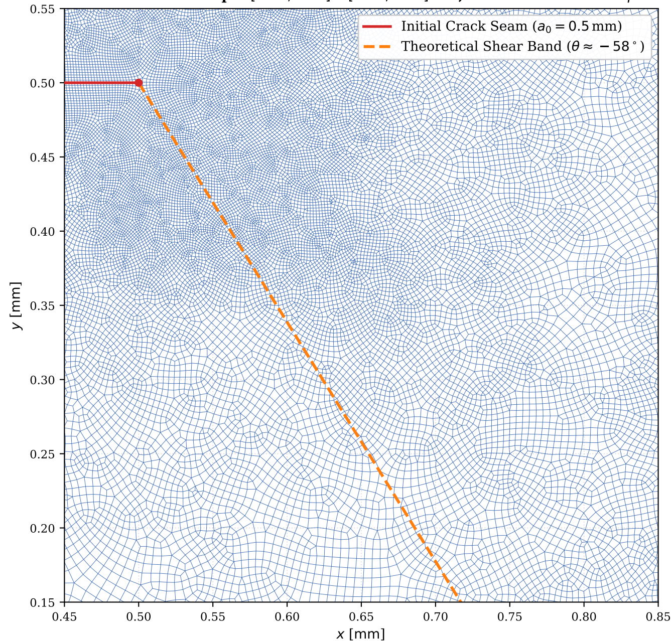
Mode-II Shear Propagation Corridor: Step-2 errorTarget = 1.0% Refinement Envelope: [0.45, 0.85] \times [0.15, 0.55] mm, 99.3% FEs with h \leq 8 \mu\text{m}
