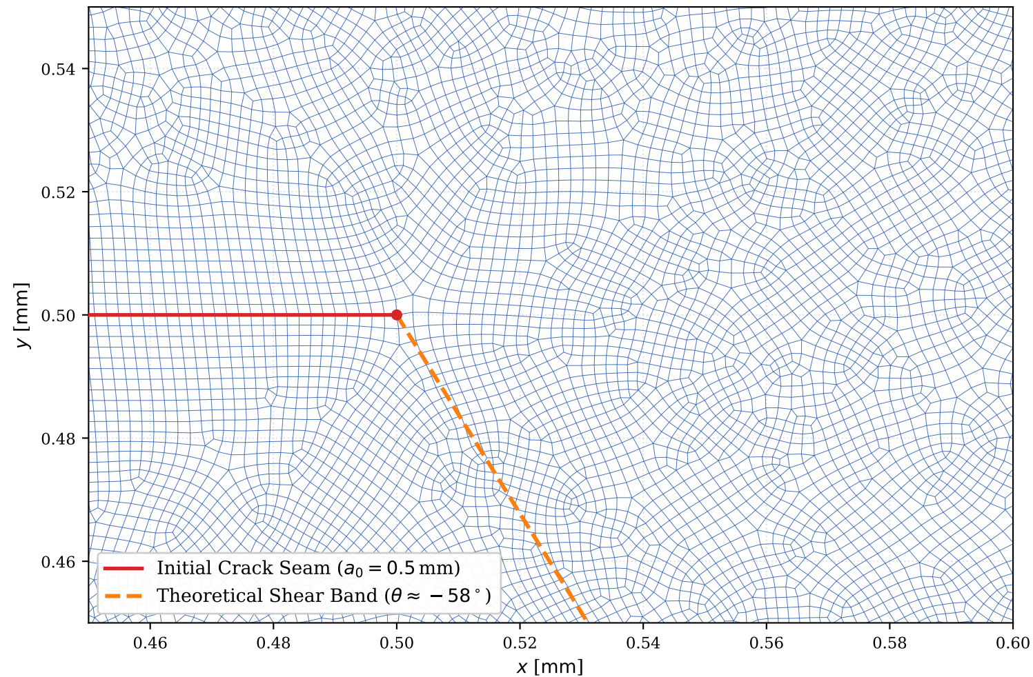
Mode-II Crack-Tip Singularity Zoom: Step-2 errorTarget = 1.0% Dense Singularity Core: h_{\min} = 0.60\ \mu\text{m} ( h/l_0 = 0.080 \ll 1 ), Domain [0.45, 0.60] \times [0.45, 0.55]\text{ mm}
