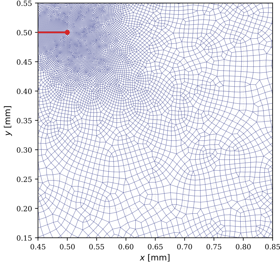
Step-2 ( u_x = 20\text{ }\mu\text{m} , ET = 2.0%) Refinement Corridor & Shear Fan
