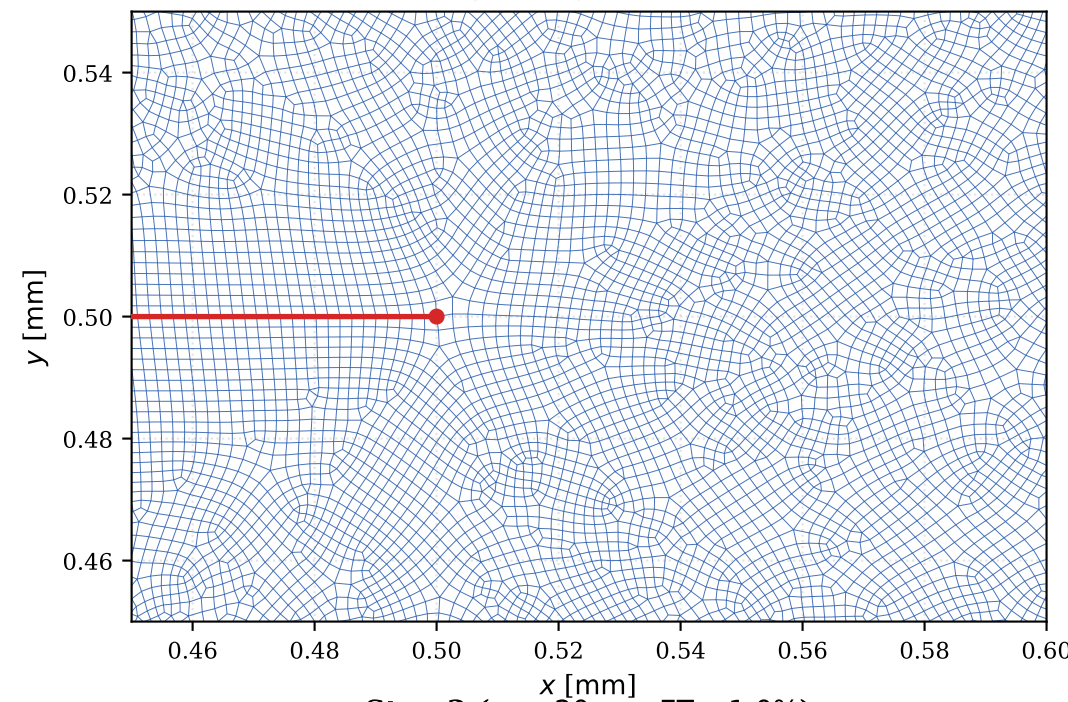
Step-2 ( u_x = 20\text{ }\mu\text{m} , ET = 1.0%) Extended Corridor (+259% FE Density)
