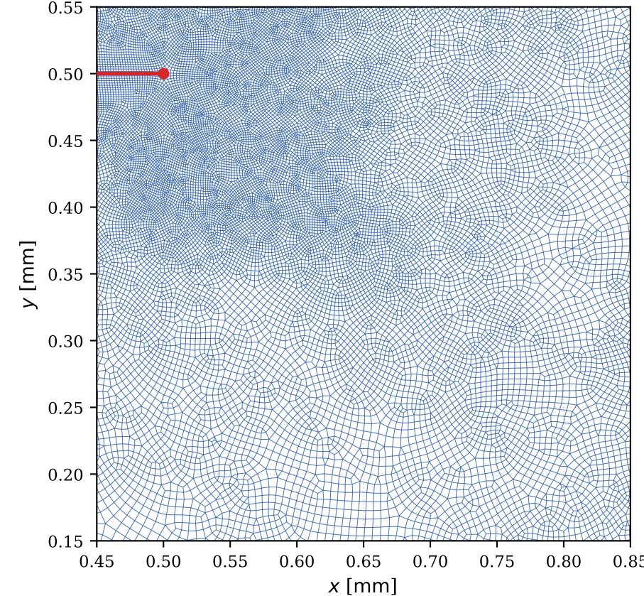
Step-2 ( u_x = 20\text{ }\mu\text{m} , ET = 1.0%) Extended Corridor (+259% FE Density)
