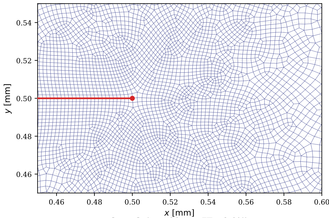
Step-2 ( u_x = 20\text{ }\mu\text{m} , ET = 2.0%) Refinement Corridor & Shear Fan
