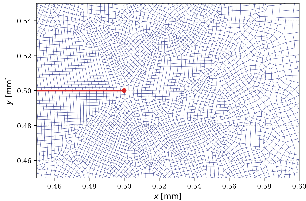
Step-1 ( u_x = 10\text{ }\mu\text{m} , ET = 2.0%) Refinement Corridor & Shear Fan
