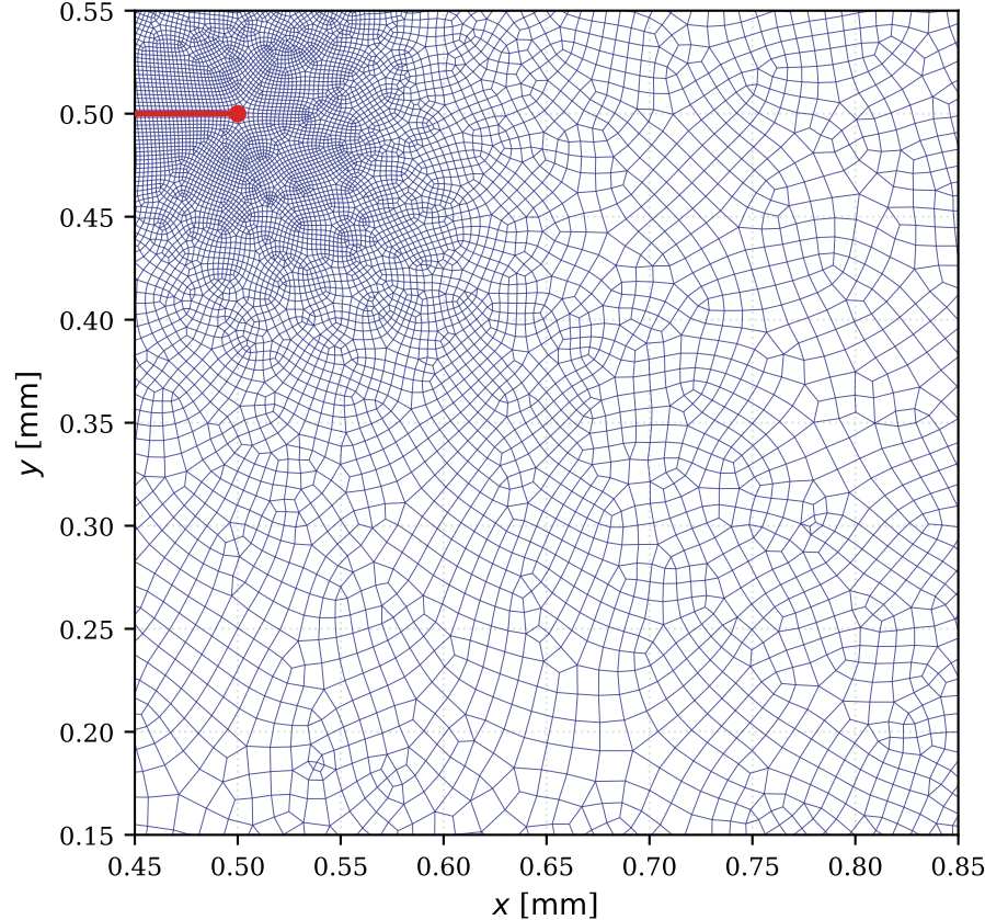
Step-1 ( u_x = 10\text{ }\mu\text{m} , ET = 2.0%) Refinement Corridor & Shear Fan
