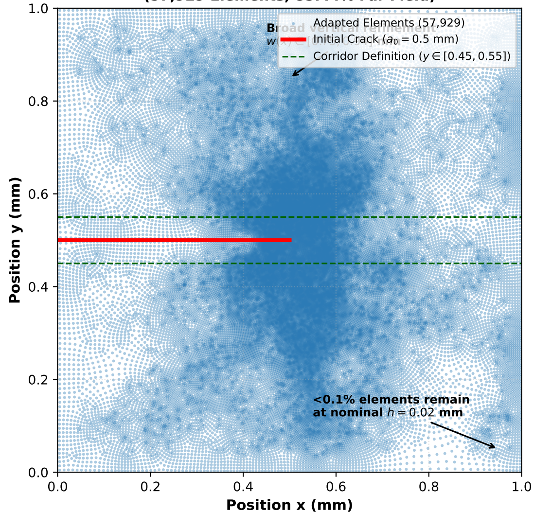
(b) Literal Native 1% Adapted Mesh (57,929 Elements, 85.44% Far Field)
