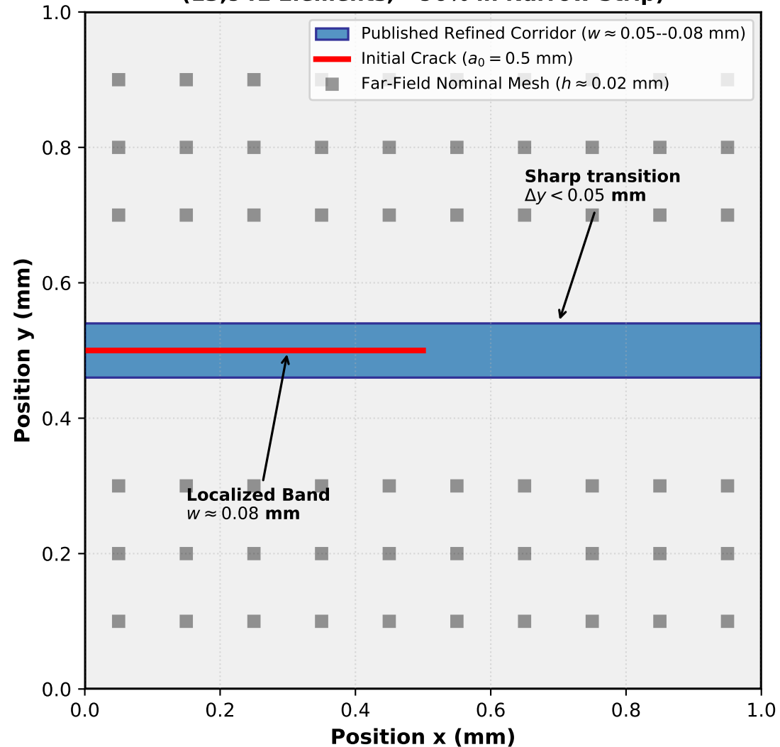
(a) Pandey & Kumar (2025) Target Morphology (13,941 Elements, >90% in Narrow Strip)
